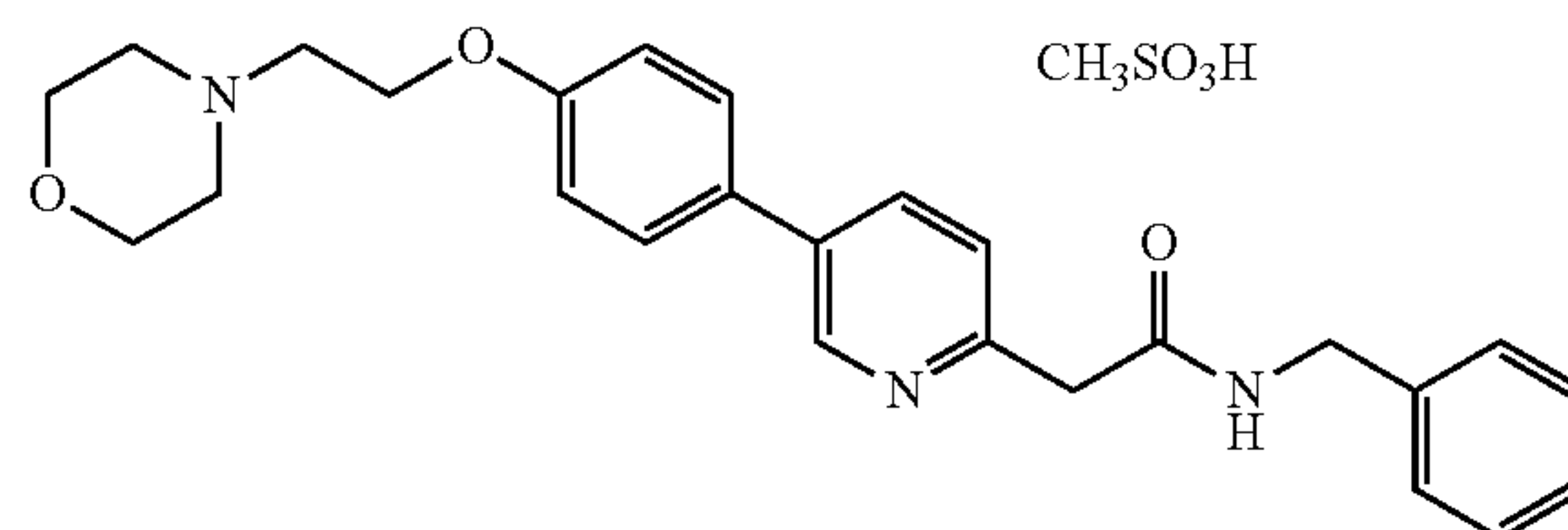
KX2-391 MSA
