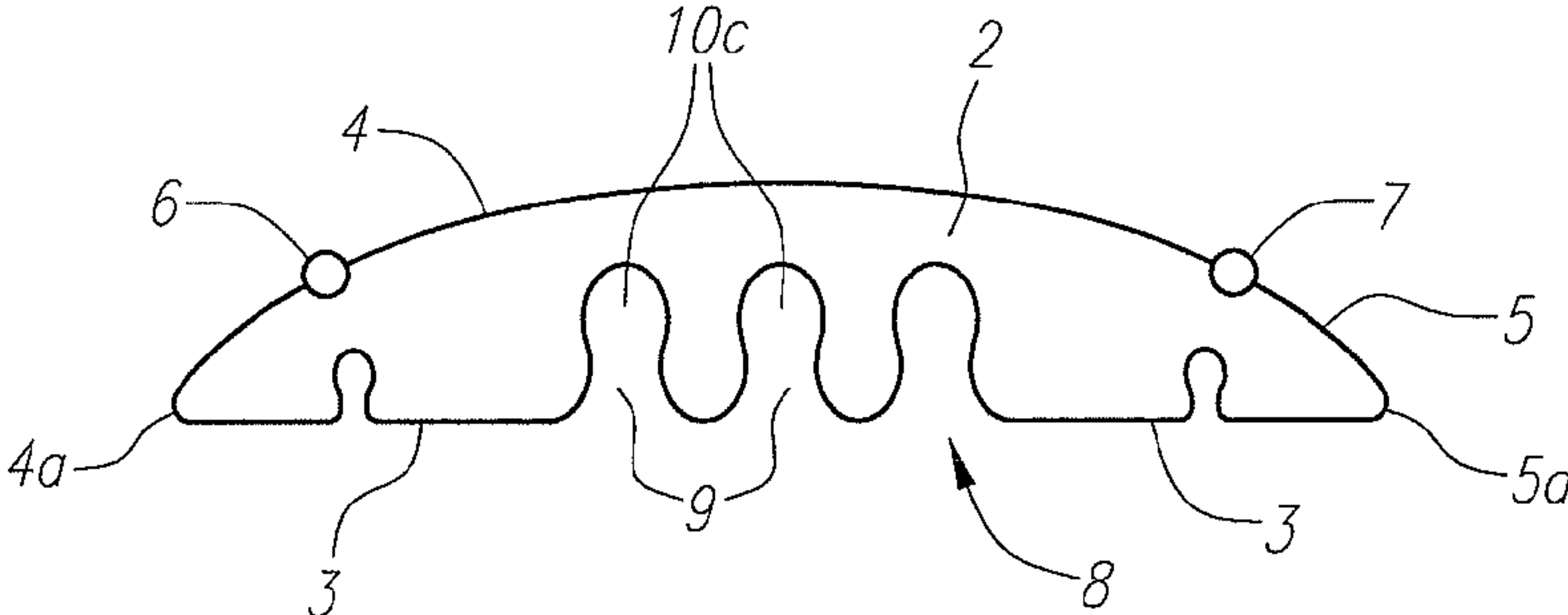
FIG. 3 (PRIOR ART)
