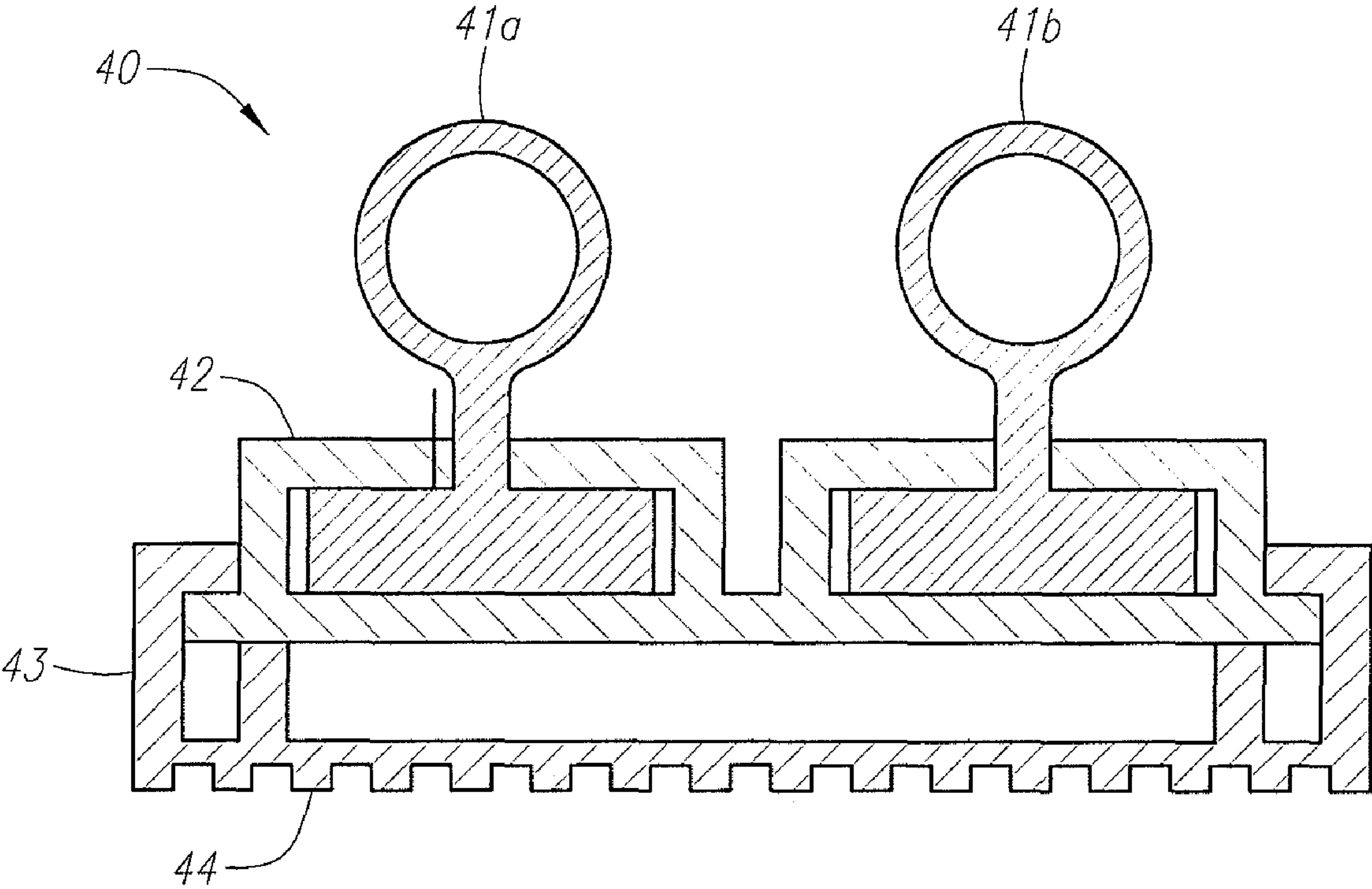
FIG. 4 (PRIOR ART)
