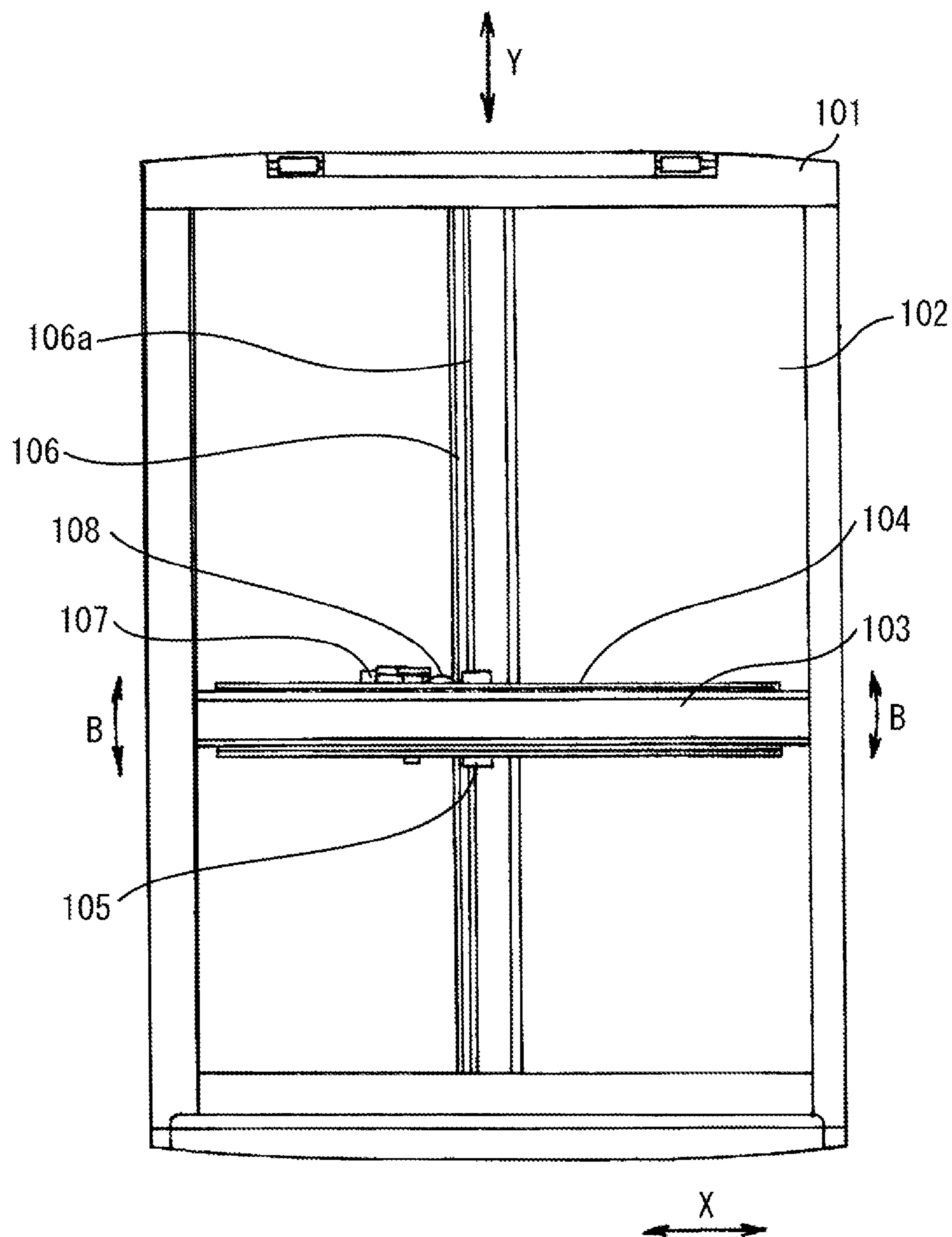
FIG. 9 PRIOR ART
