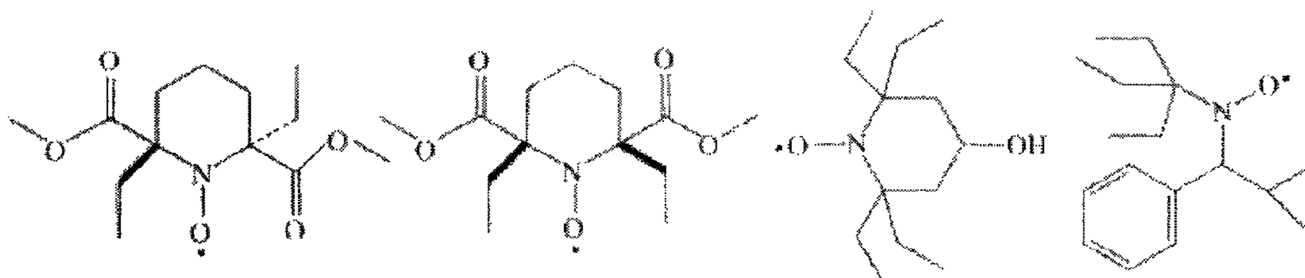
G1, LogP=2.0
