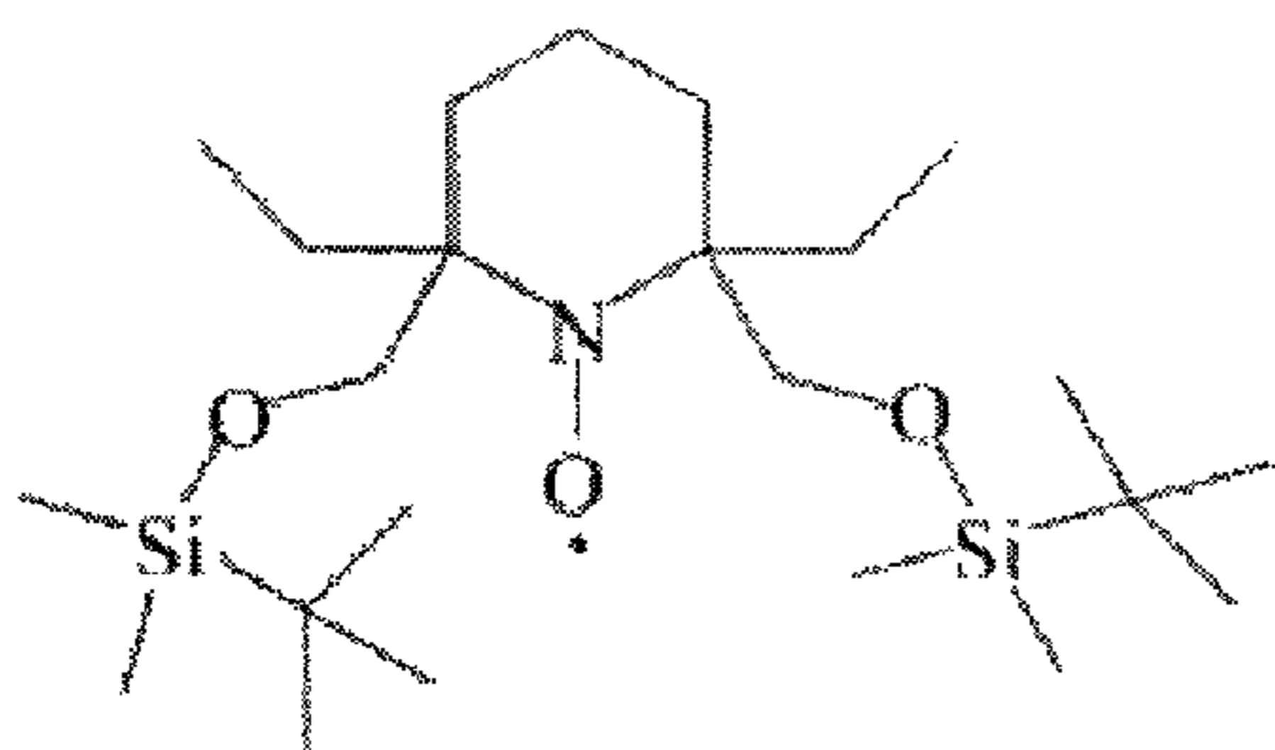
G5, LogP=8.2
