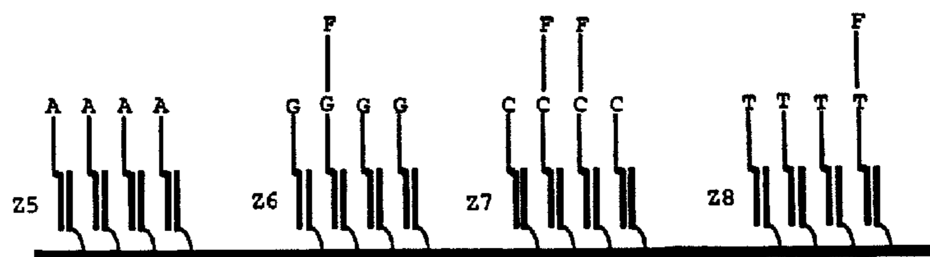
Heterozygous: G,C, and T alleles.
