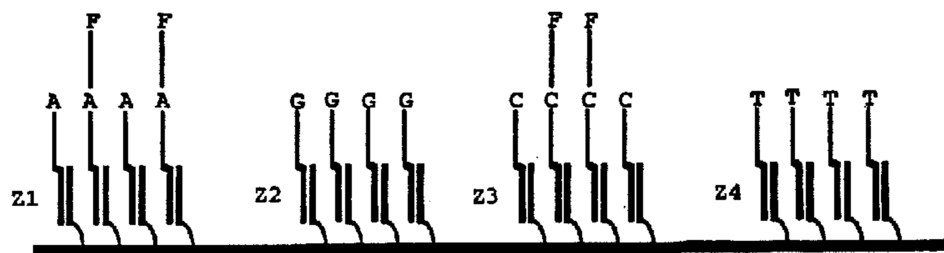
Heterozygous: A and C alleles.
