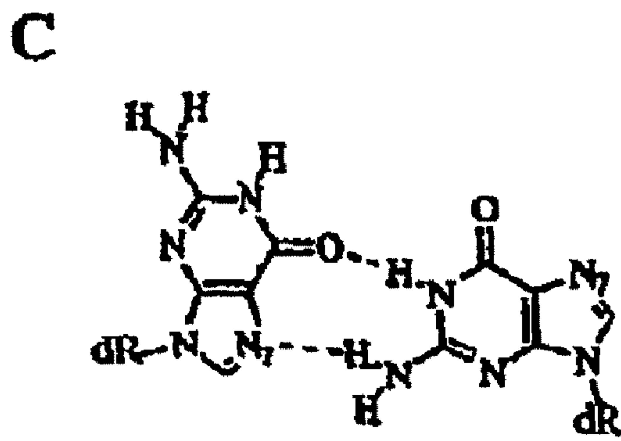
GG base pair
