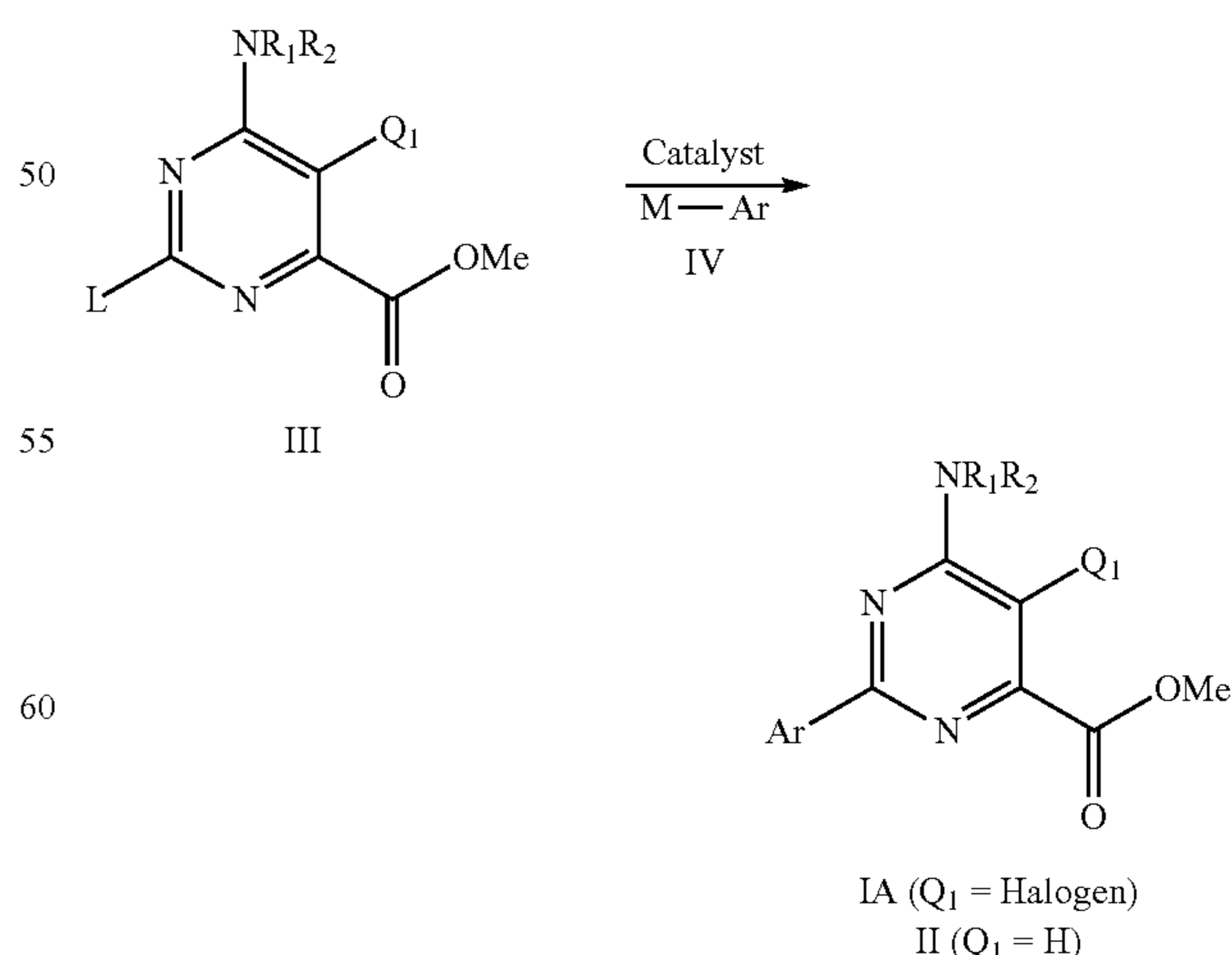
Scheme 2
