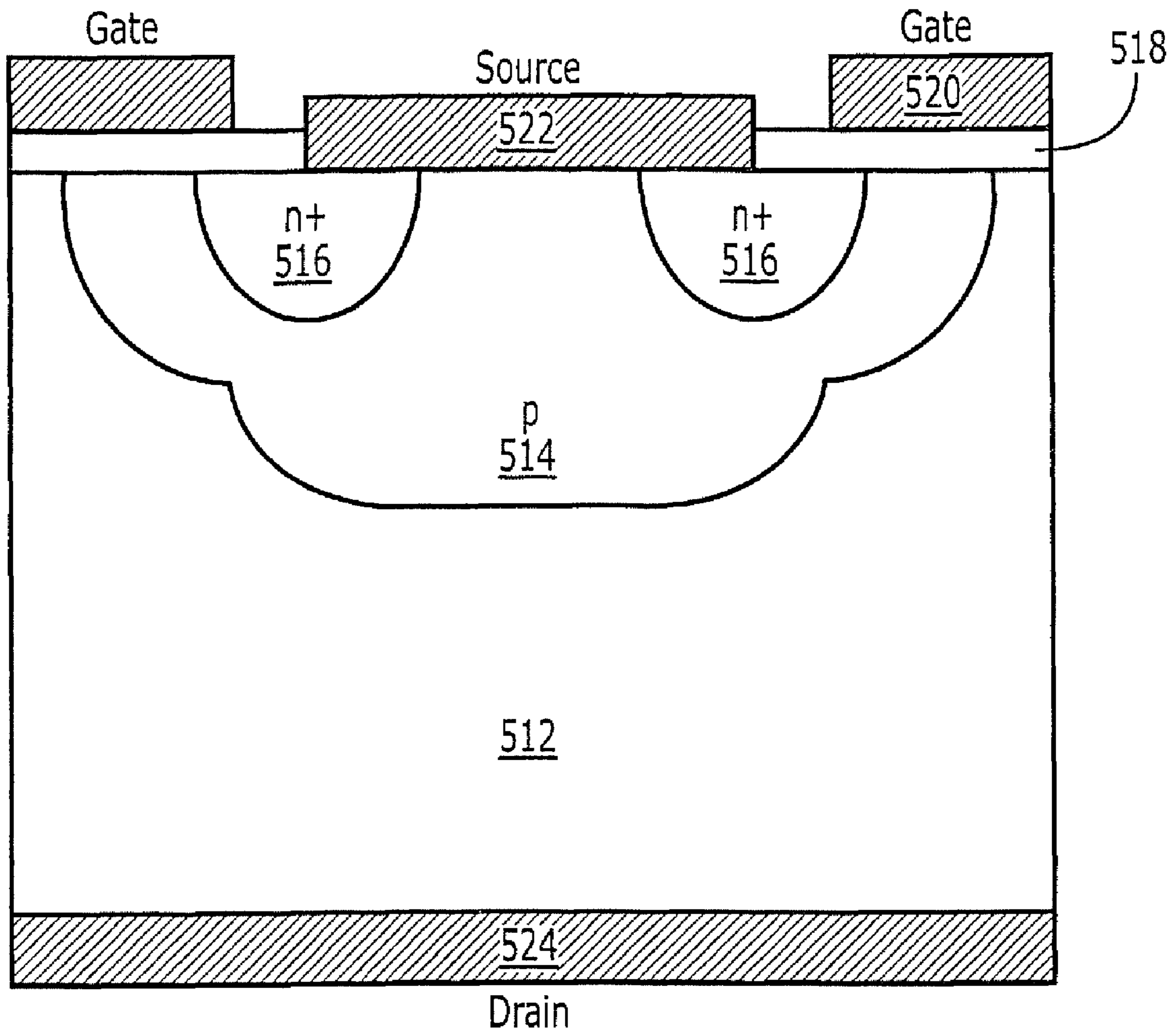
Figure 5 (RELATED ART)
