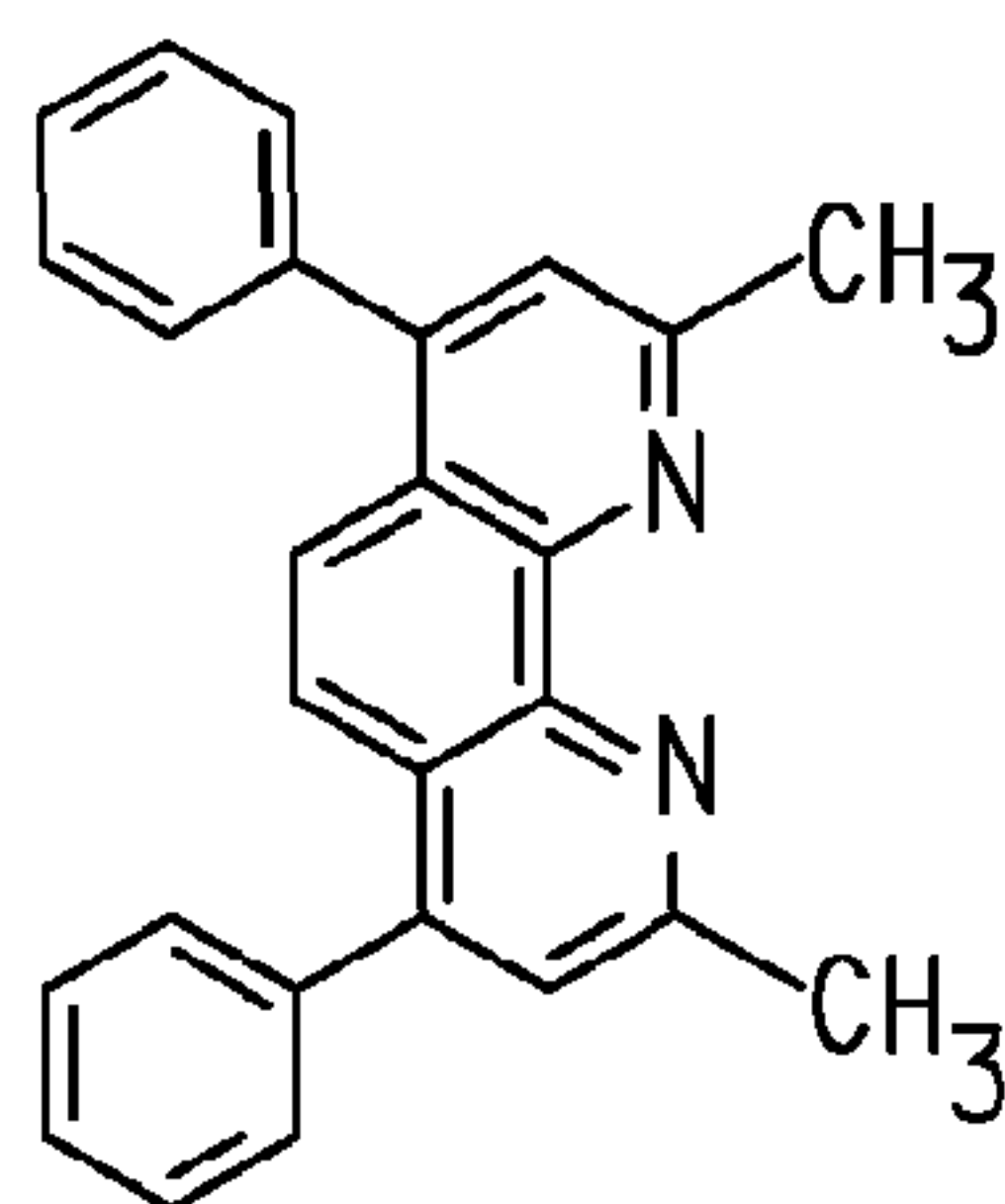
DDPa (Compound F)
