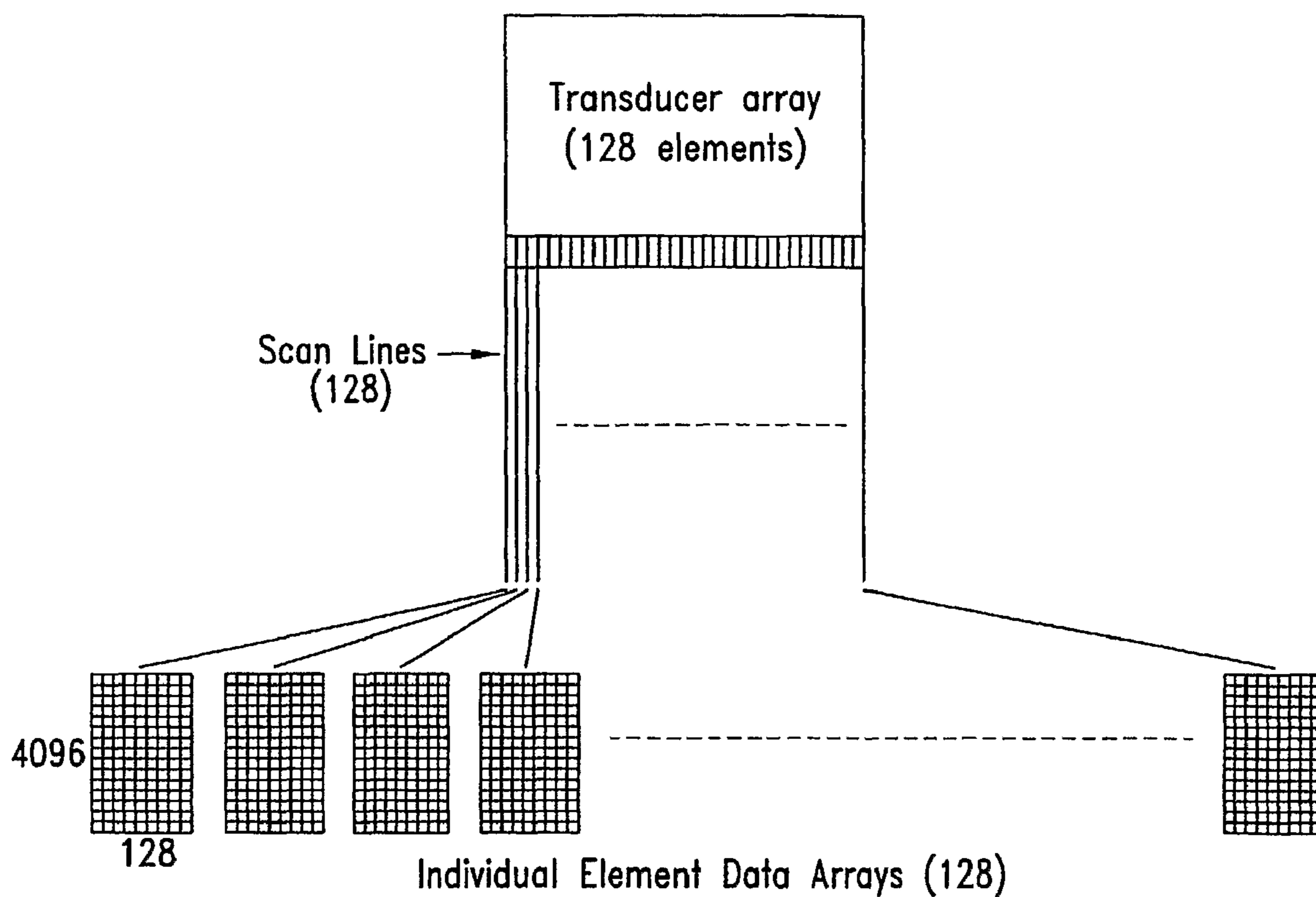
SCAN SEQUENCE AND DATA FOR A 128 ELEMENT LINEAR ARRAY
