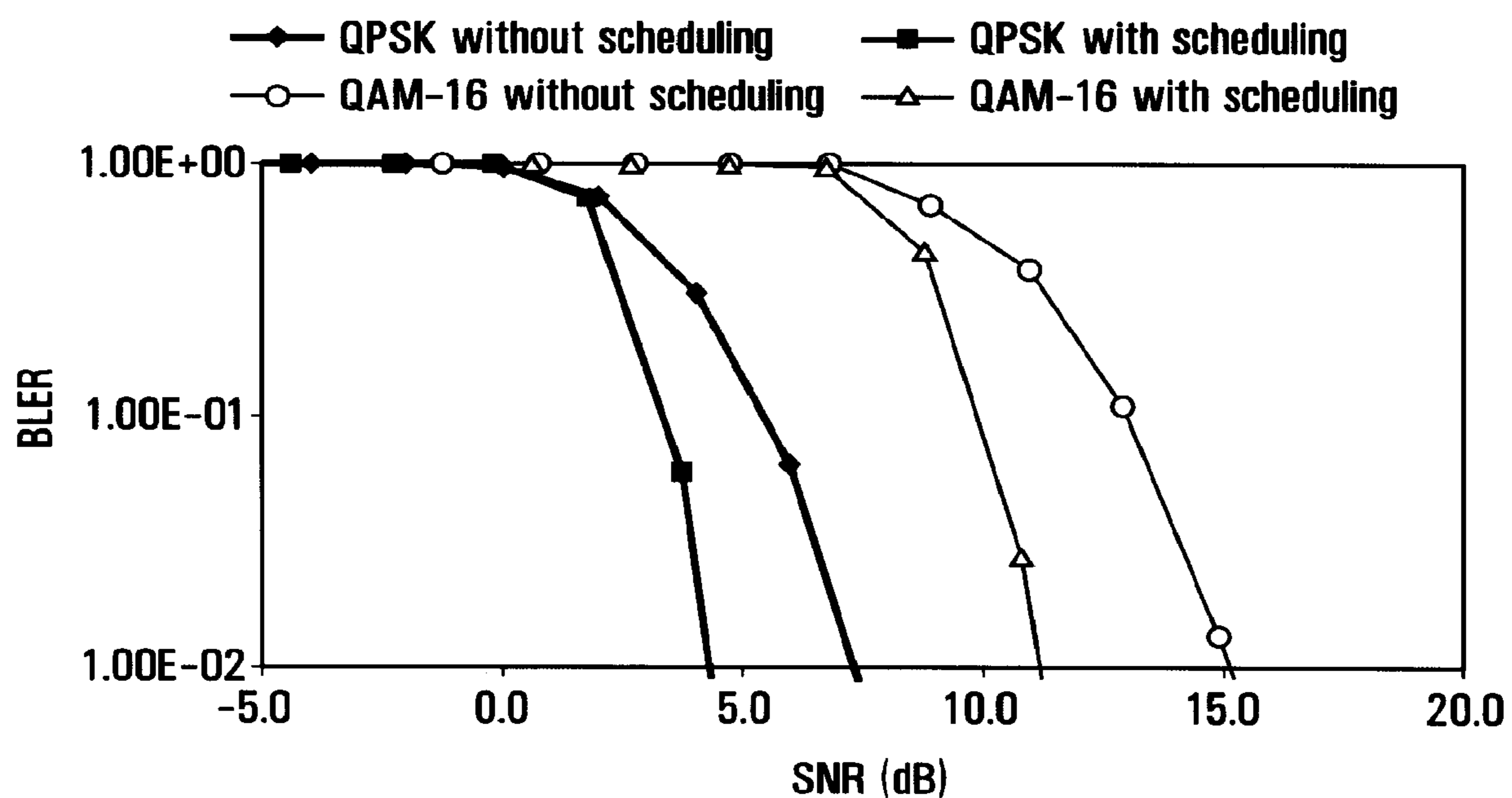
Impact on Max Capacity Scheduling (SM 2x2 MLD, 16 UEs, ITU-VA, Turbo R=1/2, 10MHz 1024-FFT, 6-Band)
