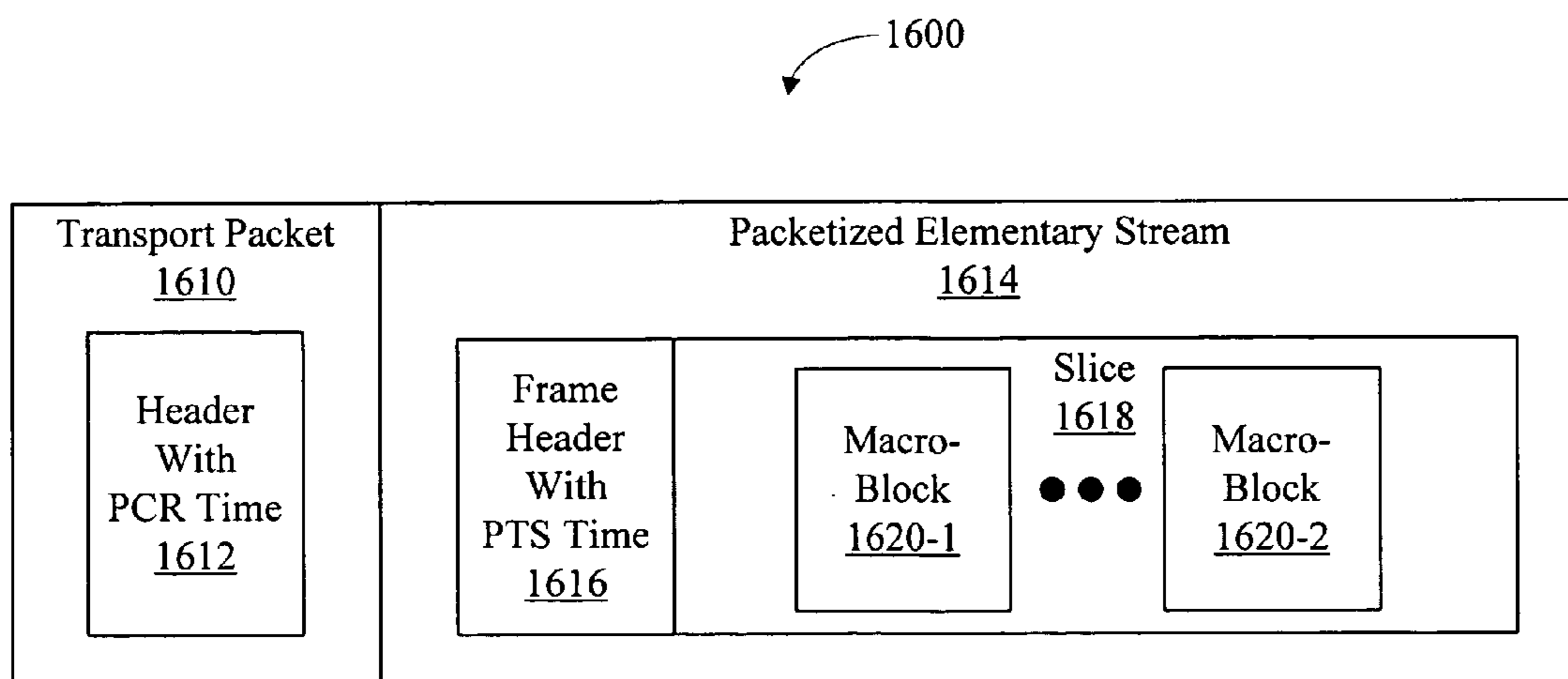
Figure 16 (Prior Art)
