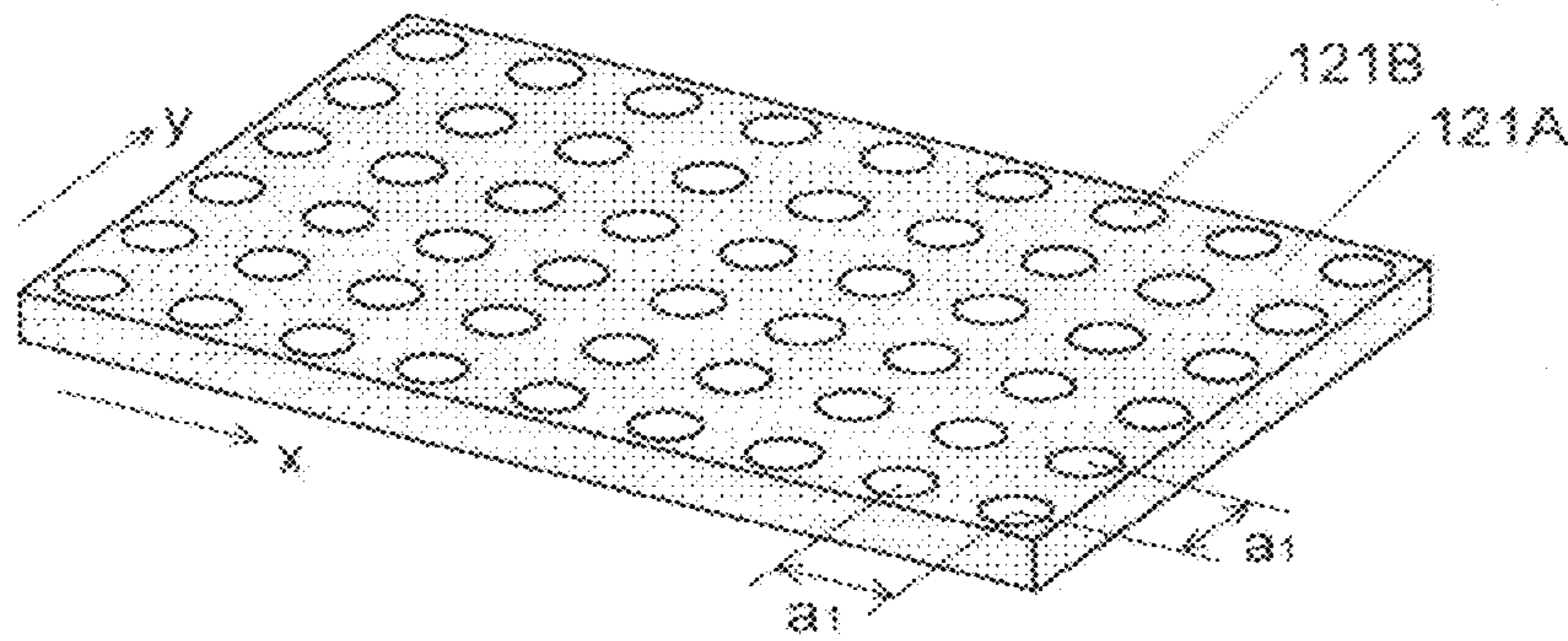
(a) 1ST TWO-DIMENSIONAL PHOTONIC CRYSTAL LAYER 121
