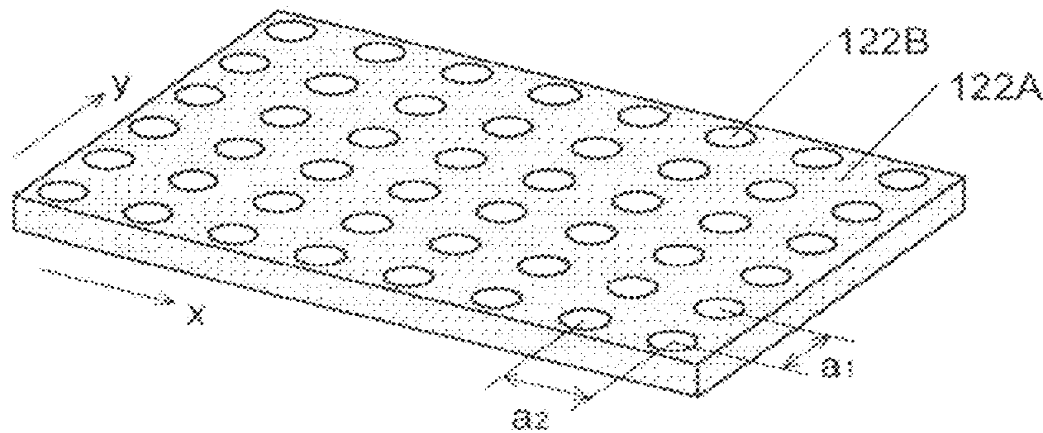
(b) 2ND TWO-DIMENSIONAL PHOTONIC CRYSTAL LAYER 122
