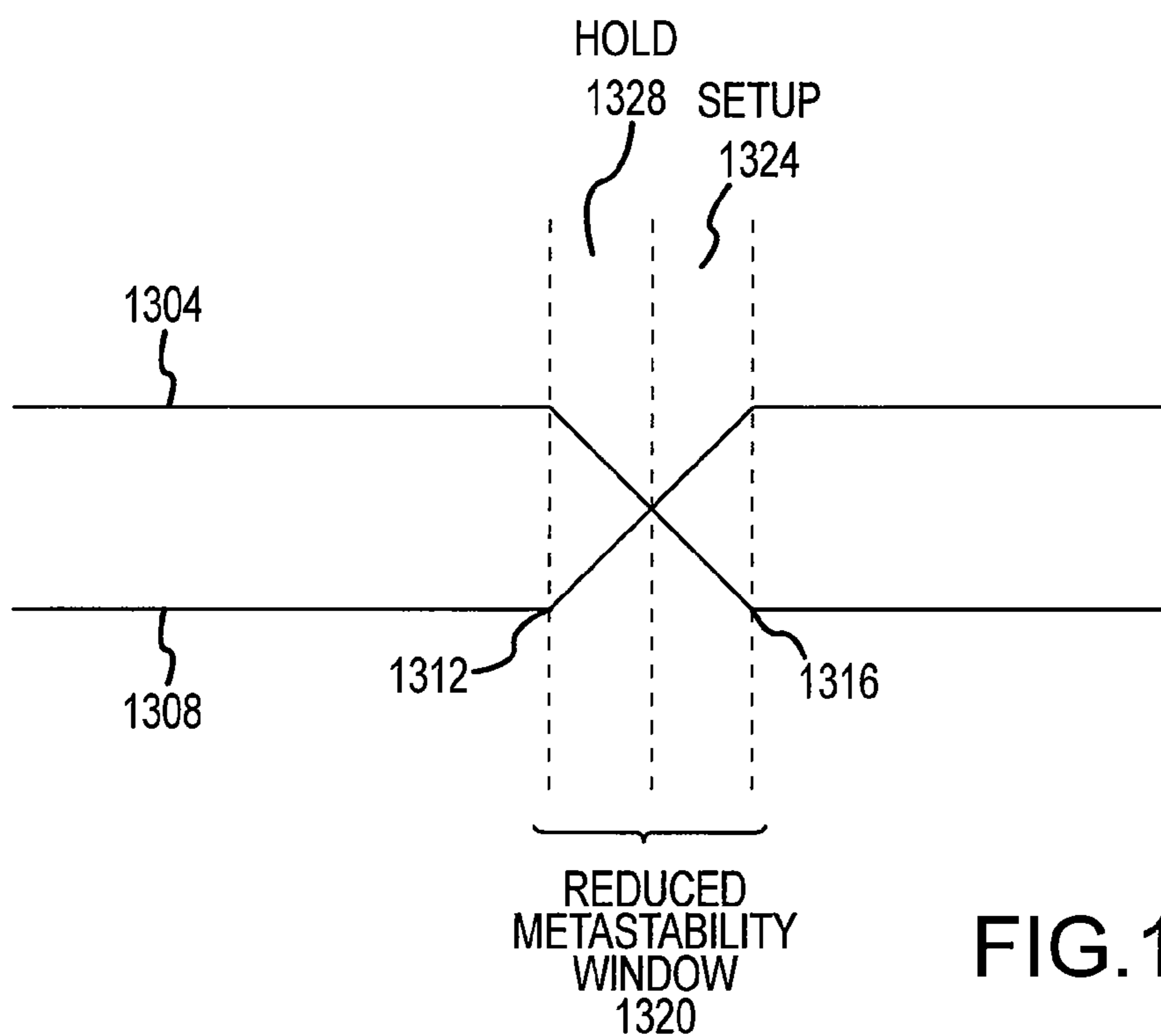
FIG.12 (PRIOR ART)
