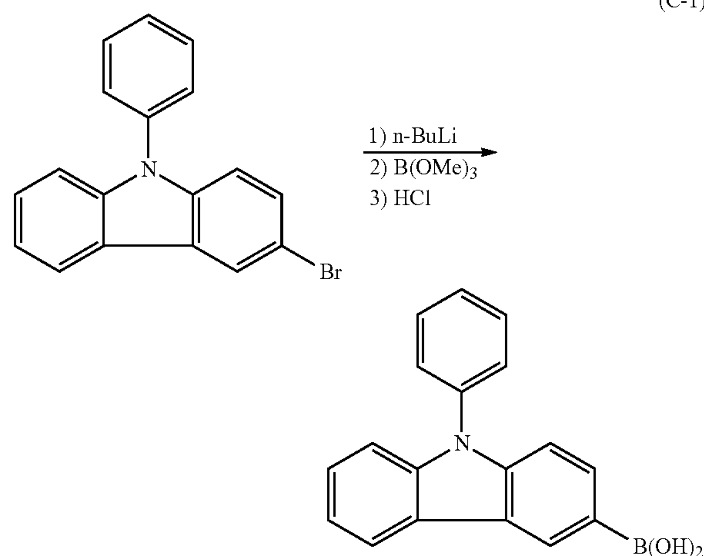
Step 2: Synthesis of 4-(9-phenyl-9H-carbazol-3-yl)diphenylamine (PCBA)
