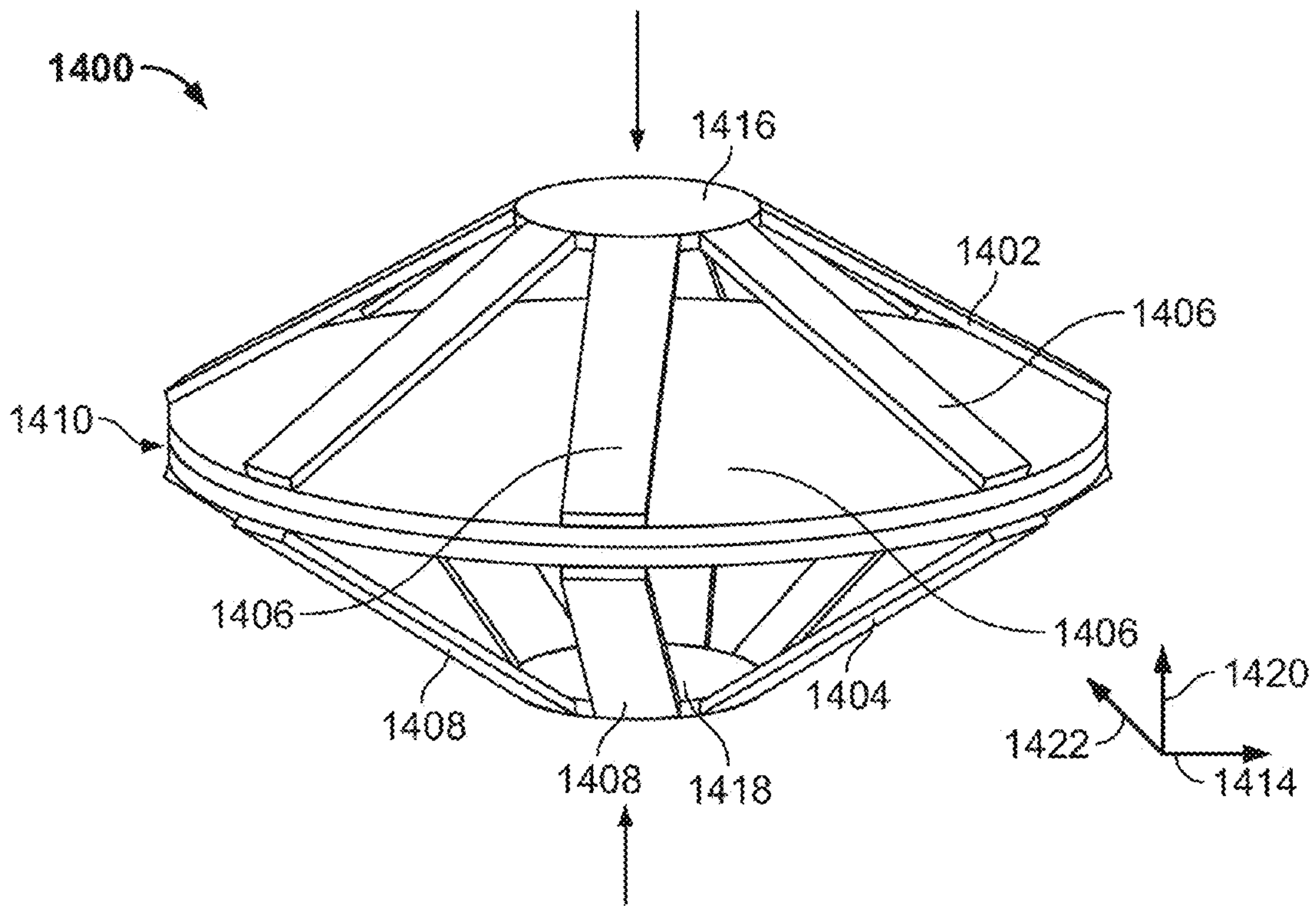
FIG. 21C (Prior Art)
