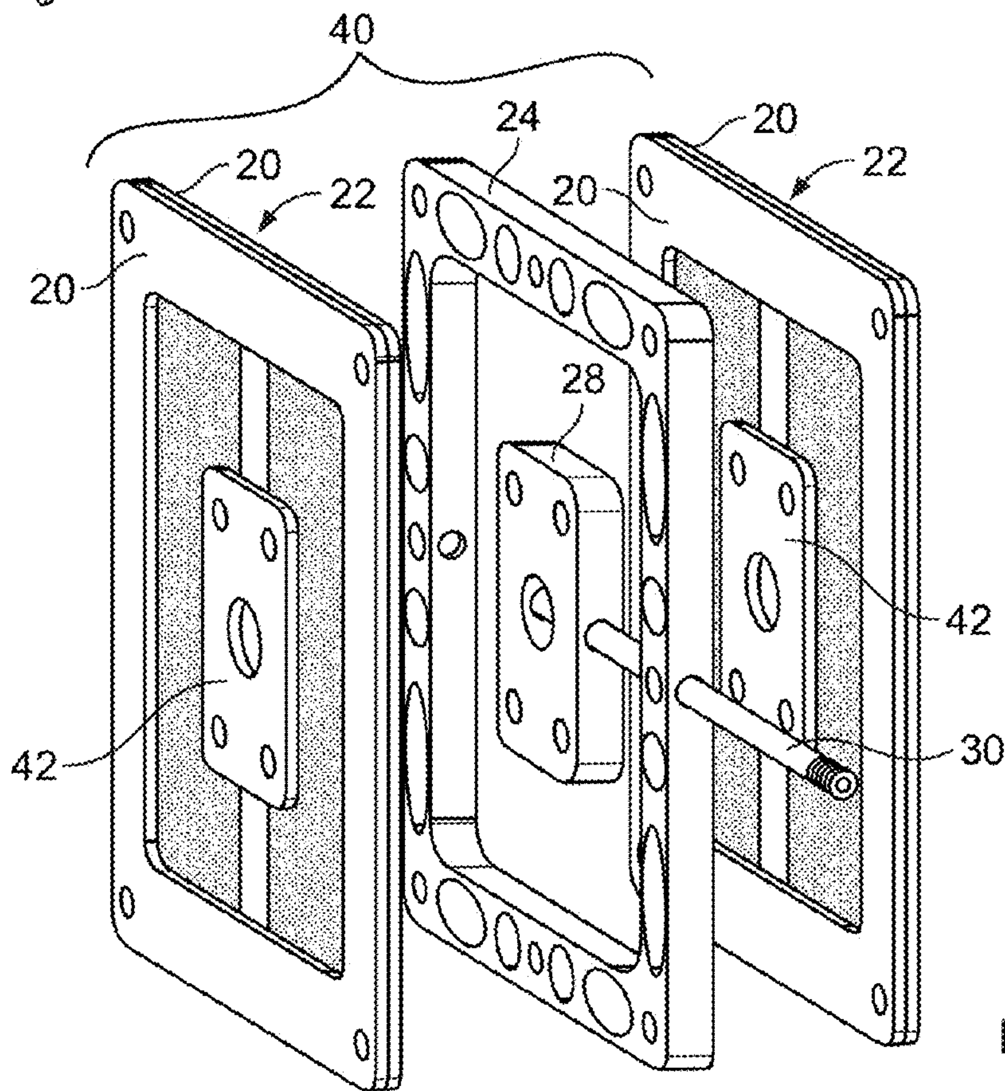
FIG. 3 (Prior Art)
