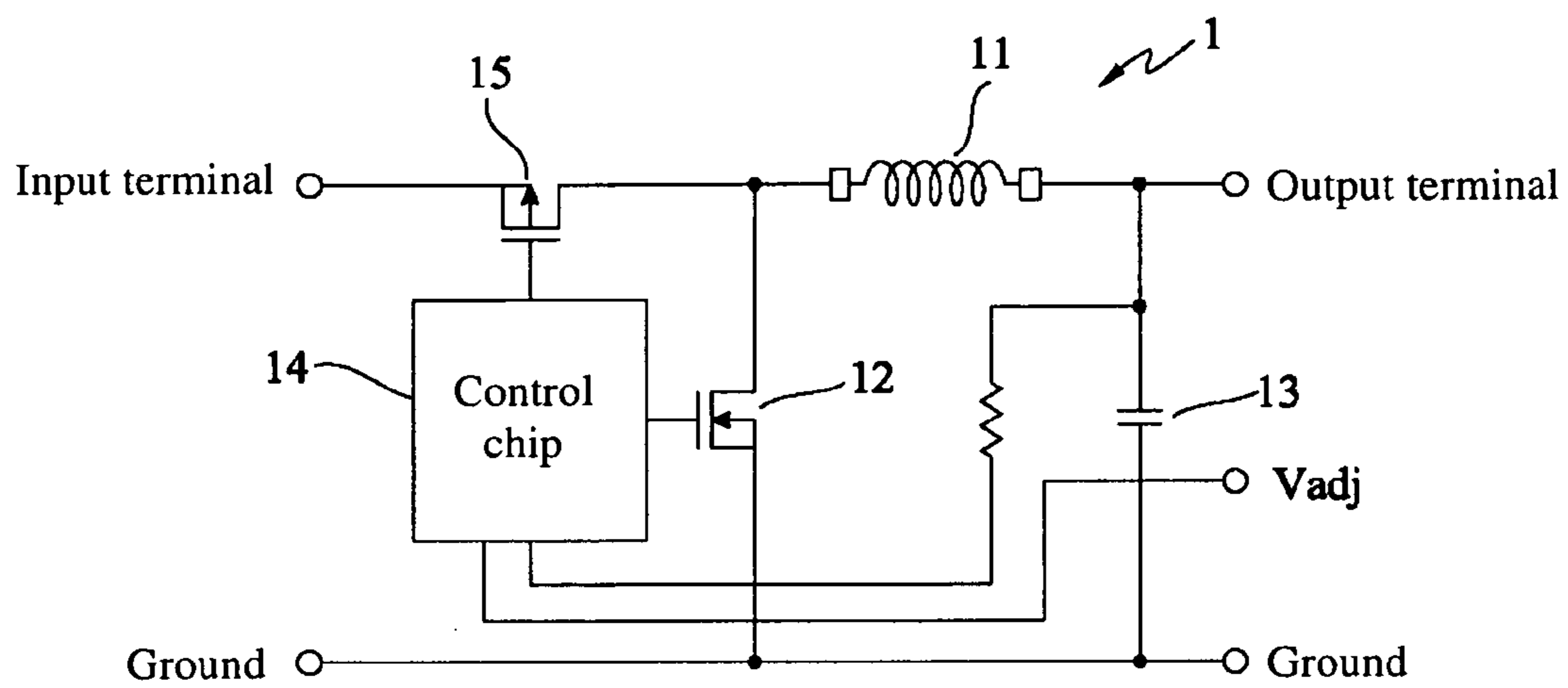
FIG. 1 (Prior Art)
