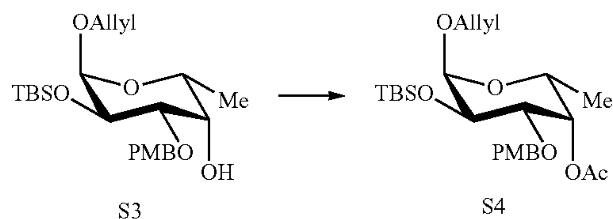
O-Allyl 4-O-acetyl-2-O-t-butyldimethylsilyl-3-O-methoxybenzyl- \alpha -D-fucopyranoside (S4)
