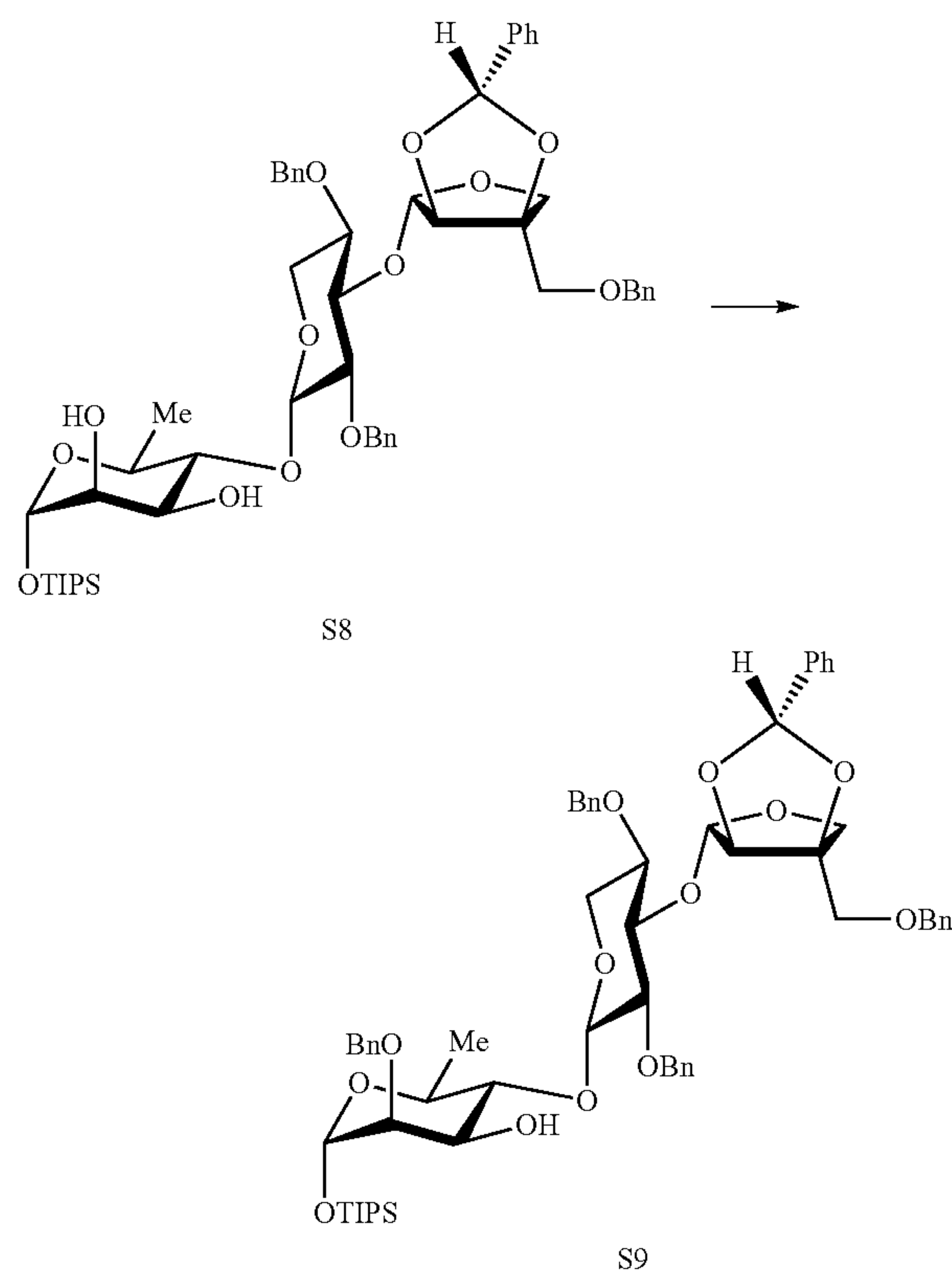
O-Triisopropylsilyl 2-O-benzyl- \{[5\text{-O-benzyl-}2,3\text{-di-O-benzylidene-}\beta\text{-D-apiofuranosyl-(1}\rightarrow\text{3)}]\text{-}2,4\text{-di-O-benzyl-}\beta\text{-D-xylopyranosyl-(1}\rightarrow\text{4)}]\}\text{-}\alpha\text{-L-rhamnopyranoside (S9)}
