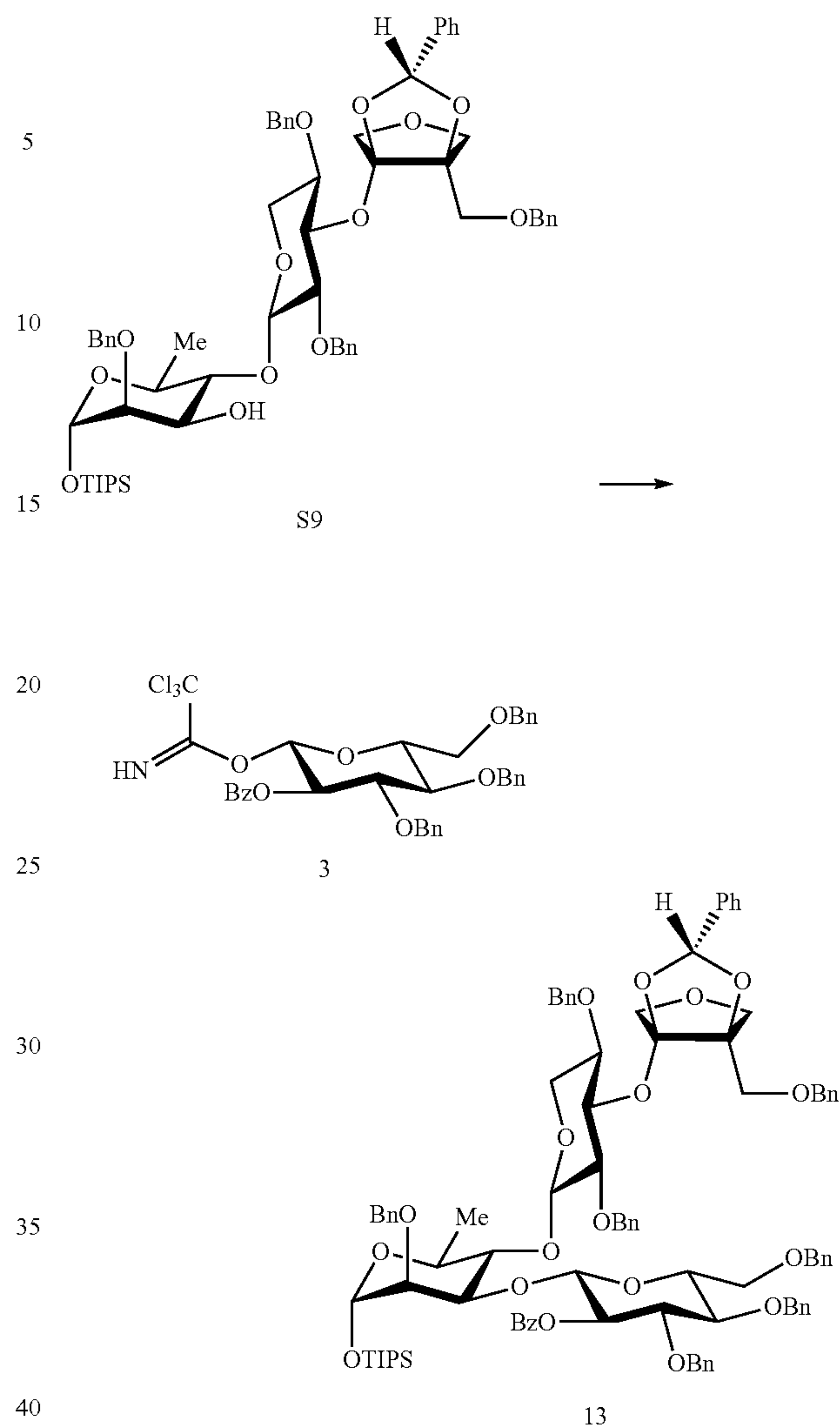
O-Triisopropylsilyl[2-O-benzoyl-3,4,6-tri-O-benzyl- \beta\text{-D-glucopyranosyl-(1}\rightarrow\text{3)}]-2\text{-O-benzyl-}\{[5\text{-O-benzyl-}2,3\text{-di-O-benzylidene-}\beta\text{-D-apiofuranosyl-(1}\rightarrow\text{3)}]-2,4\text{-di-O-benzyl-}\beta\text{-D-xylopyranosyl-(1}\rightarrow\text{4)}]\} - \alpha\text{-L-rhamnopyranoside (13)}
