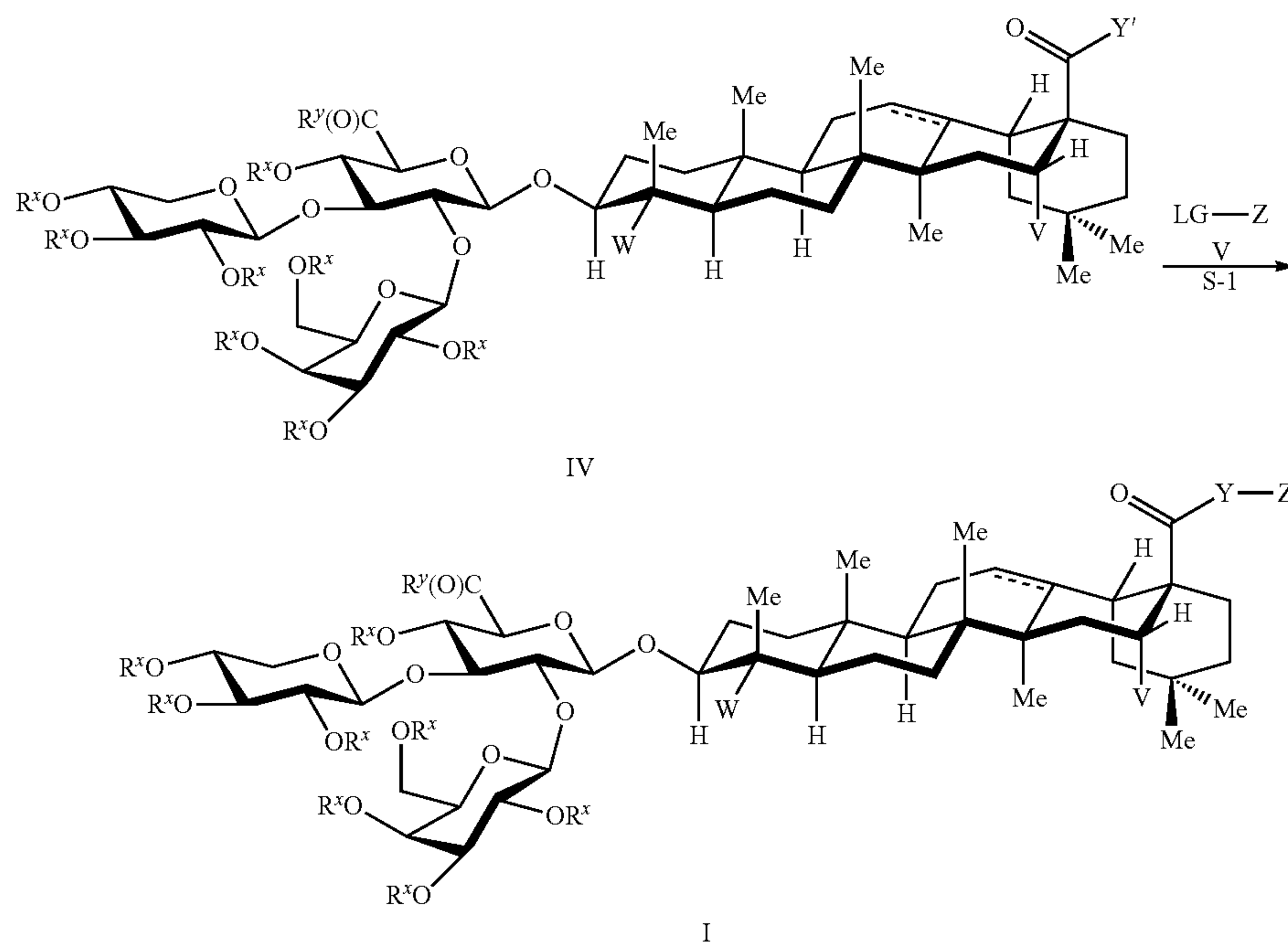
Scheme 1
