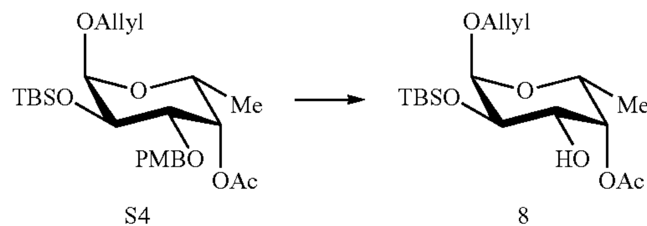
O-Allyl 4-O-acetyl-2-O-t-butyldimethylsilyl- \alpha -D-fucopyranoside (8)
