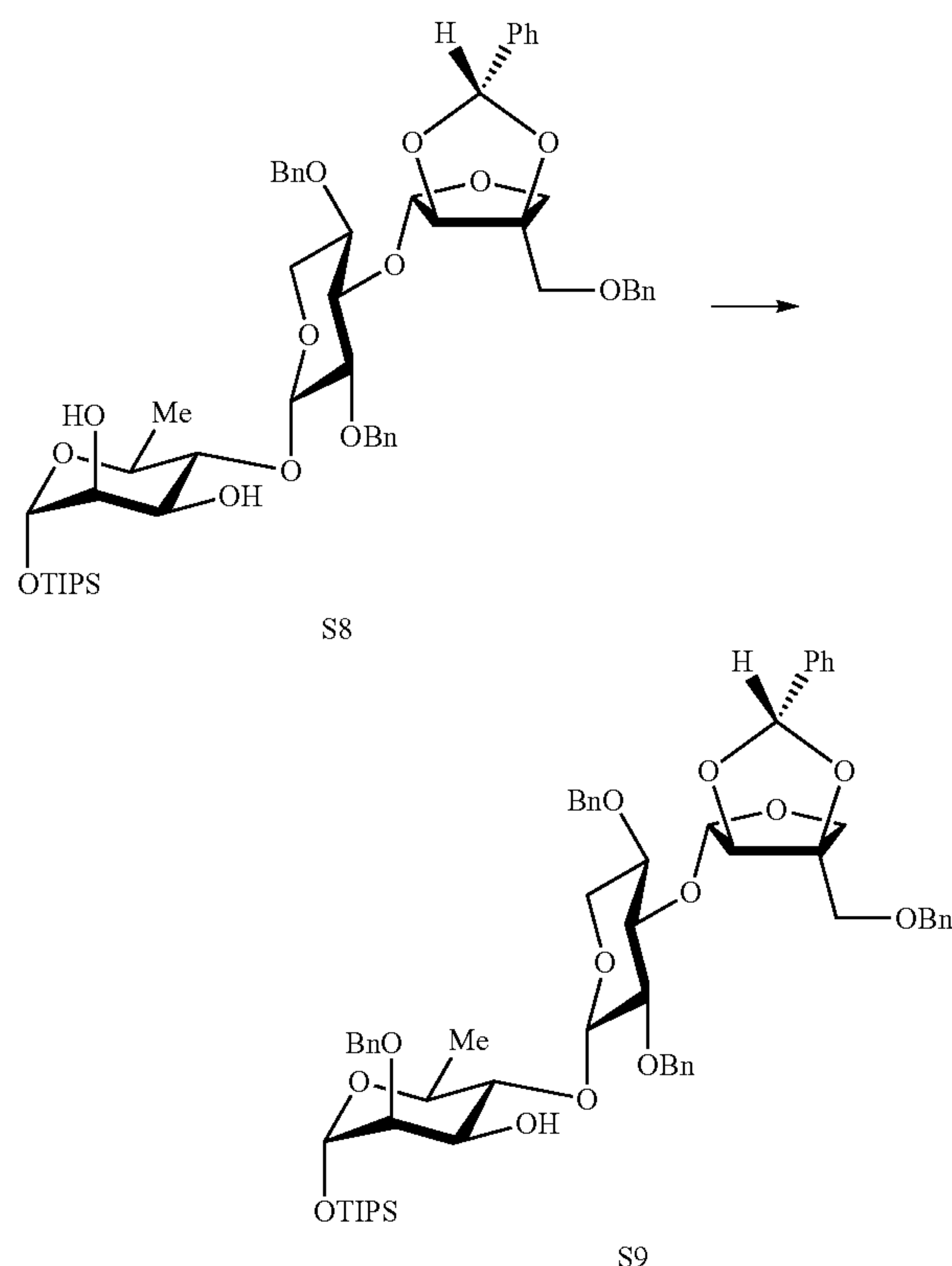
O-Triisopropylsilyl 2-O-benzyl- \{[5\text{-O-benzyl-}2,3\text{-di-O-benzylidene-}\beta\text{-D-apiofuranosyl-(1}\rightarrow\text{3)}]-2,4\text{-di-O-benzyl-}\beta\text{-D-xylopyranosyl-(1}\rightarrow\text{4)}]\} - \alpha\text{-L-rhamnopyranoside (S9)}
