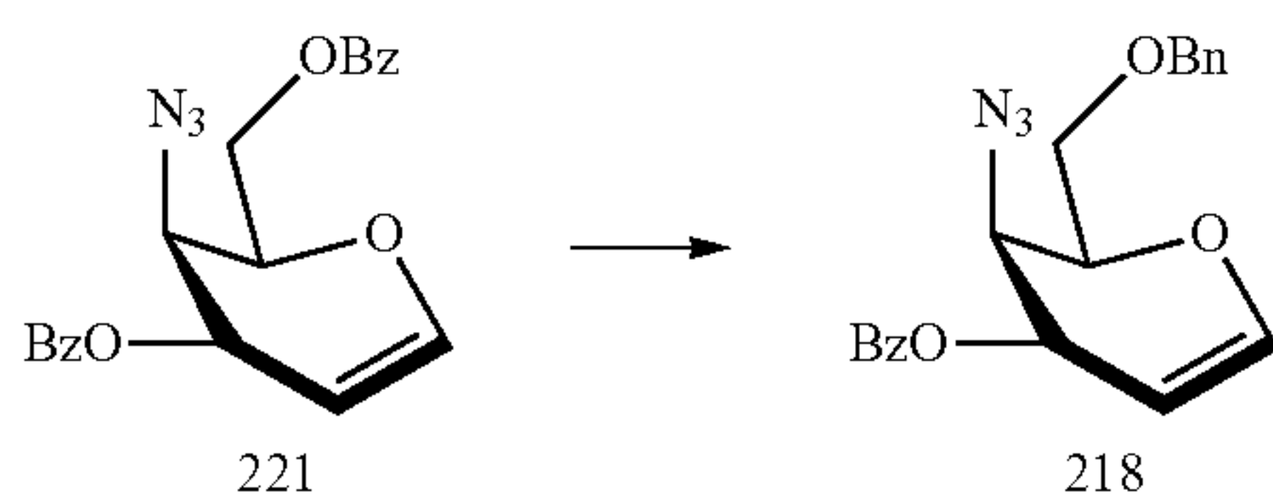
3,6-Di-O-benzyl-4-azido-4-deoxy-D-galactal (218)
