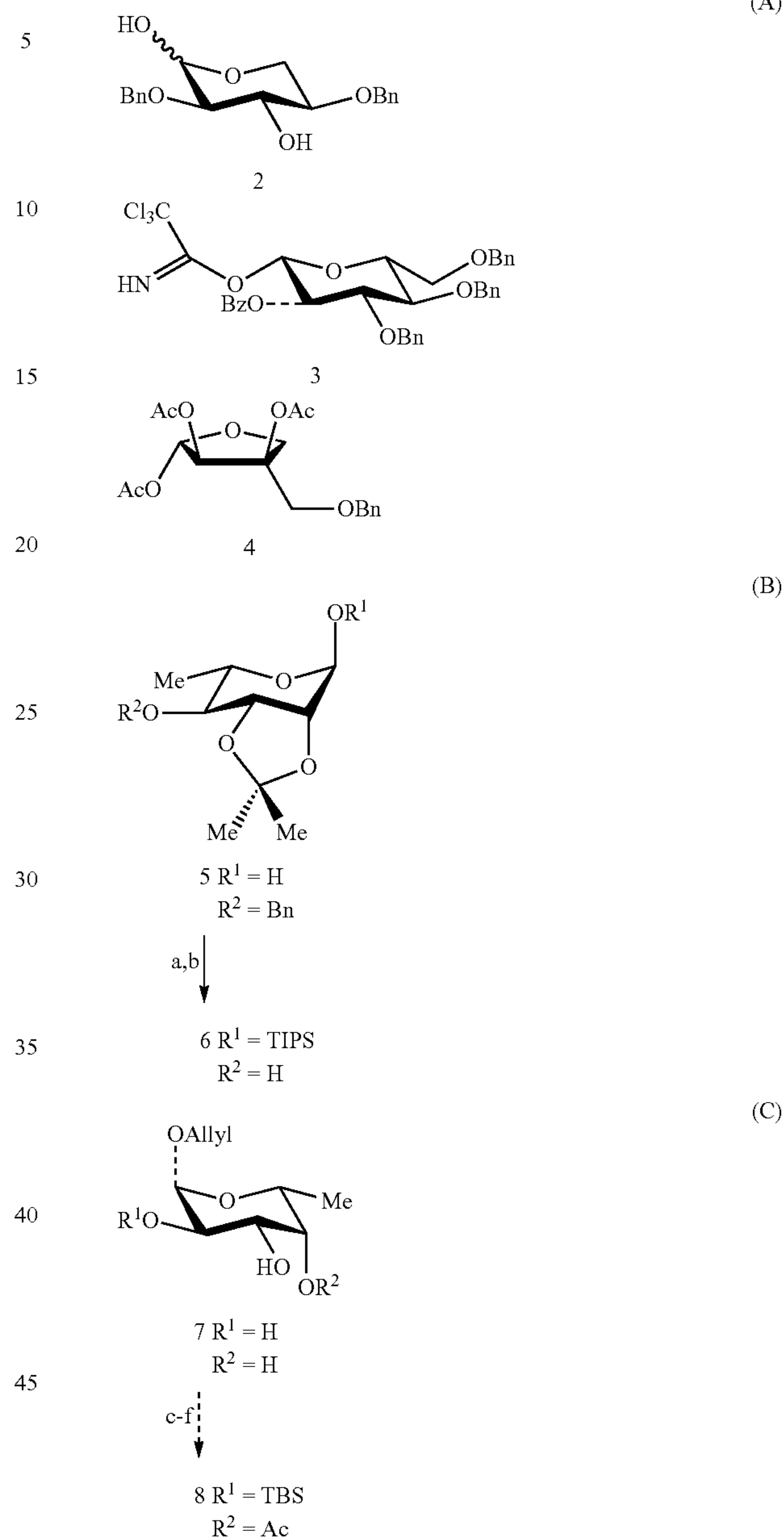
Scheme 7 a
