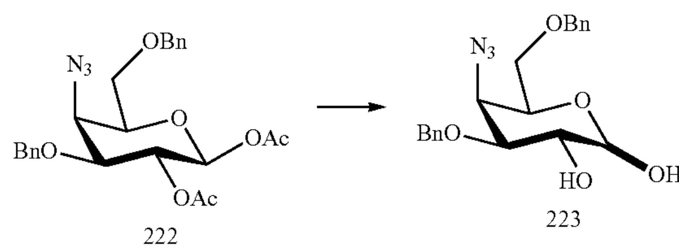
4-azido-4-deoxy-3,6-di-O-benzyl-D-galactopyranose (223)
