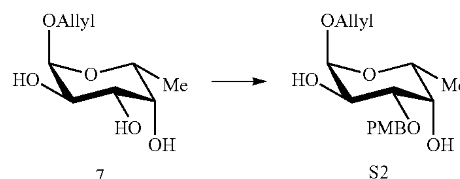
Allyl 3-O-methoxybenzyl- \alpha -D-fucopyranoside (S2)
