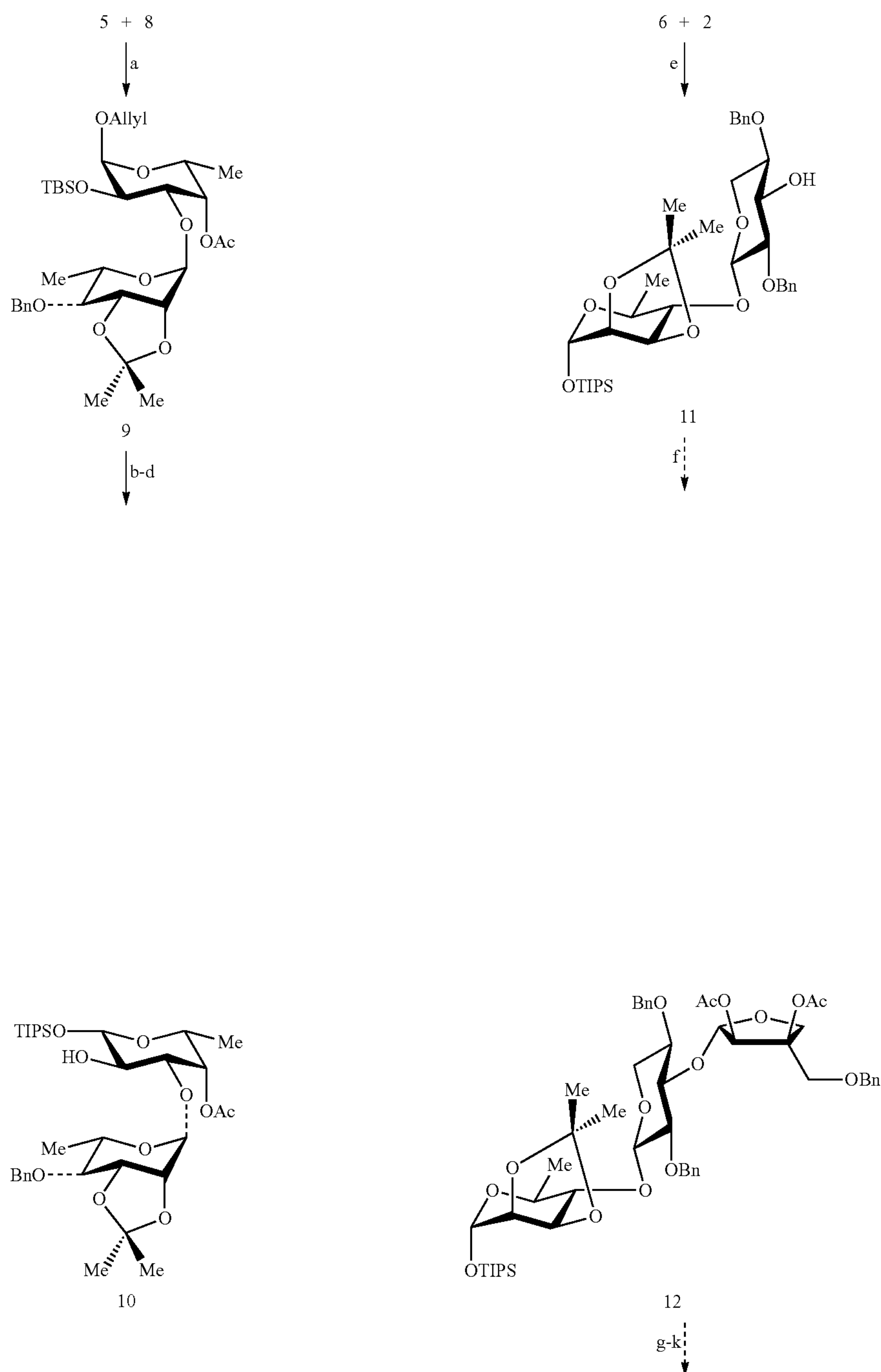
Scheme 8 a
