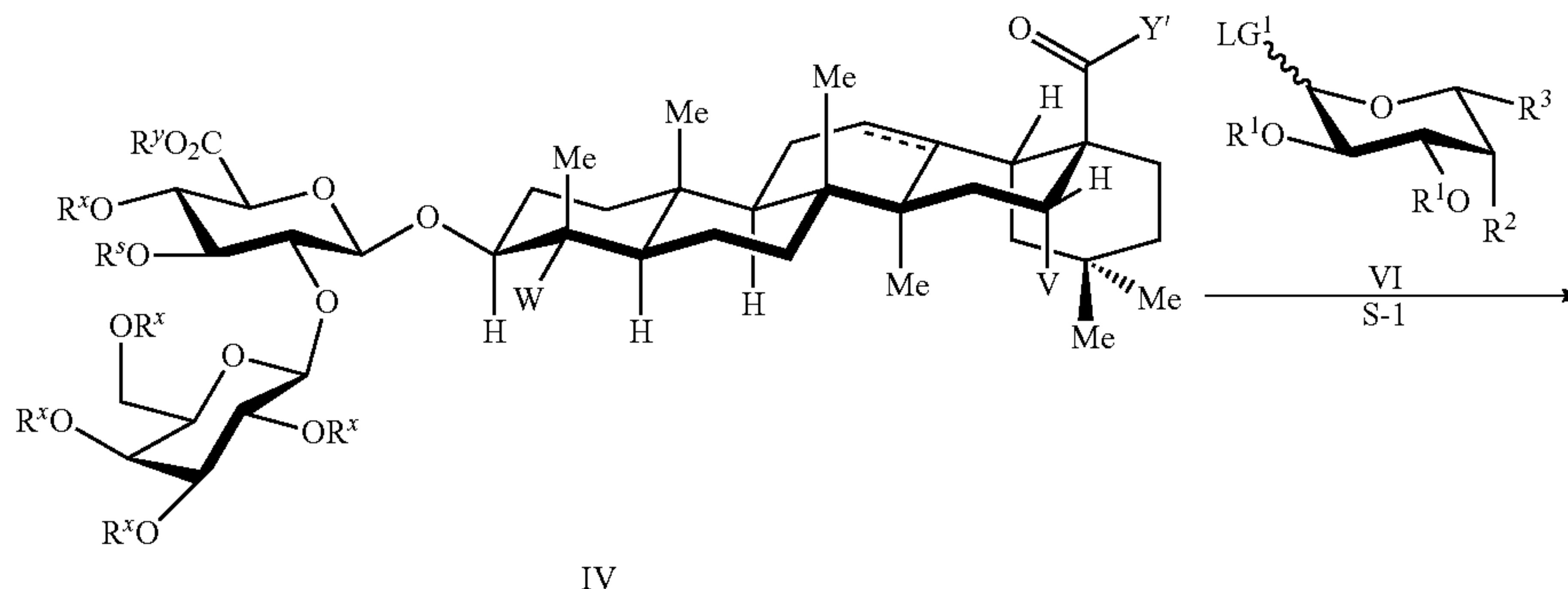
Scheme 2
