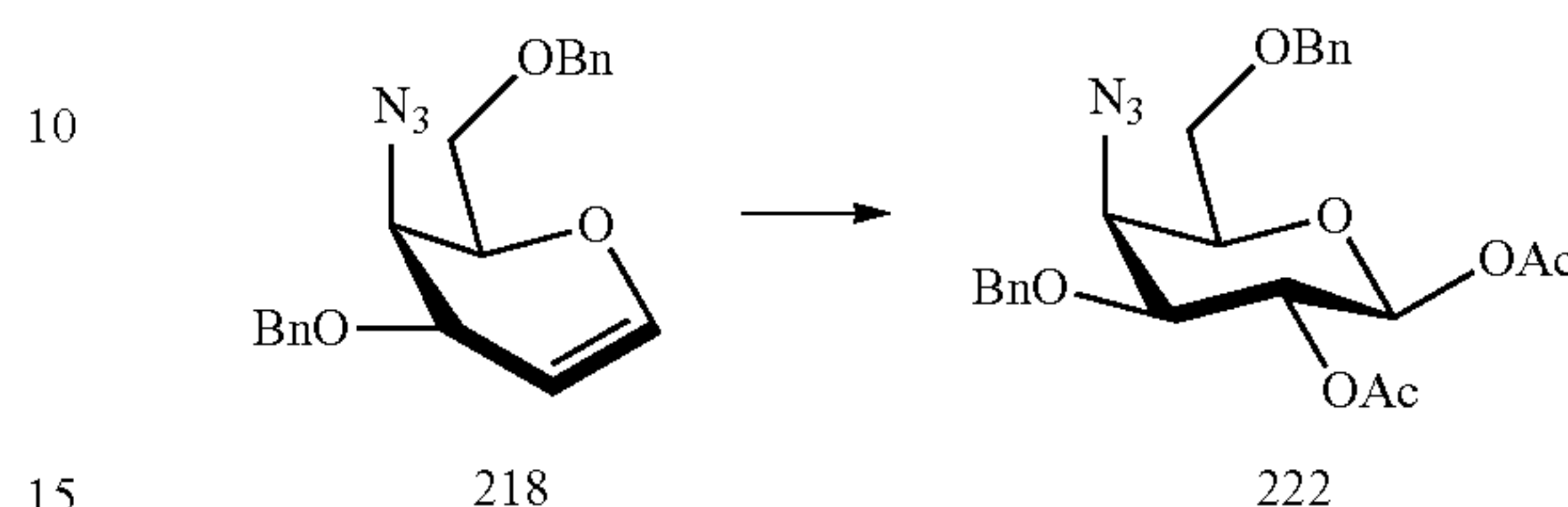
O-Acetyl 2-O-acetyl-4-azido-4-deoxy-3,6-di-O-benzyl- \beta -D-galactopyranoside (222)
