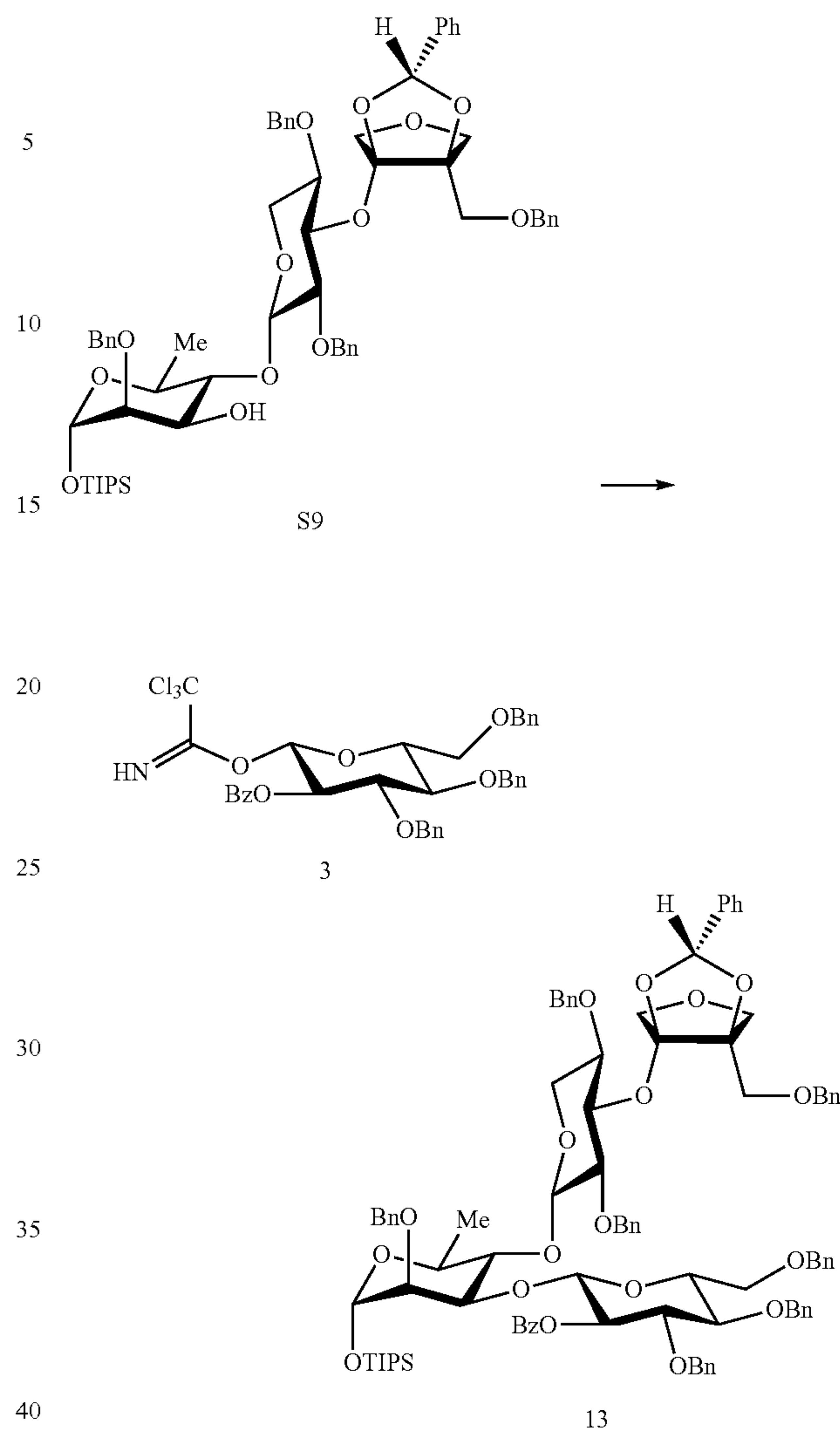
O-Triisopropylsilyl[2-O-benzoyl-3,4,6-tri-O-benzyl- \beta\text{-D-glucopyranosyl-(1}\rightarrow\text{3)}]\text{-}2\text{-O-benzyl-}\{[5\text{-O-benzyl-}2,3\text{-di-O-benzylidene-}\beta\text{-D-apiofuranosyl-(1}\rightarrow\text{3)}]\text{-}2,4\text{-di-O-benzyl-}\beta\text{-D-xylopyranosyl-(1}\rightarrow\text{4)}]\}\text{-}\alpha\text{-L-rhamnopyranoside (13)}
