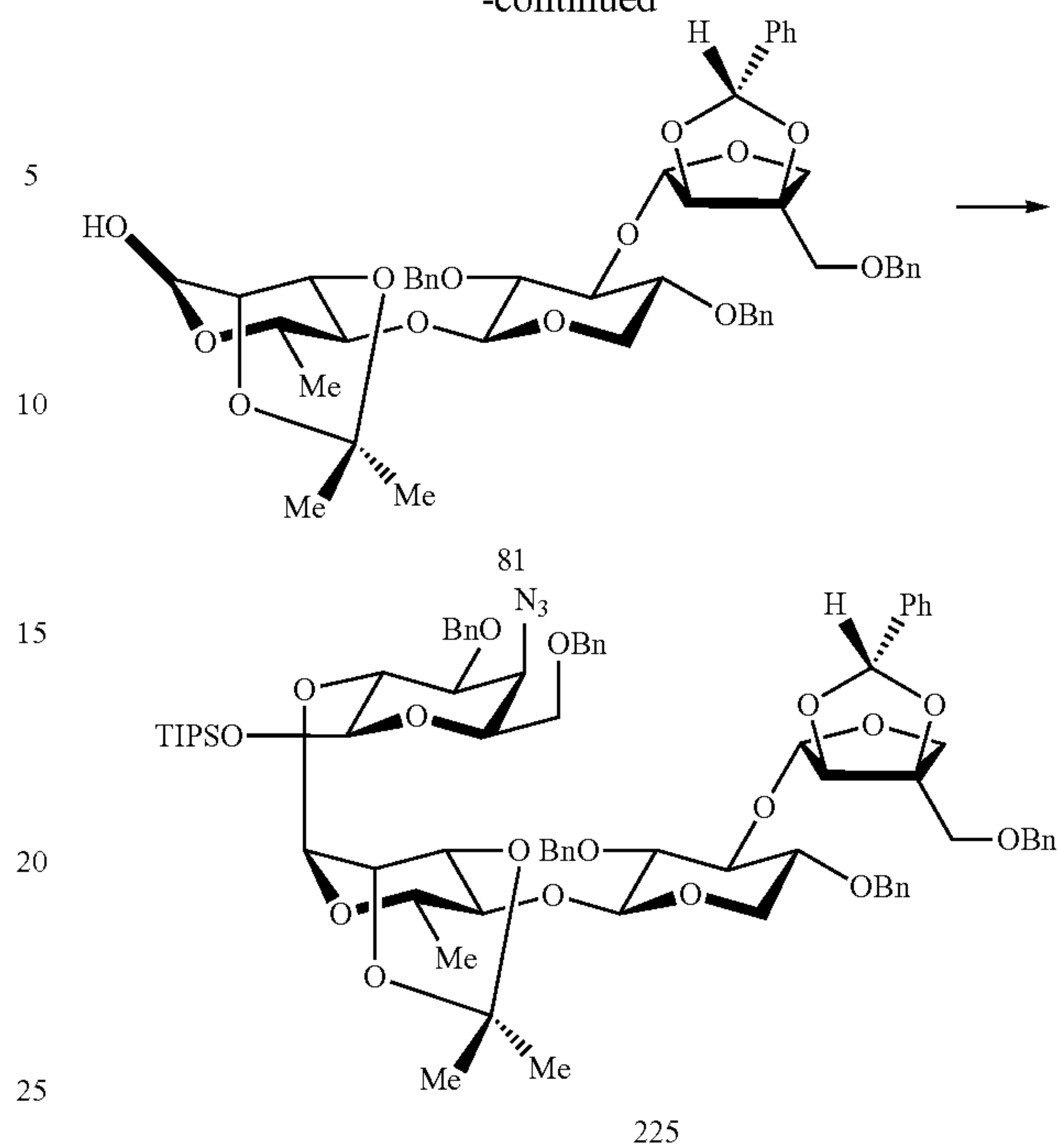
Azido tetrasaccharide 225
