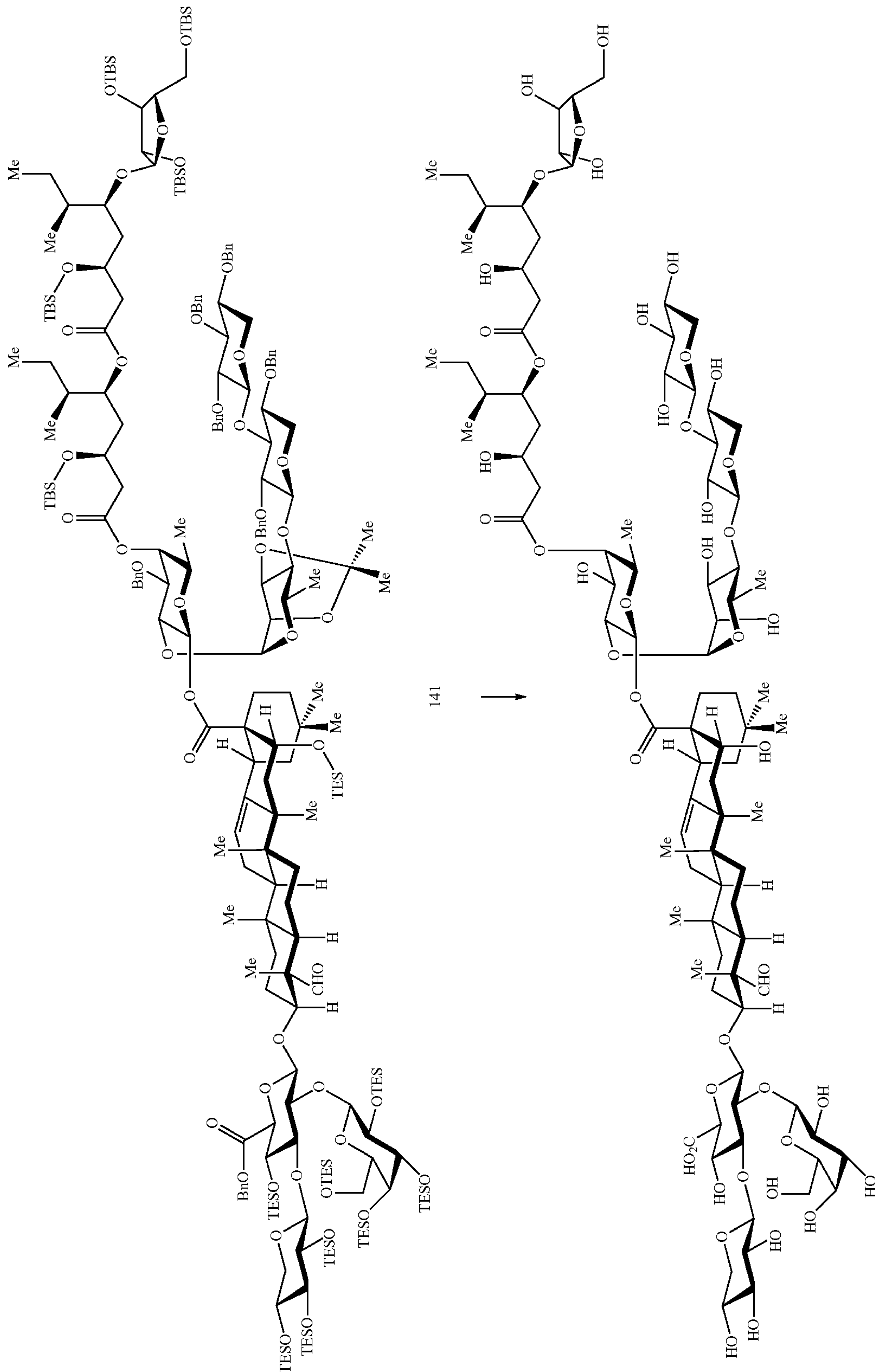
QS-21-Xyl (5)
