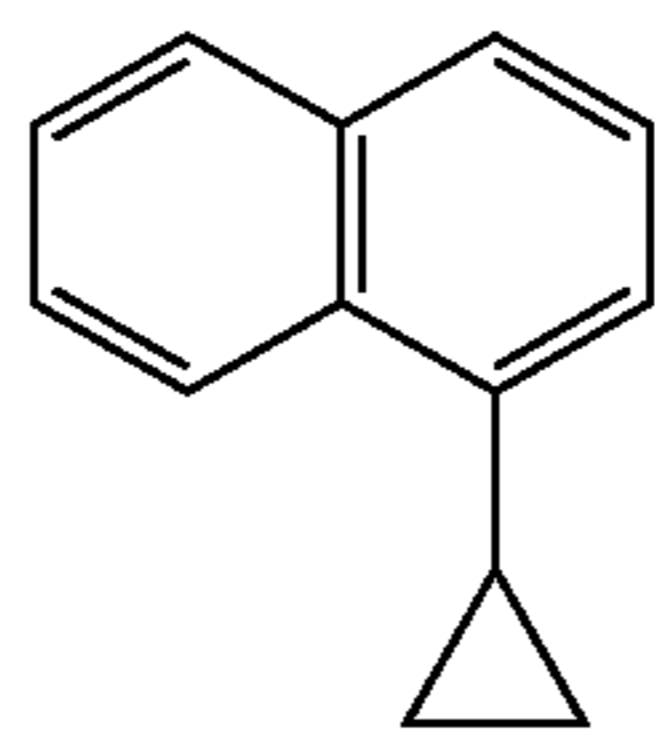
1-Cyclopropylnaphthalene
