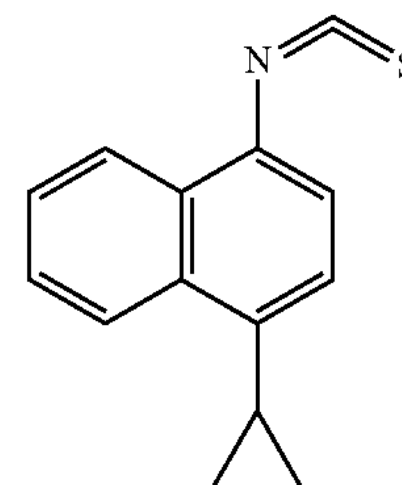
1-Cyclopropyl-4-isothiocyanatonaphthalene
