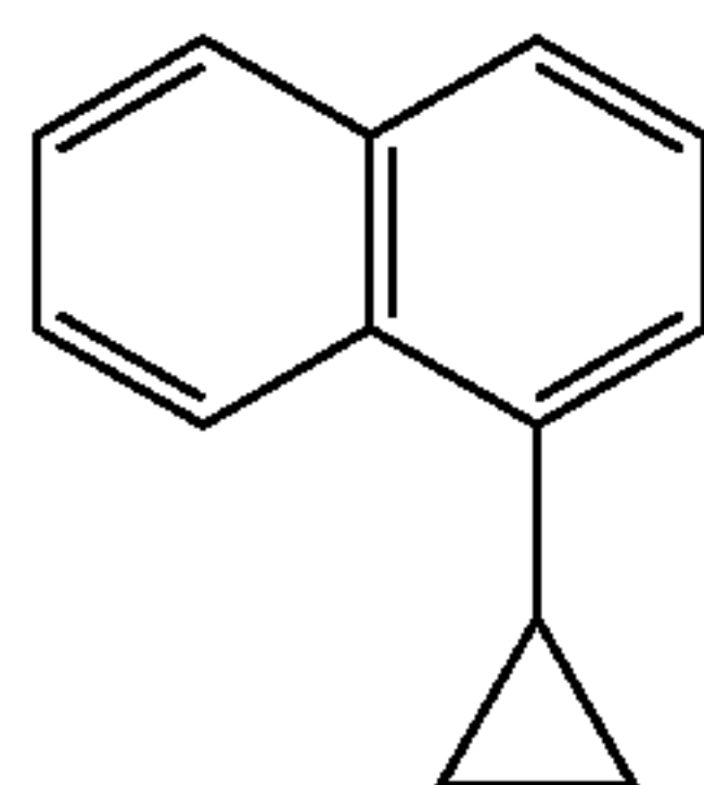
1-Cyclopropylnaphthalene
