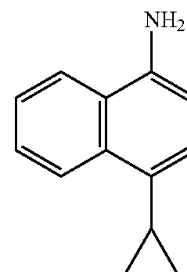
1-Amino-4-cyclopropylnaphthalene
