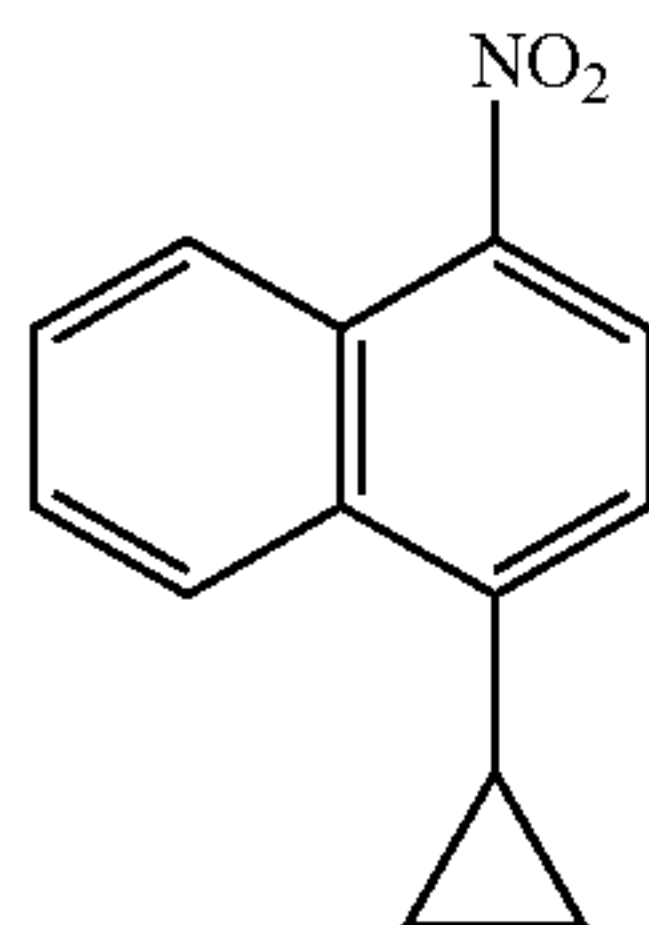
1-Cyclopropyl-4-nitronaphthalene
