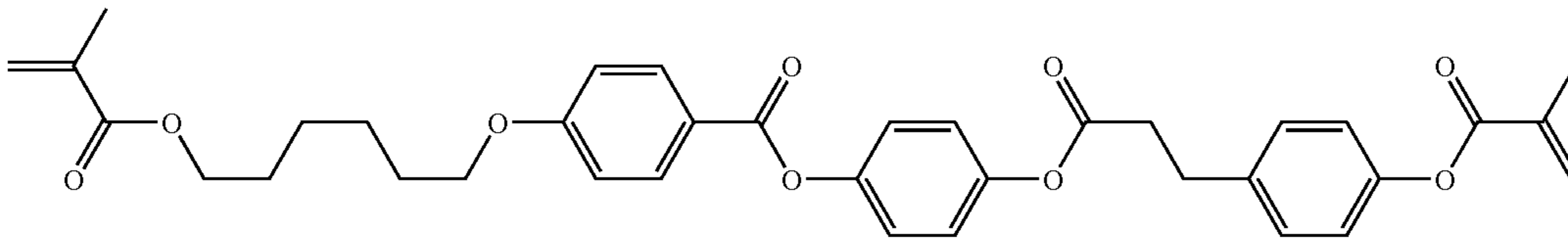
Polymerizable Compound No.14
