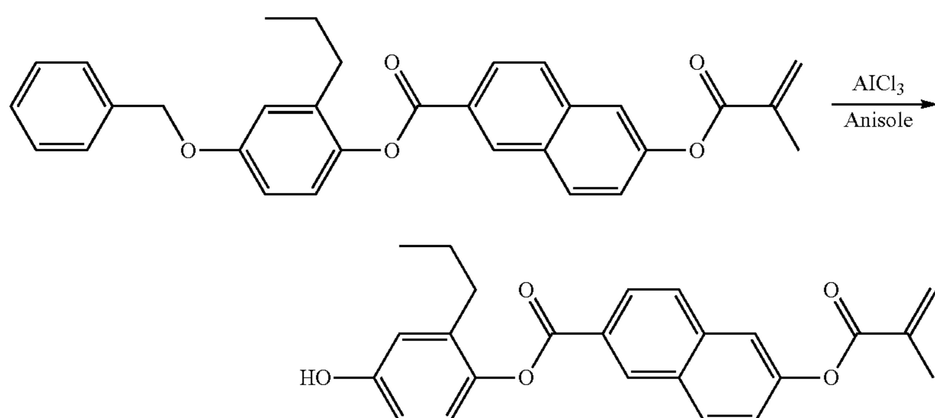
(Reaction Scheme 2)
