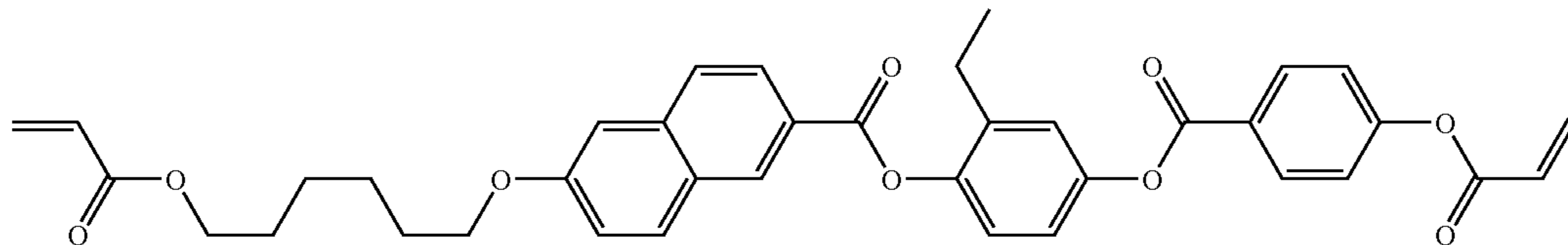
Polymerizable Compound No.27
