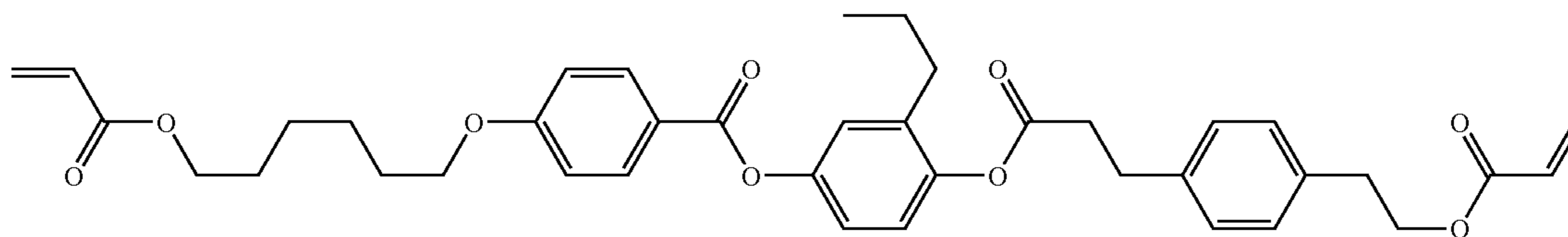
Polymerizable Compound No.37
