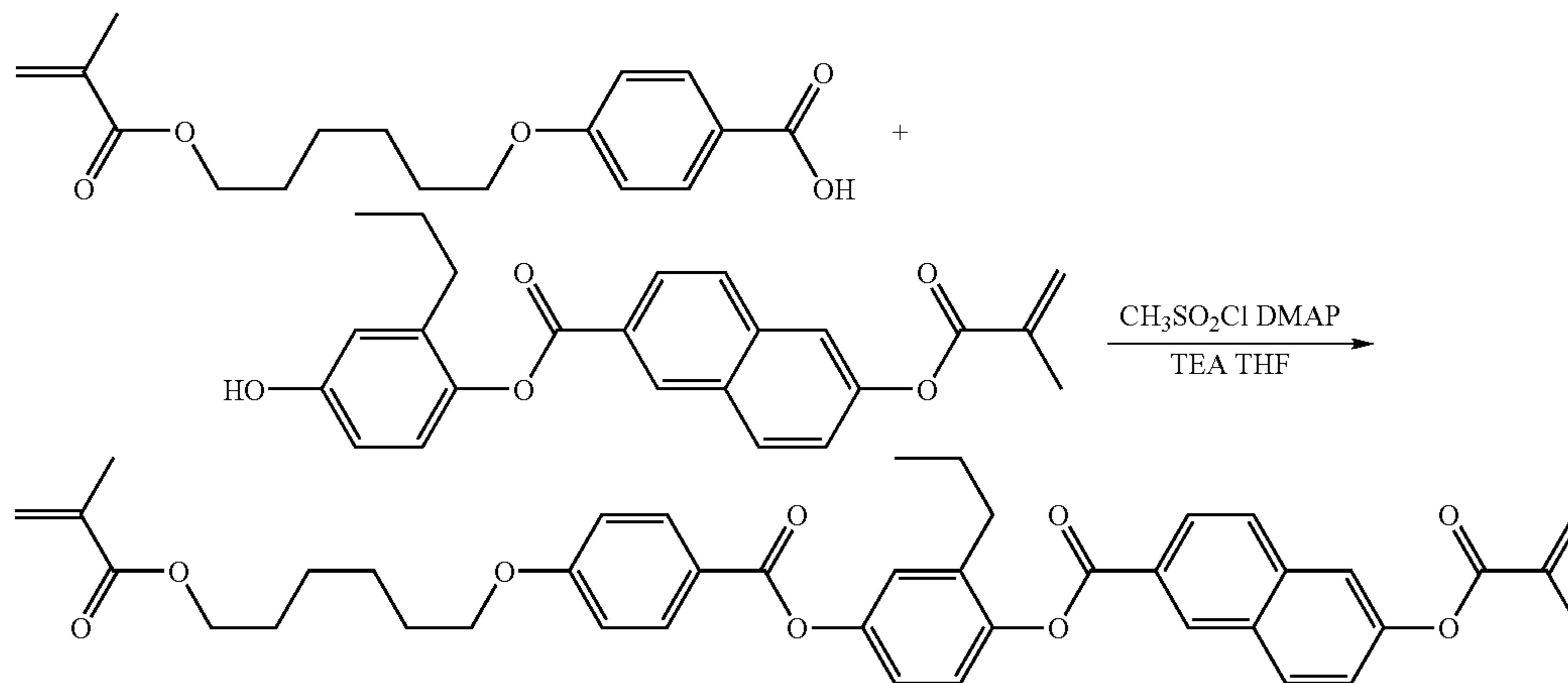
{Reaction Scheme 3}
