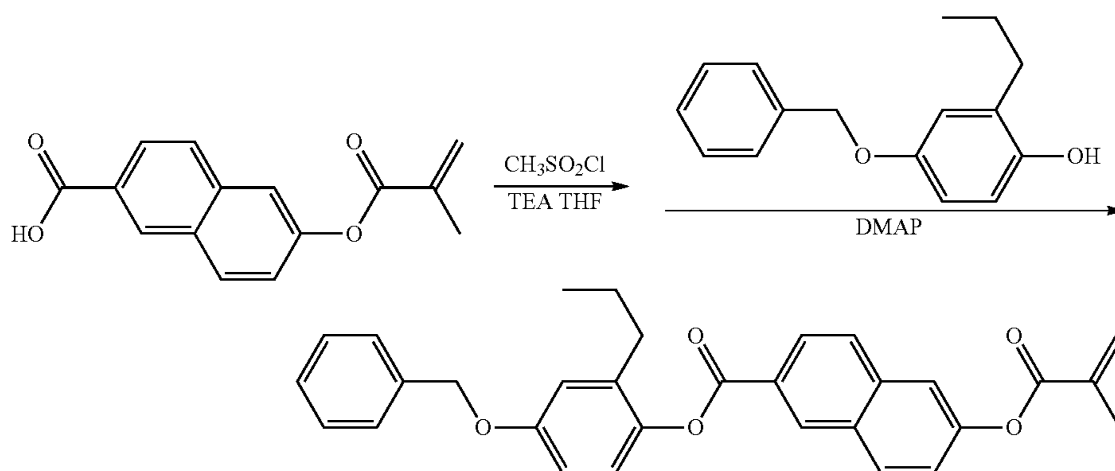
(Reaction Scheme 1)
