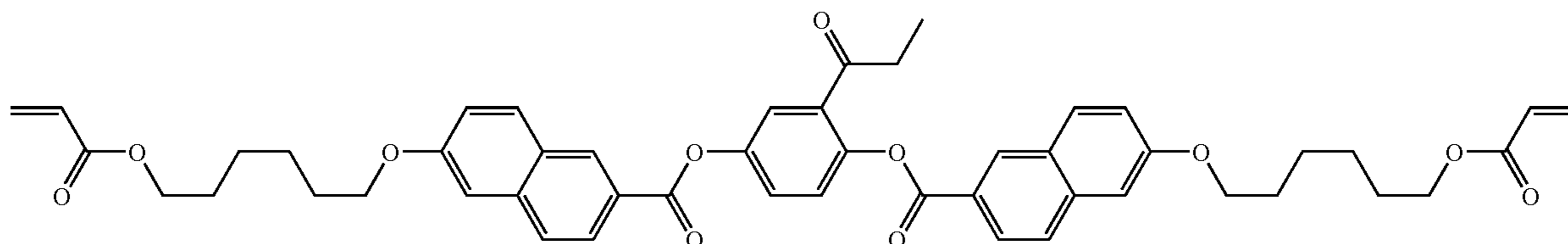
Polymerizable Compound No.43
