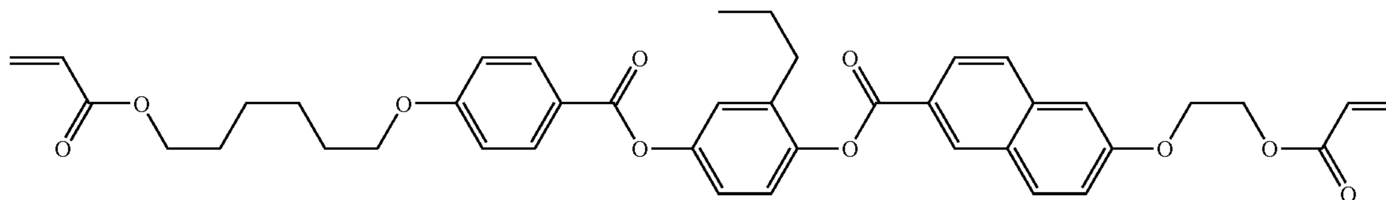
Polymerizable Compound No.40
