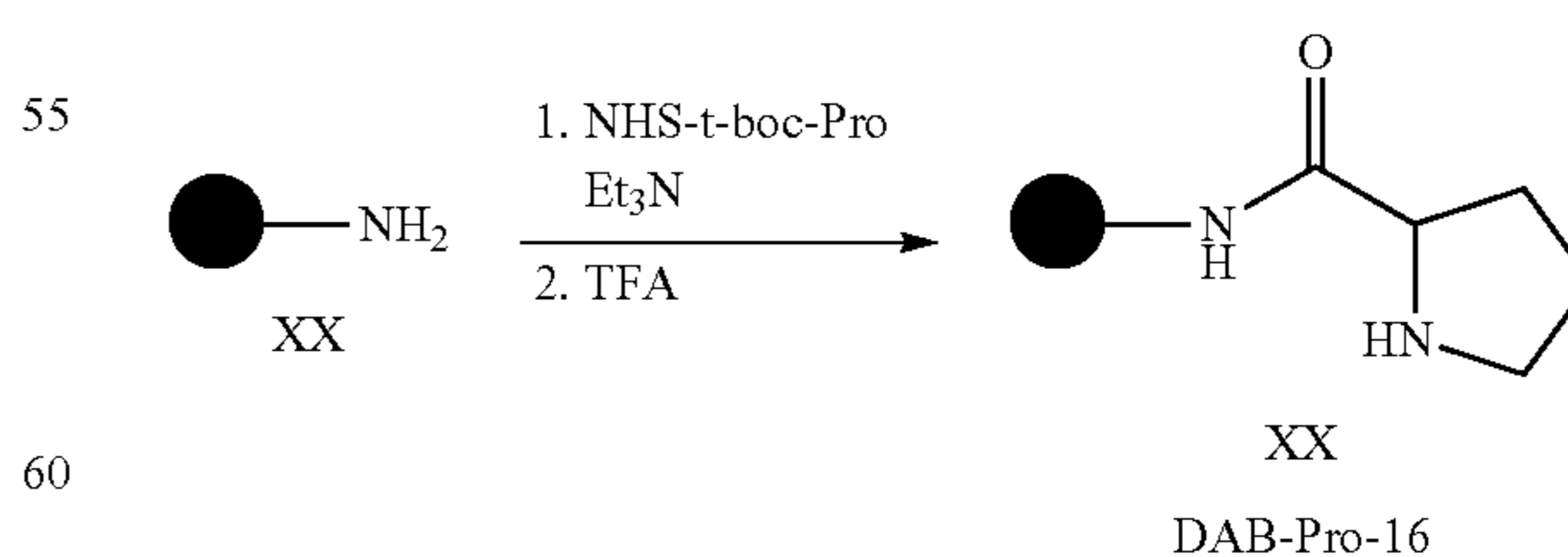
Scheme 7. Preparation of DAB-Pro-16.
