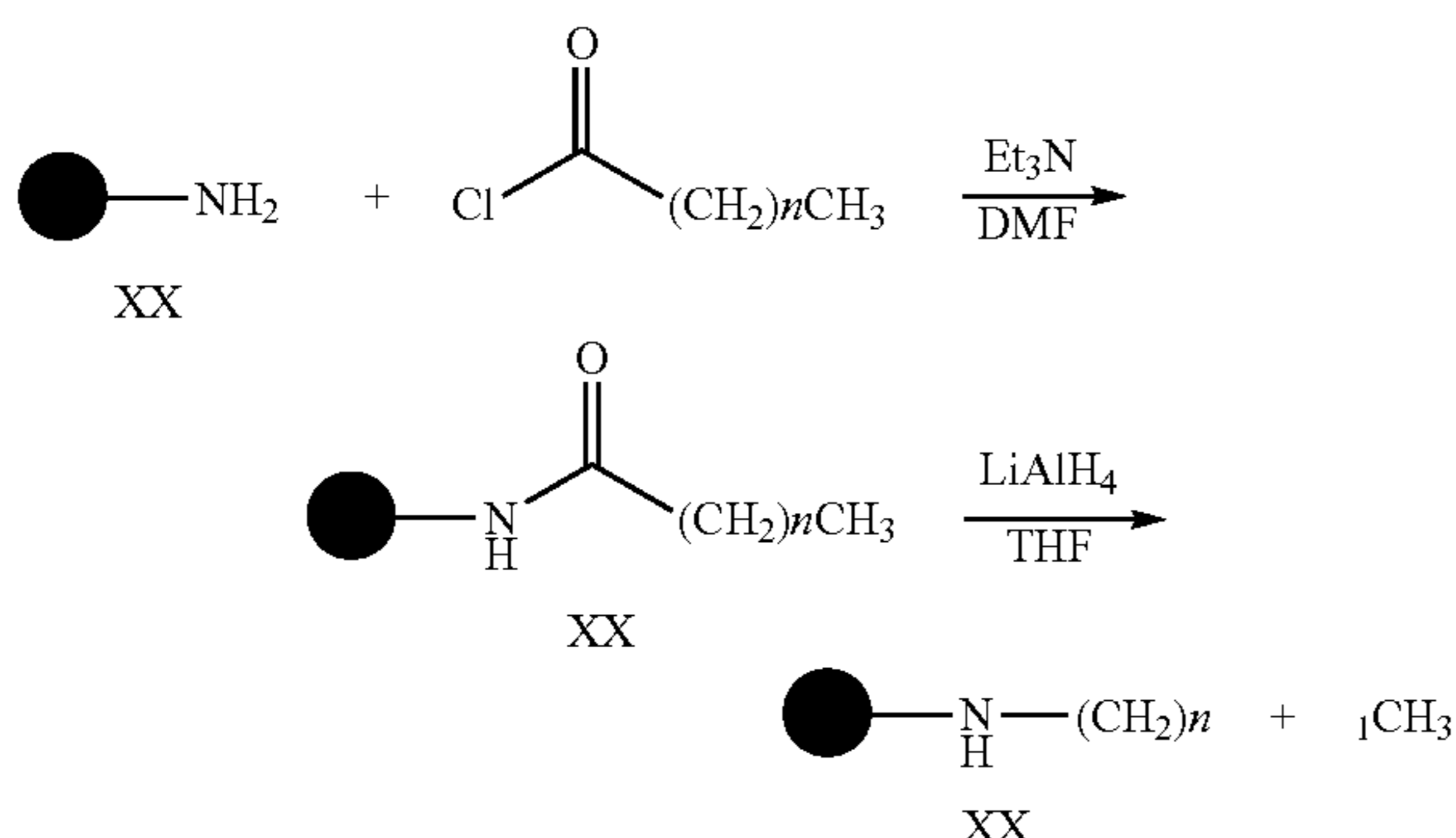
Scheme 3. General procedure for dendrimers with lipophilic tails.
