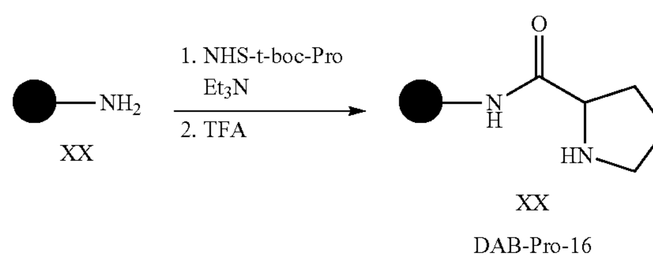
Scheme 7. Preparation of DAB-Pro-16.
