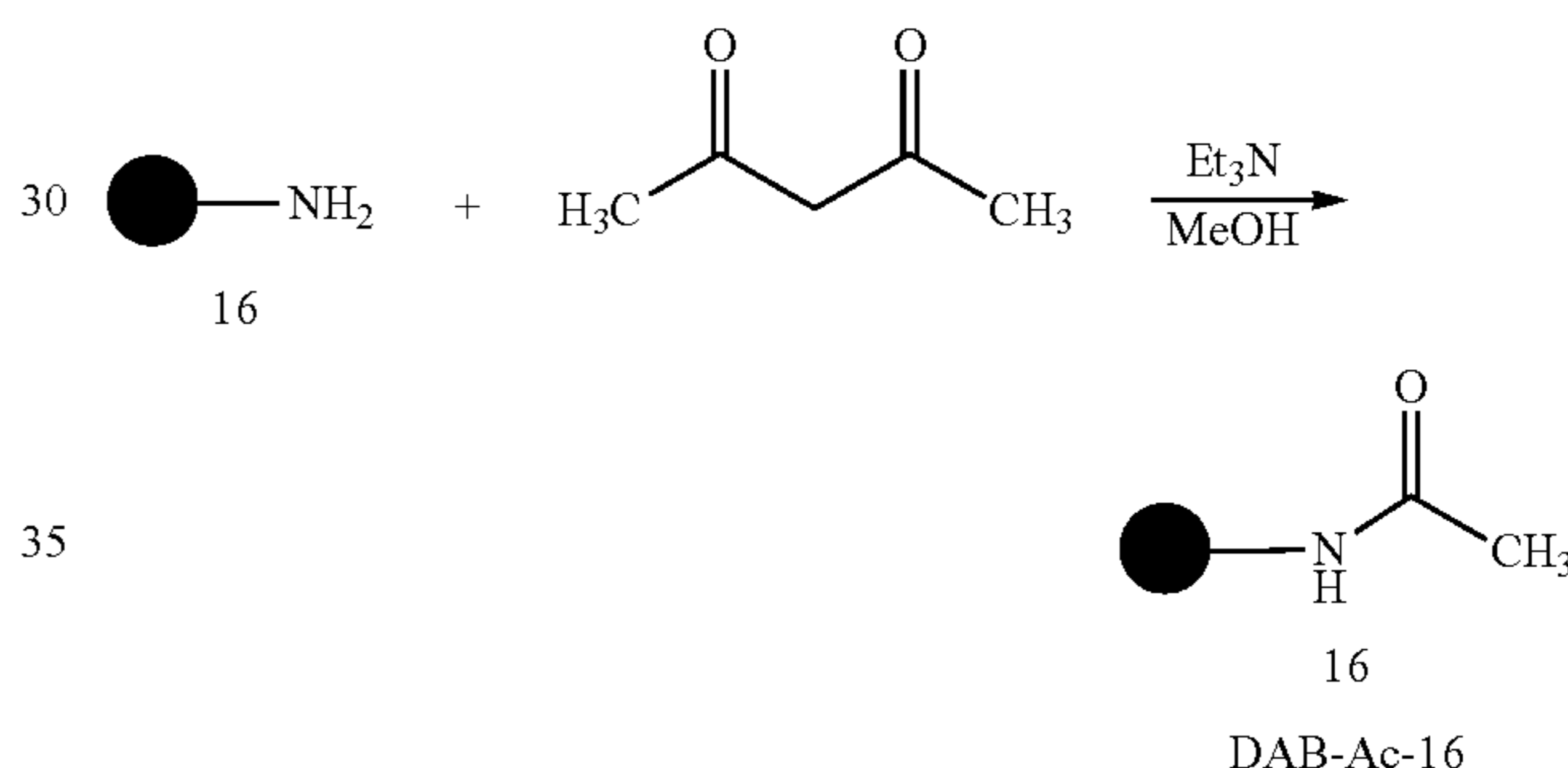
Scheme 6. Preparation of DAB-Ac-16.
