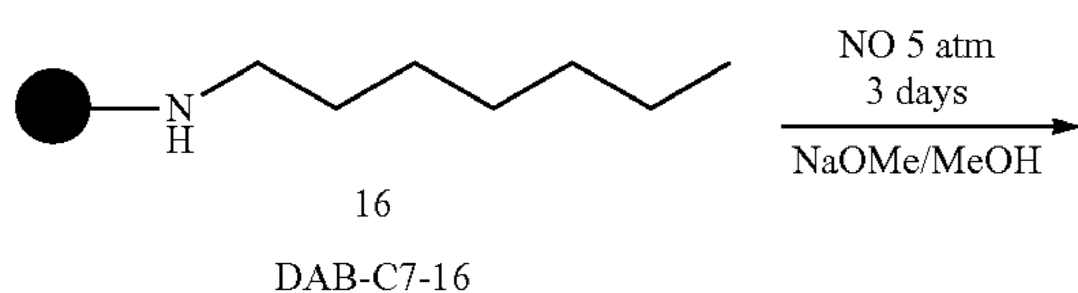
Scheme 5. Preparation of DAB-C7-16 diazeniumdiolate.
