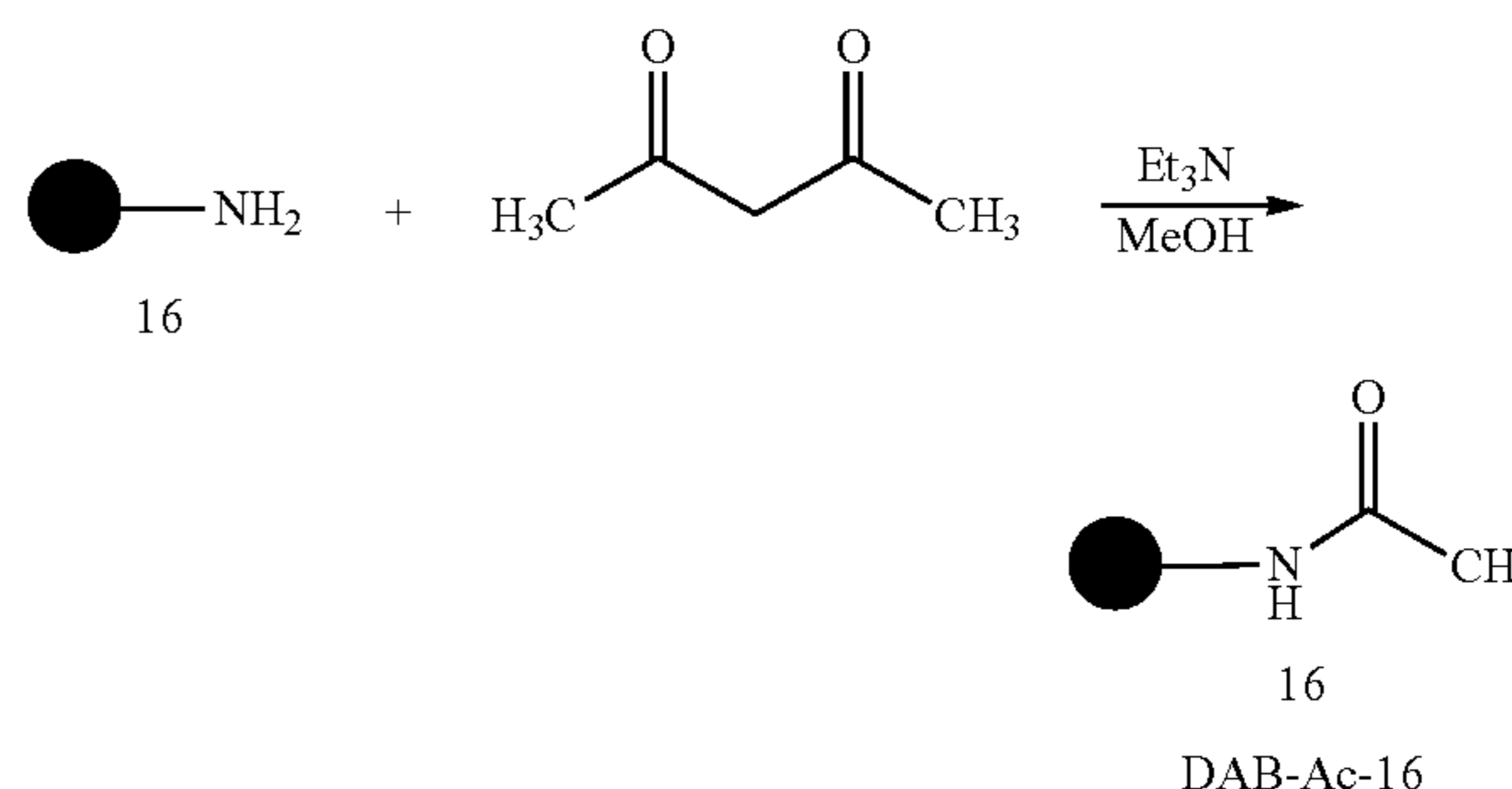
Scheme 6. Preparation of DAB-Ac-16.
