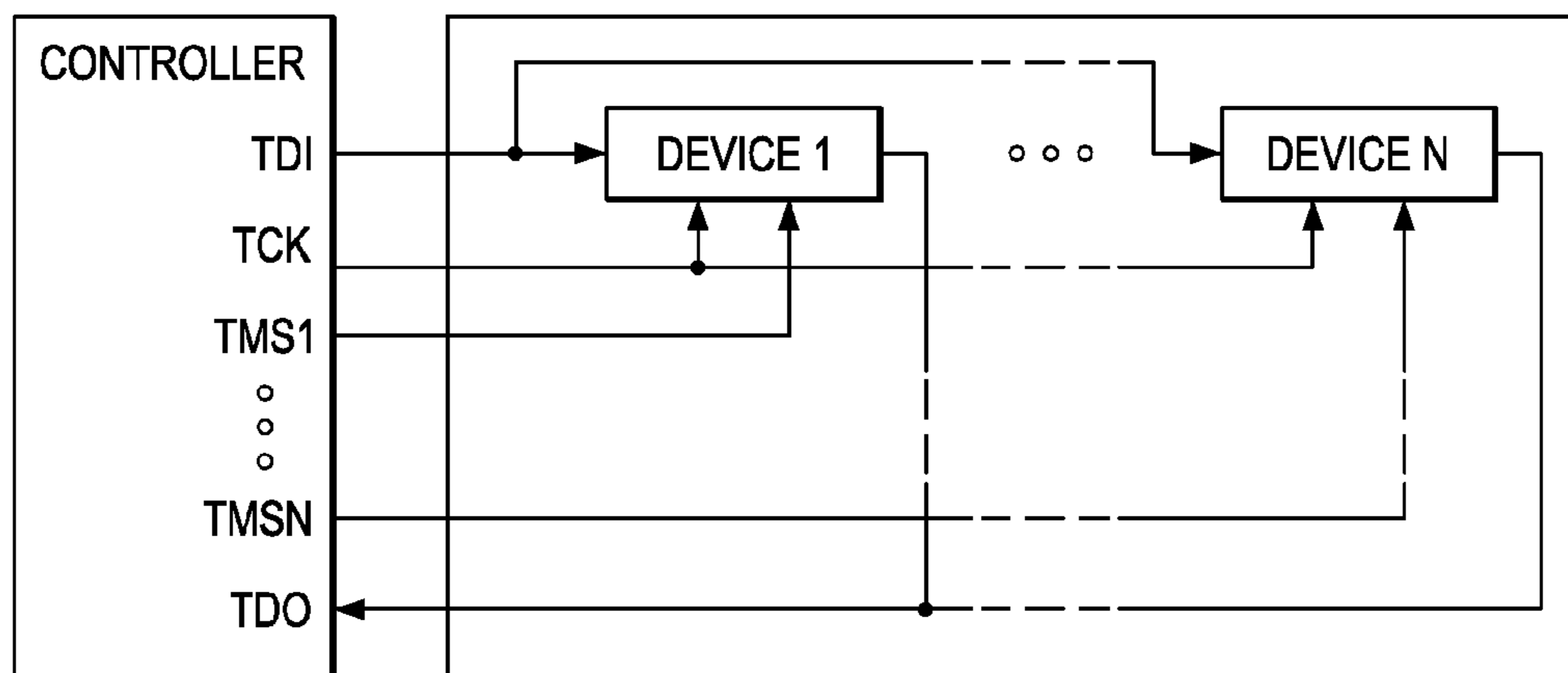
FIG. 5 (PRIOR ART)
