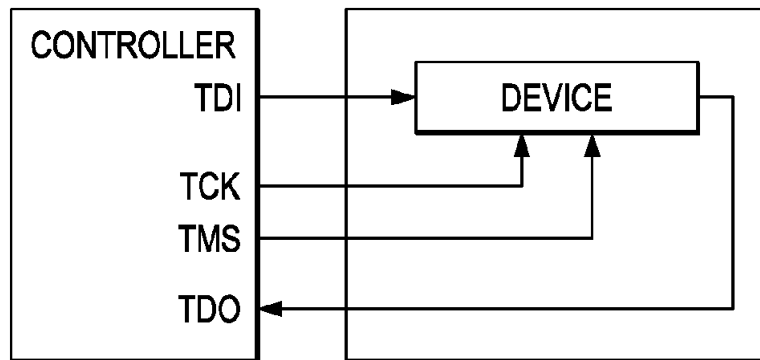
FIG. 4 (PRIOR ART)
