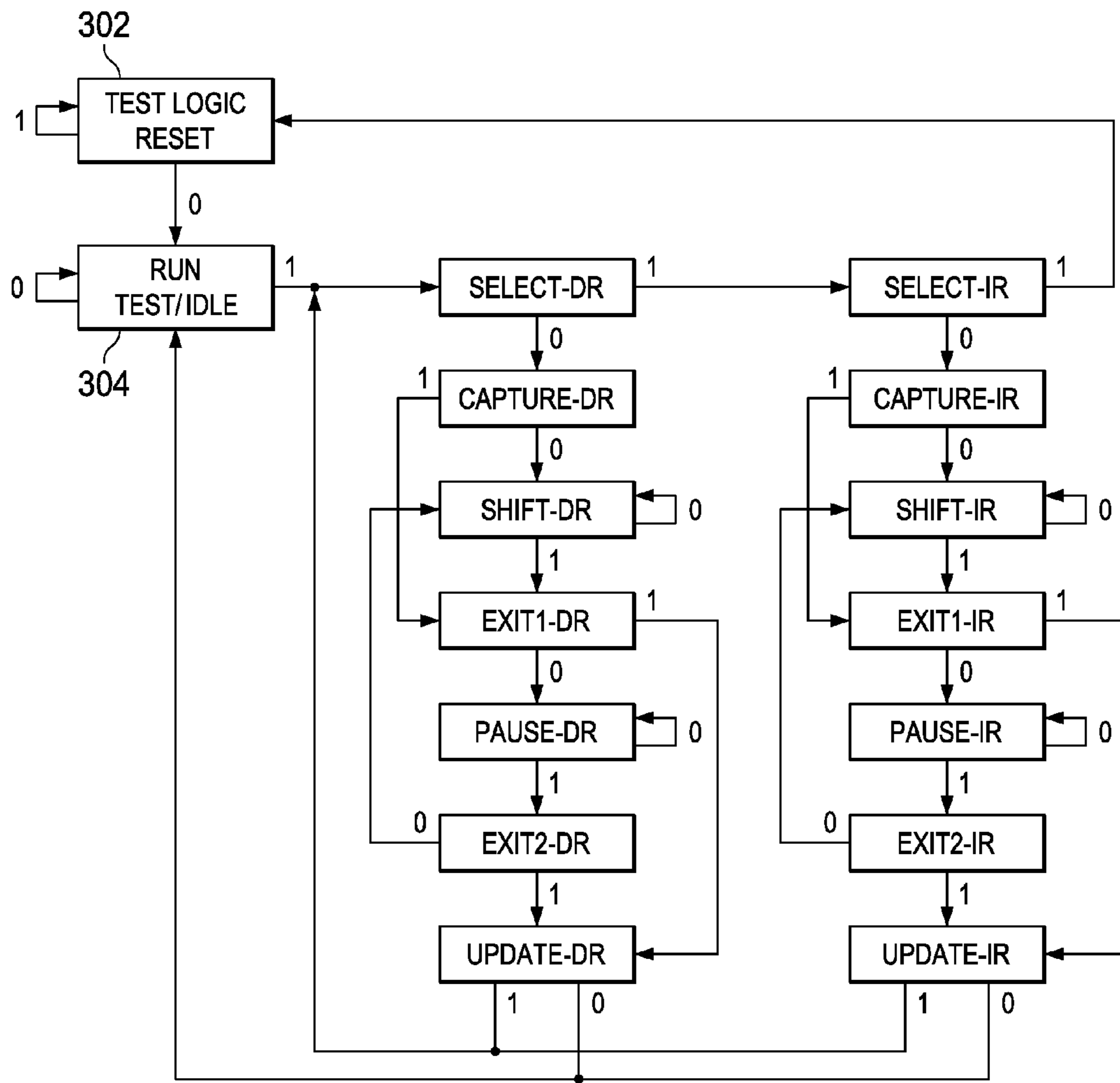
FIG. 3 (PRIOR ART)
