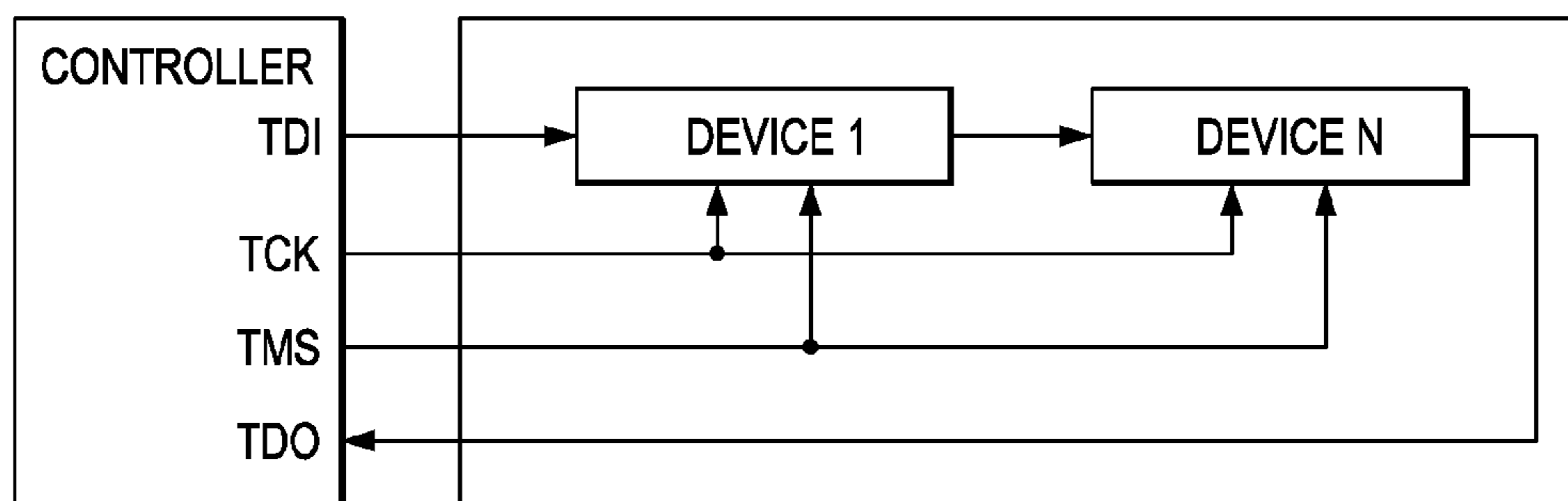
FIG. 6 (PRIOR ART)
