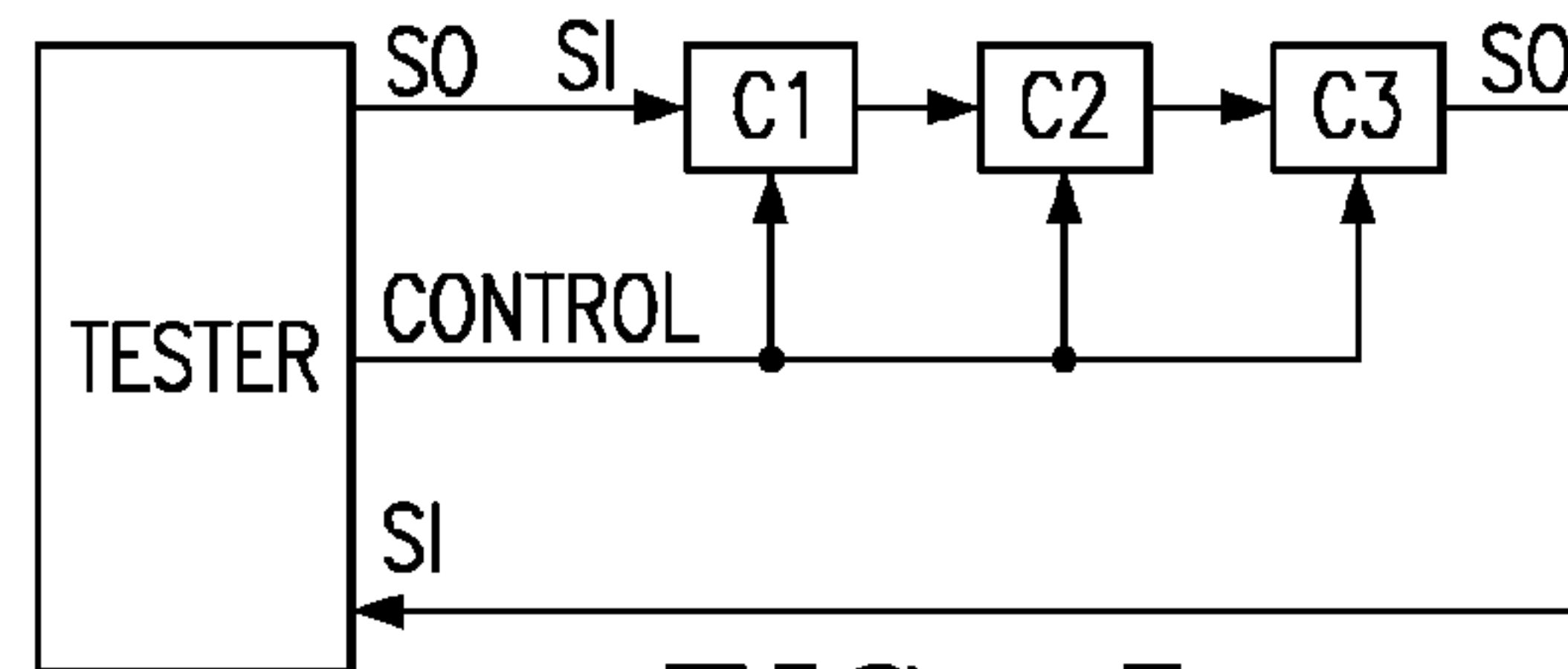
FIG. 5 (PRIOR ART)
