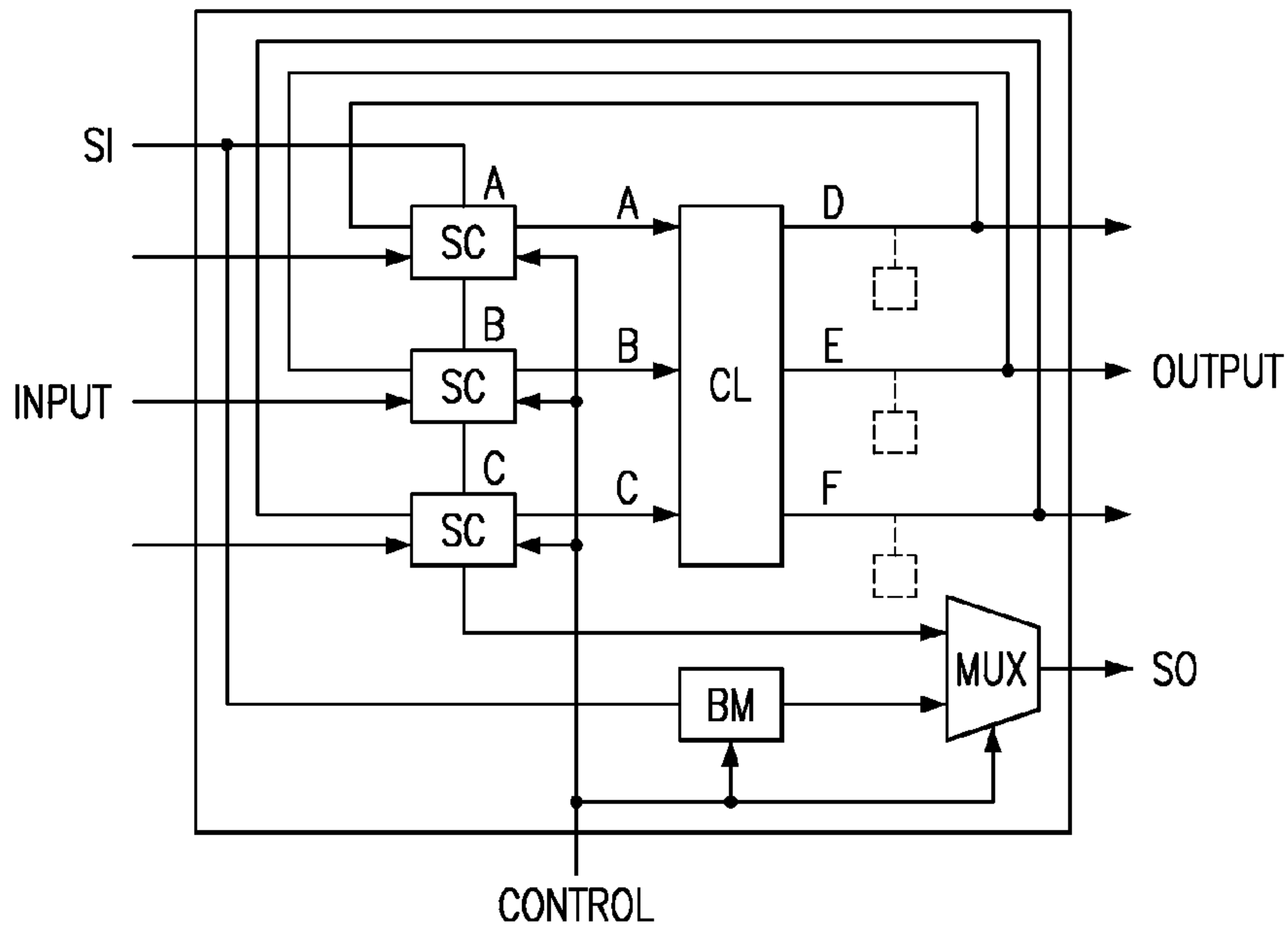
FIG. 3 (PRIOR ART)
