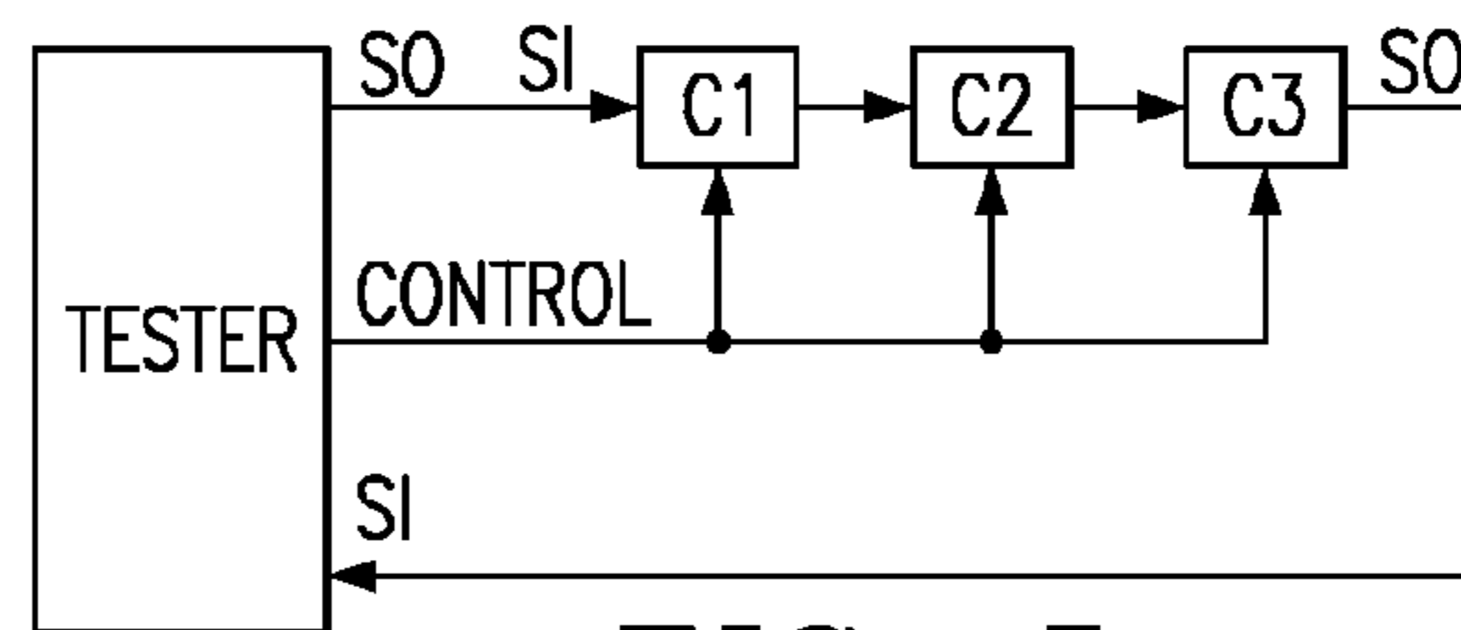
FIG. 5 (PRIOR ART)
