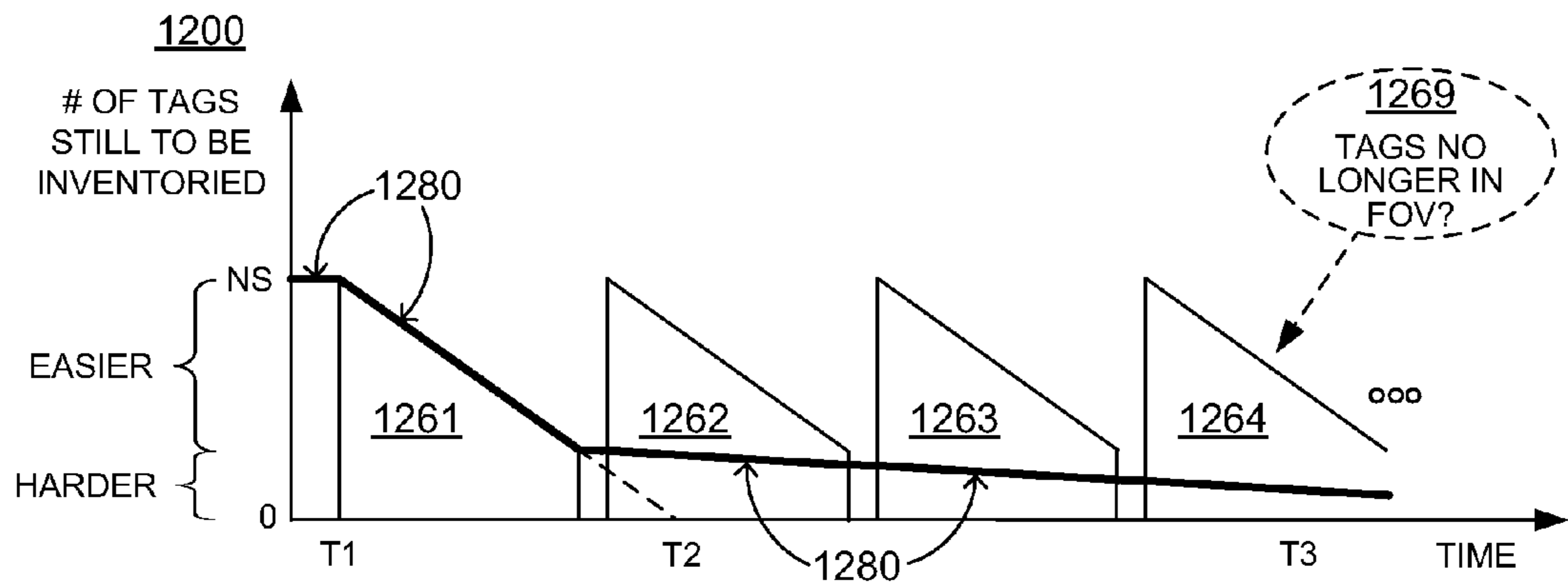
FIG. 12 INVENTORYING TAGS - SOME HARDER TO READ THAN OTHERS (PRIOR ART)
