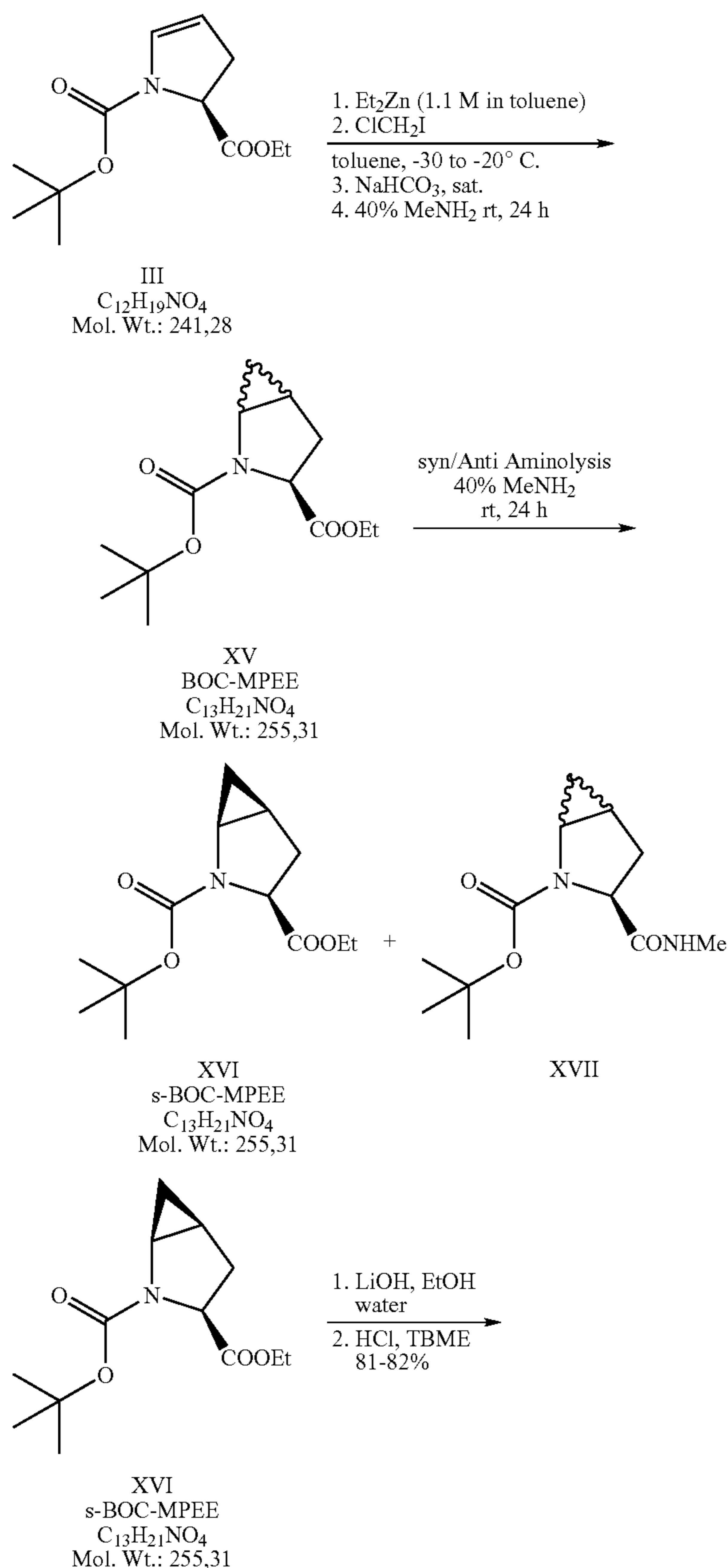
SCHEME VIA
