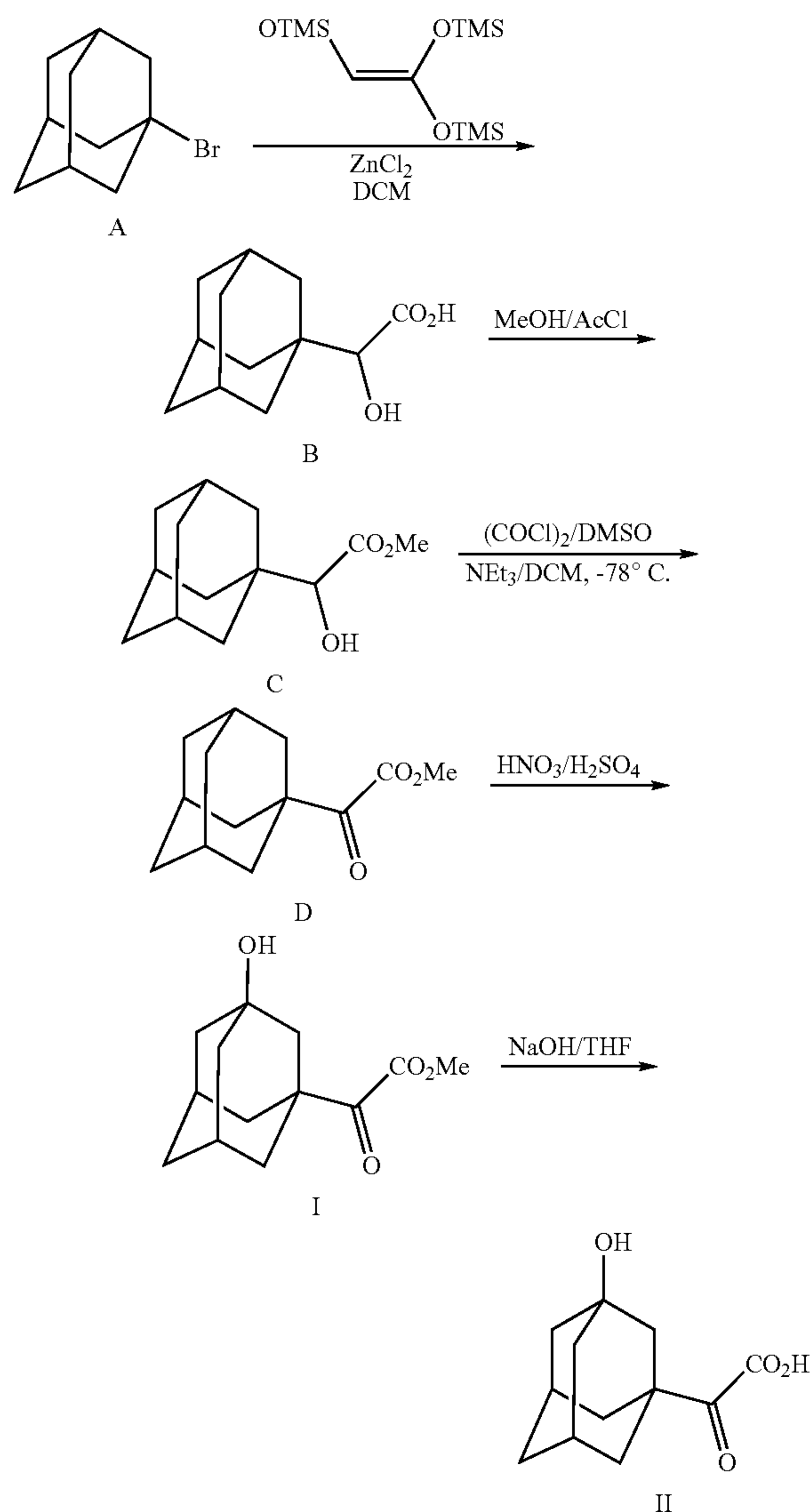
SCHEME IV
