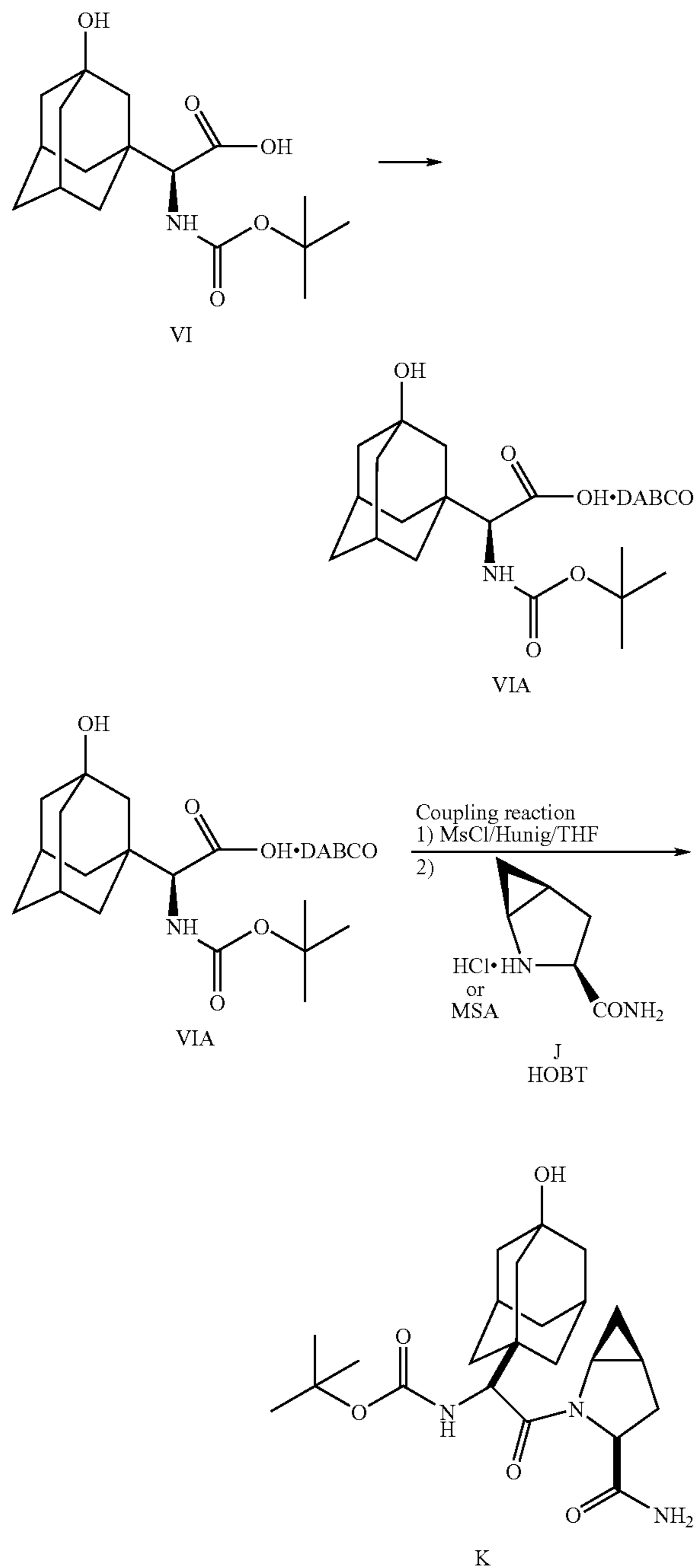
SCHEME VIIA
