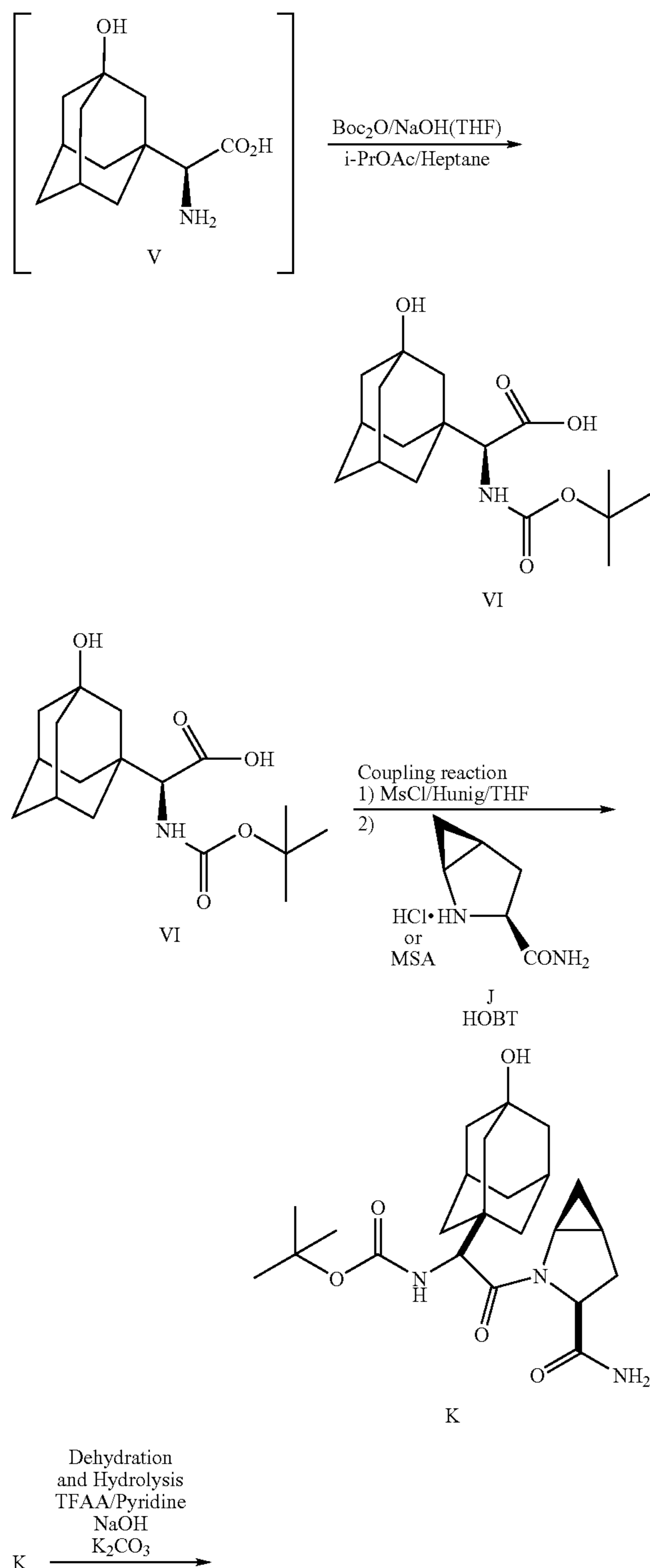
SCHEME VII
