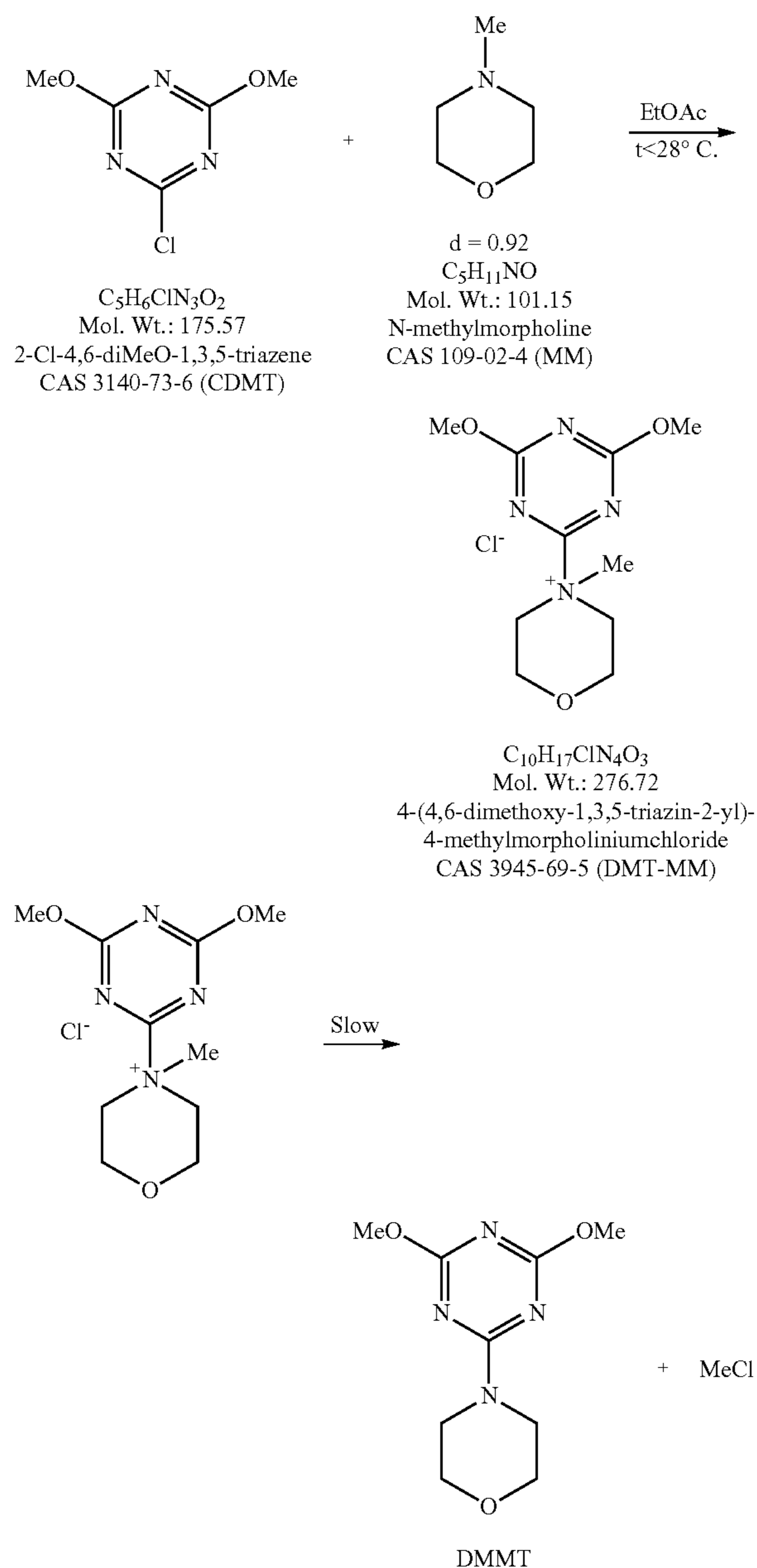
SCHEME VIA
