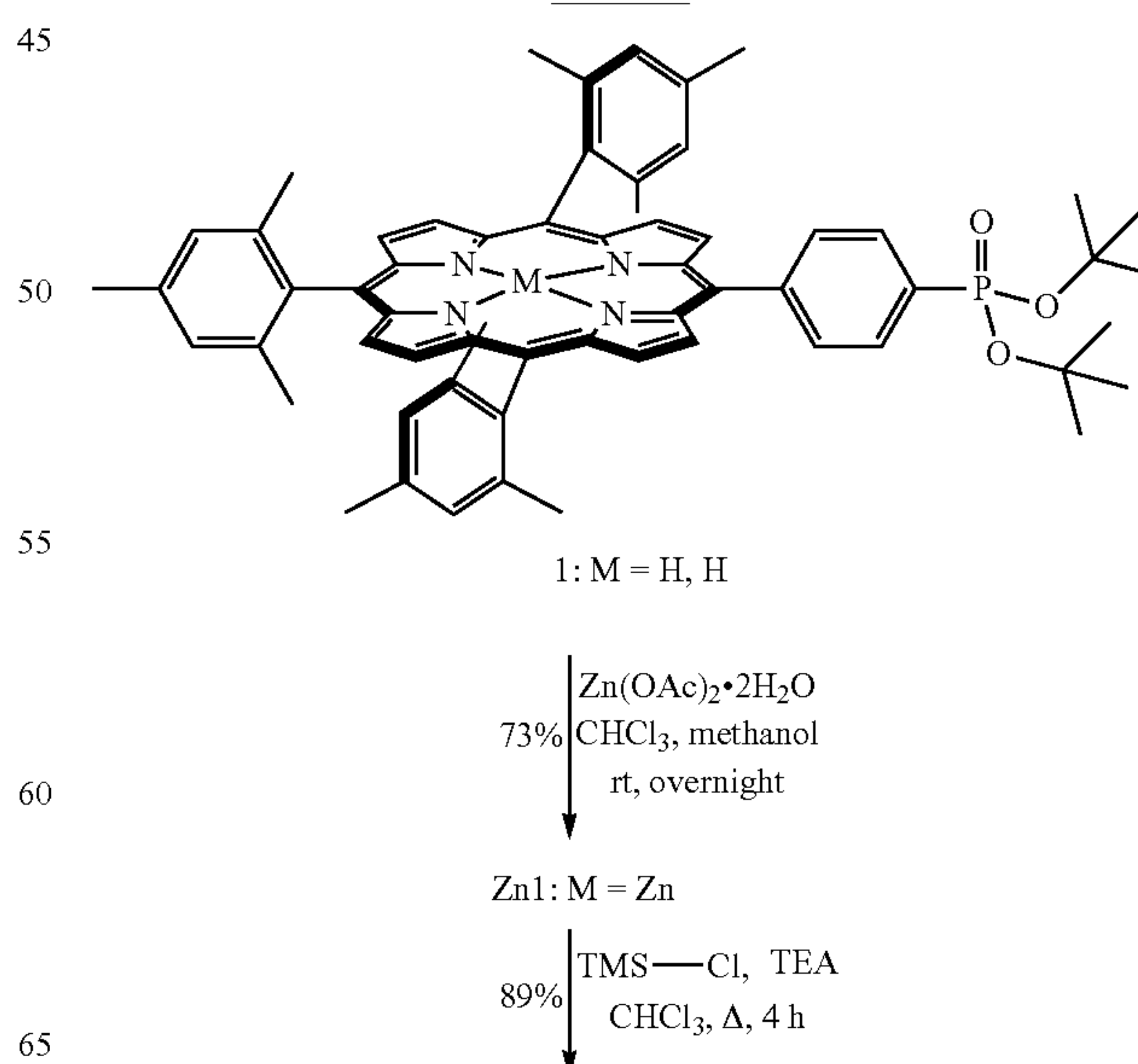
Scheme 1
