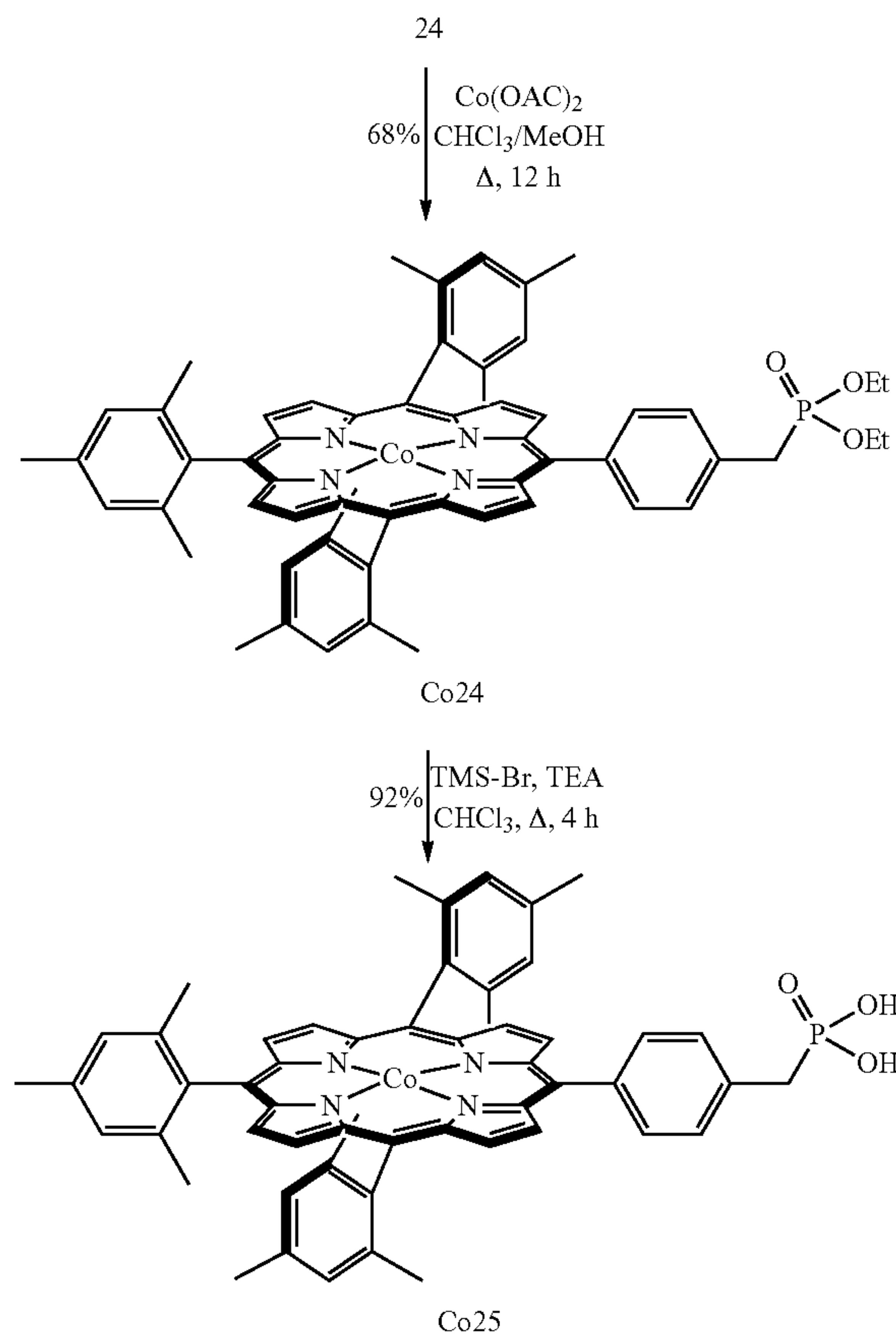
Scheme 14
