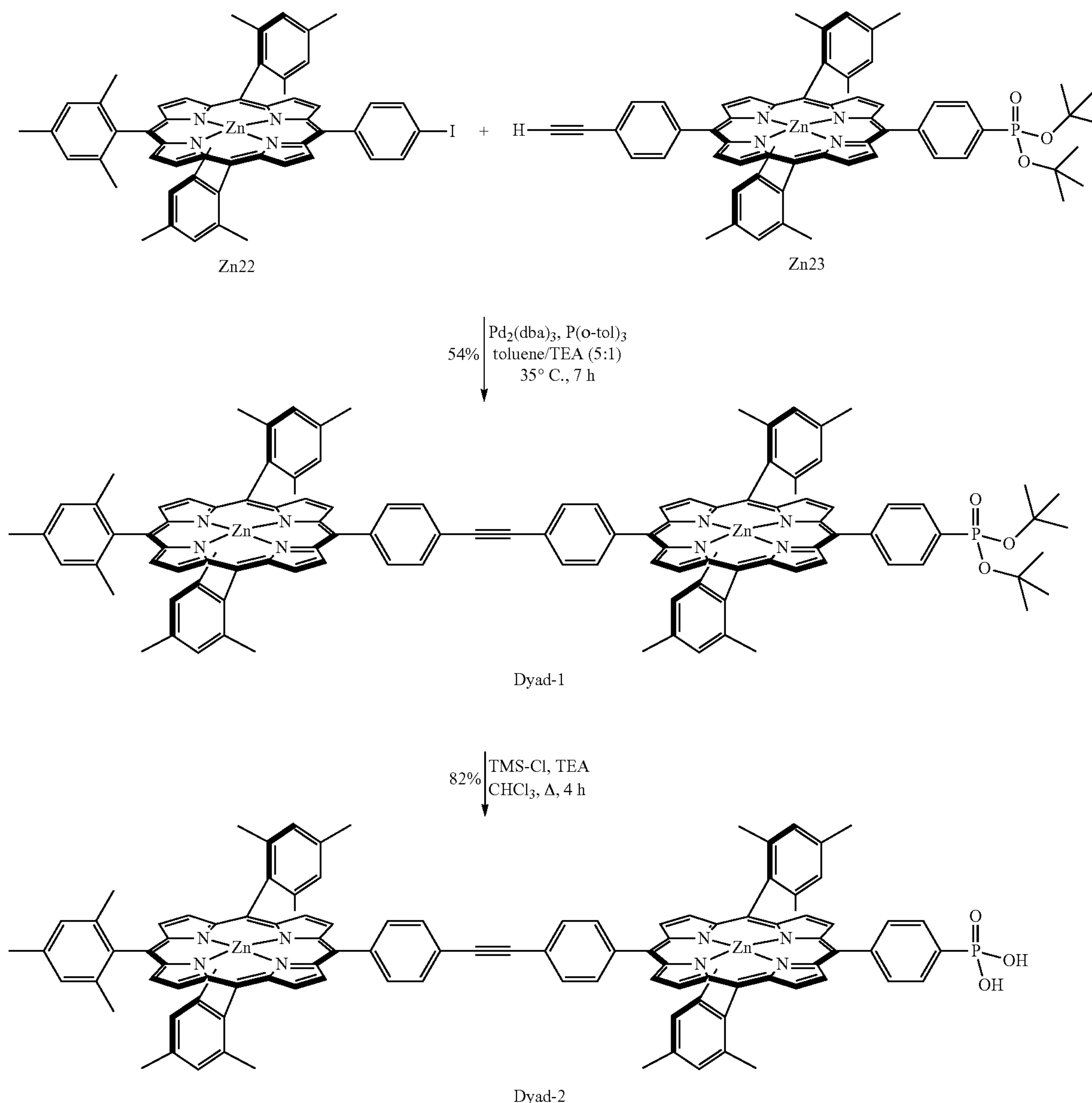
Scheme 9
