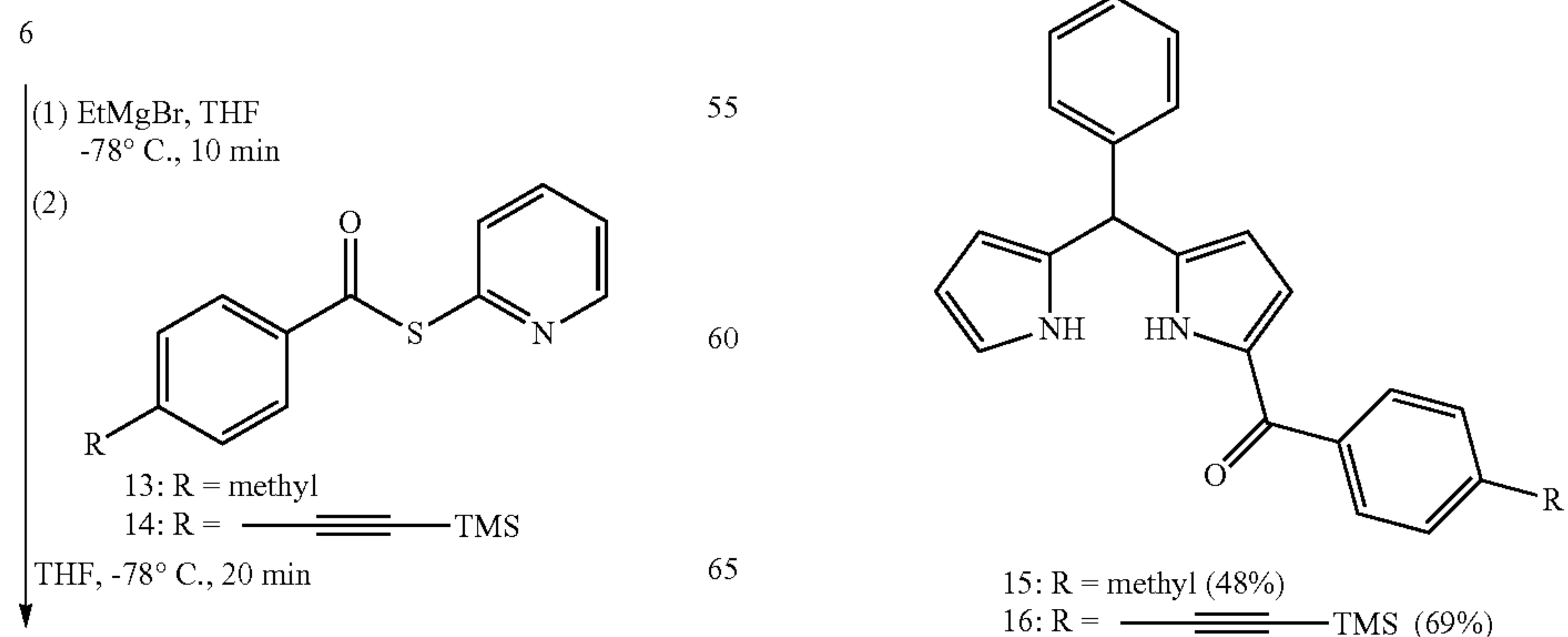
Scheme 6
