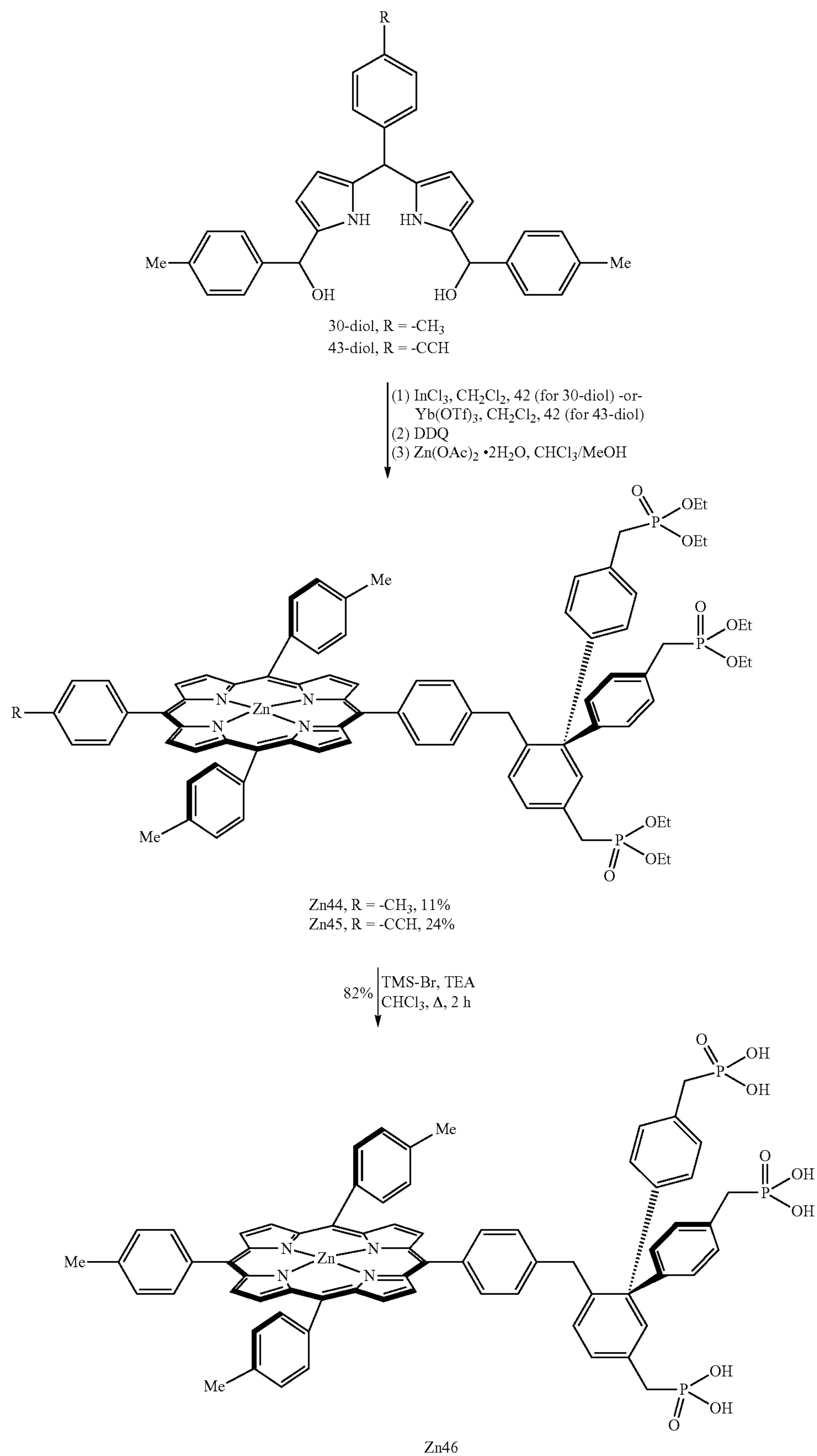
Scheme 16
