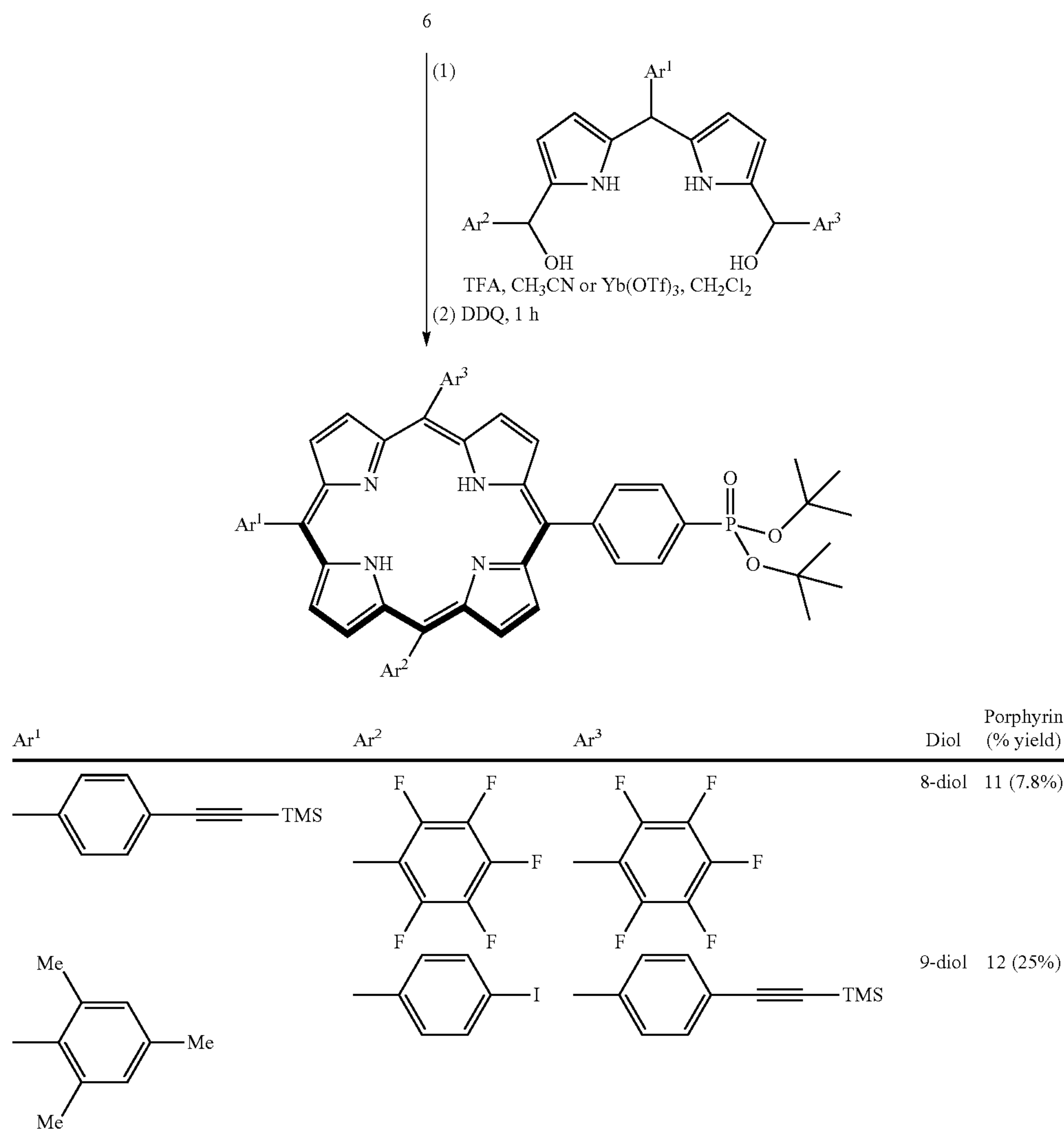
Scheme 5
