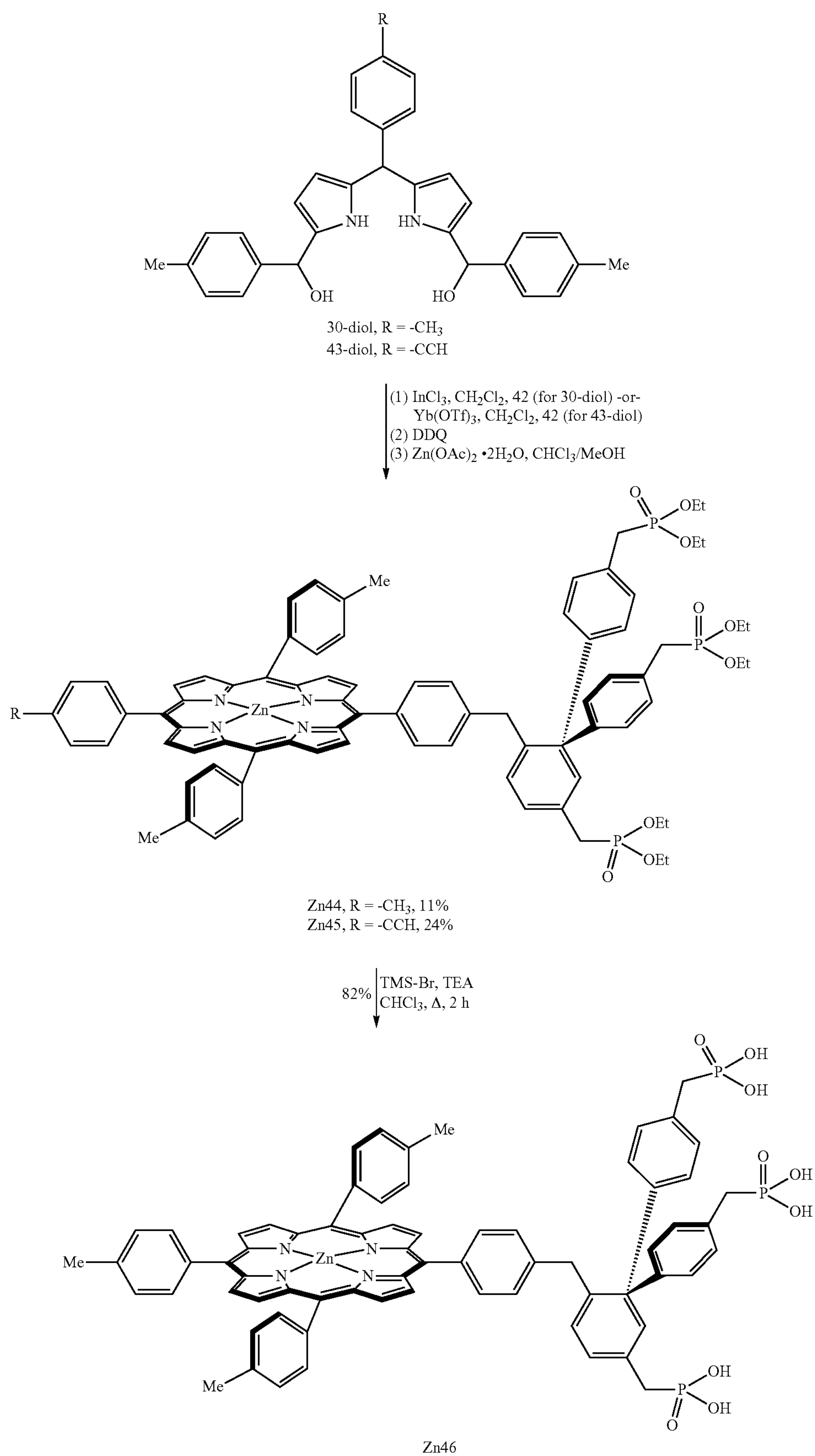
Scheme 16
