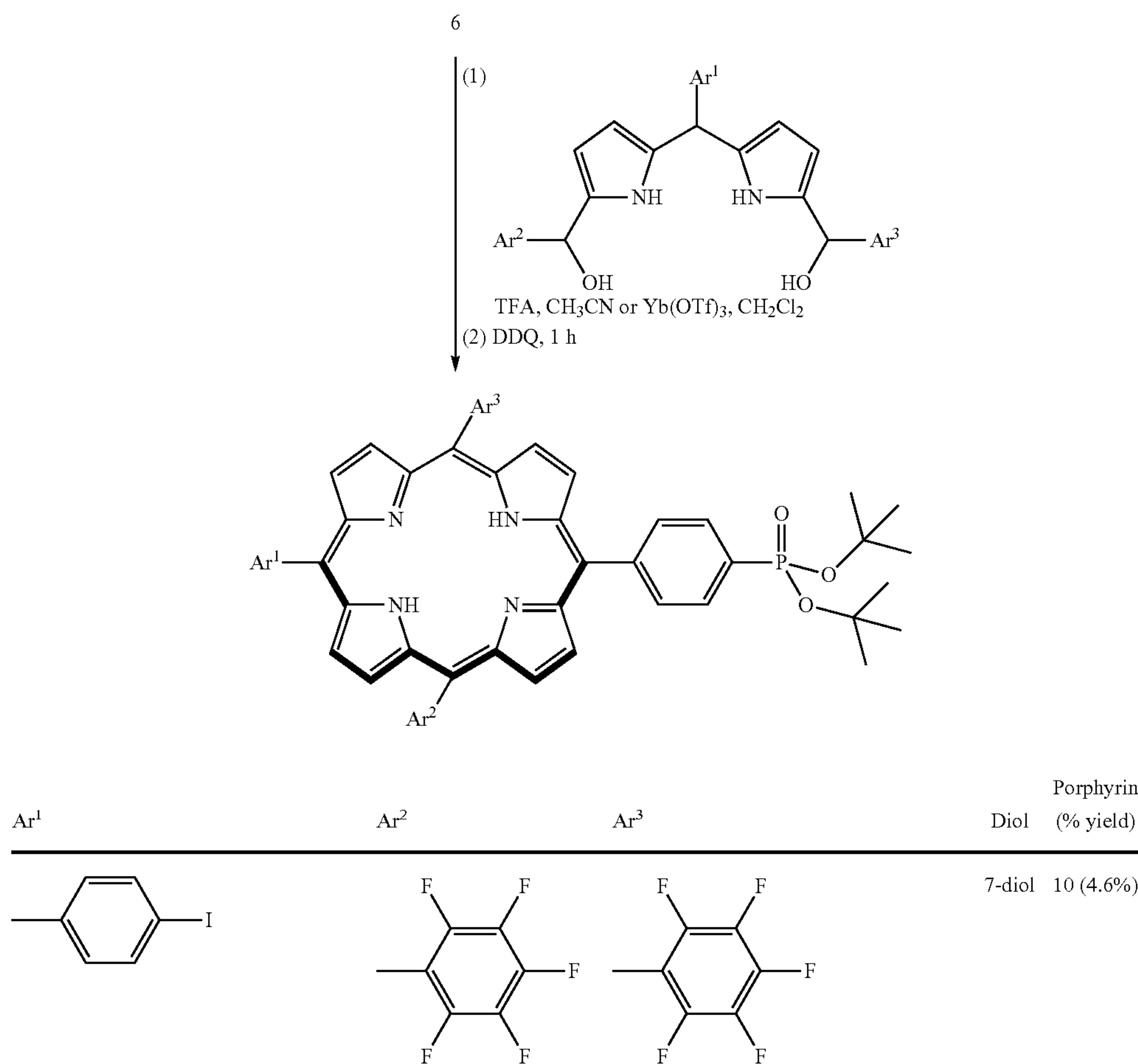
Scheme 5
