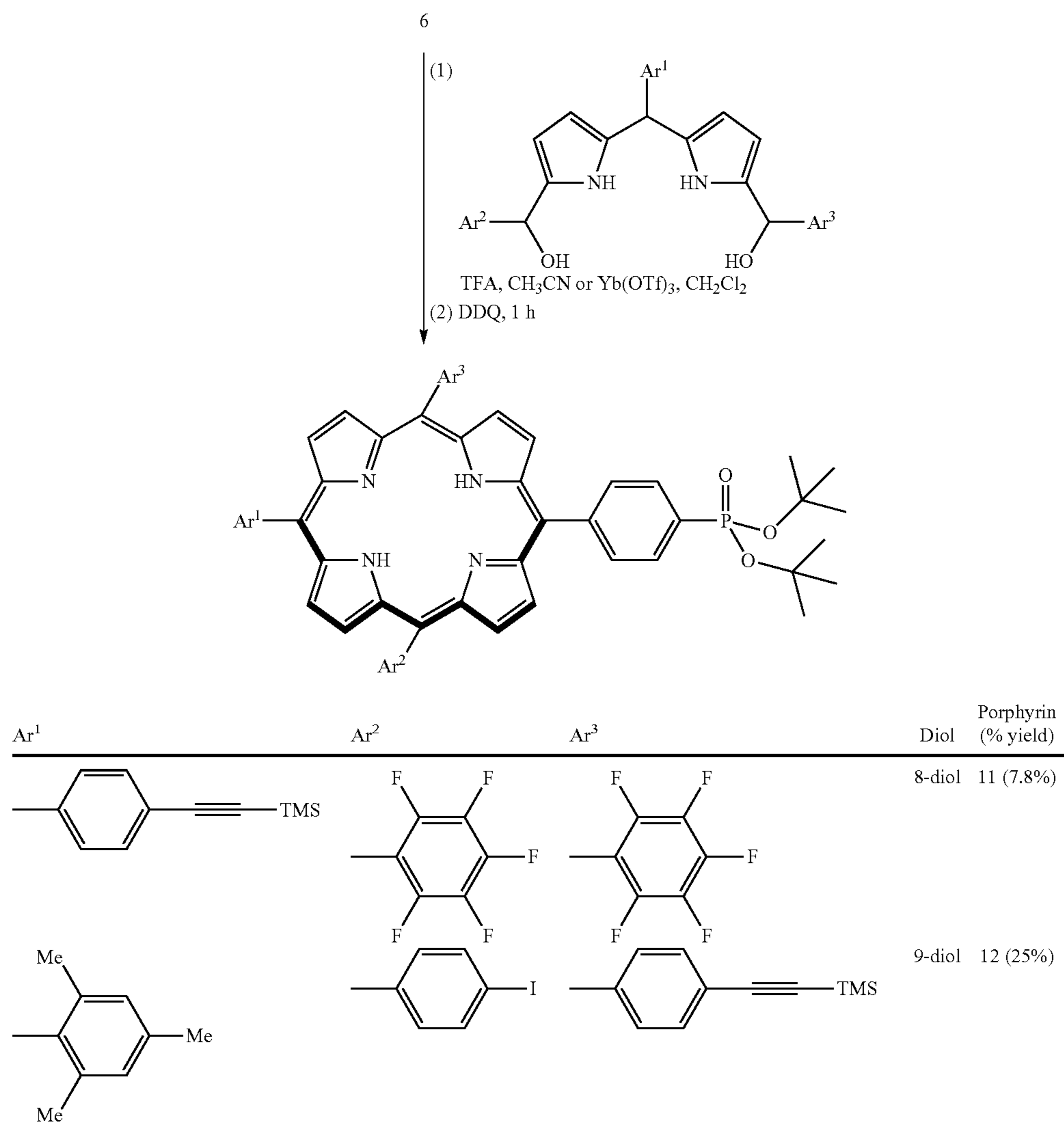
Scheme 5
