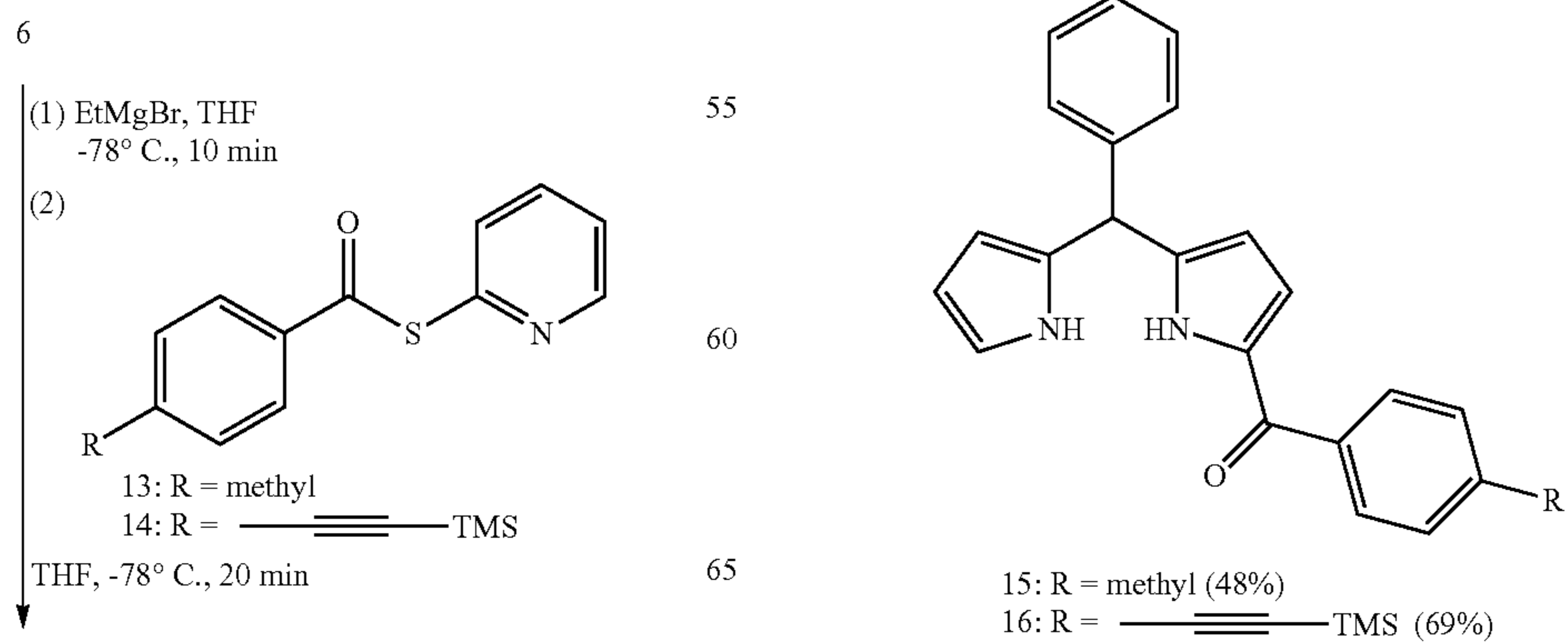
Scheme 6
