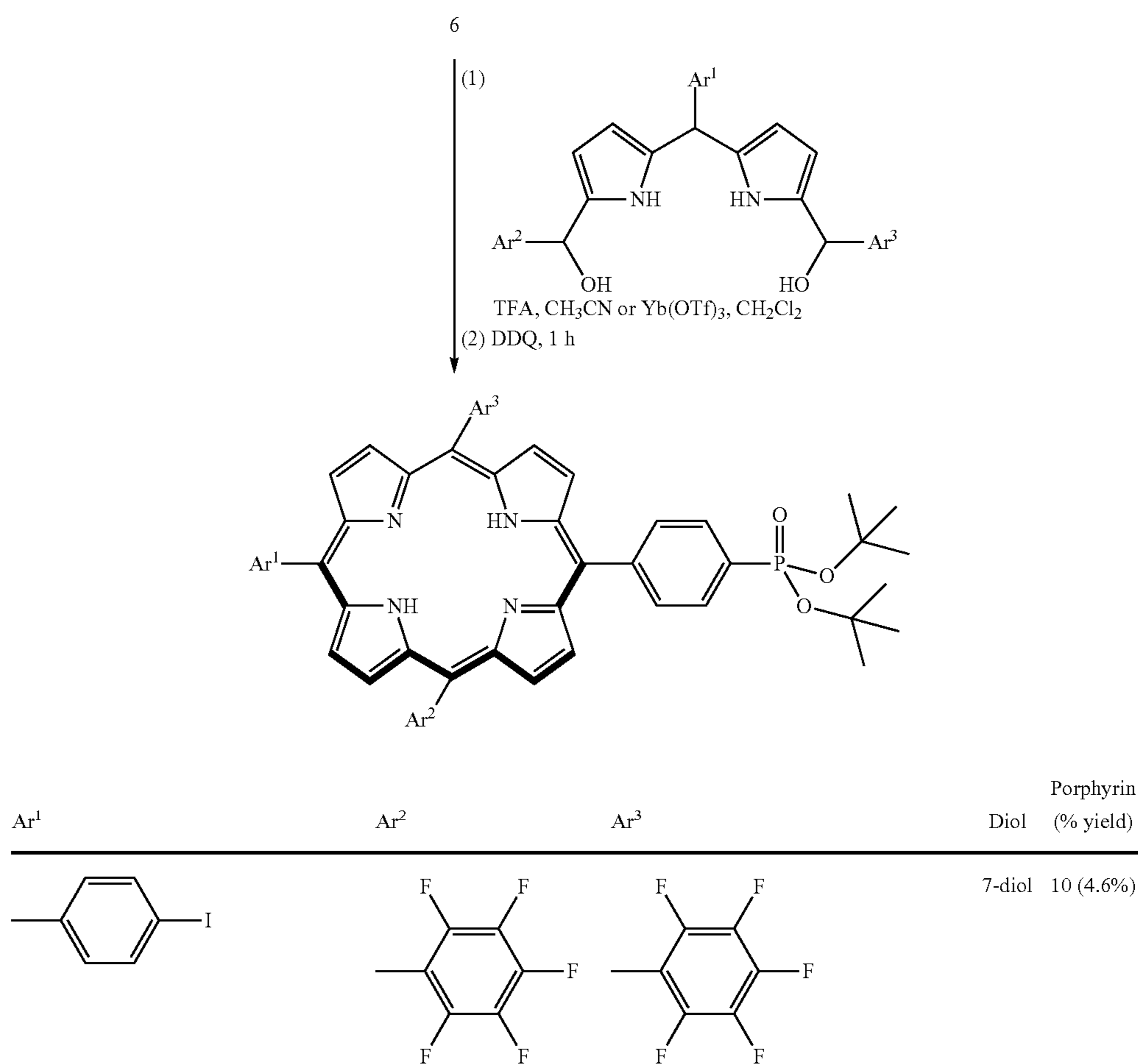
Scheme 5
