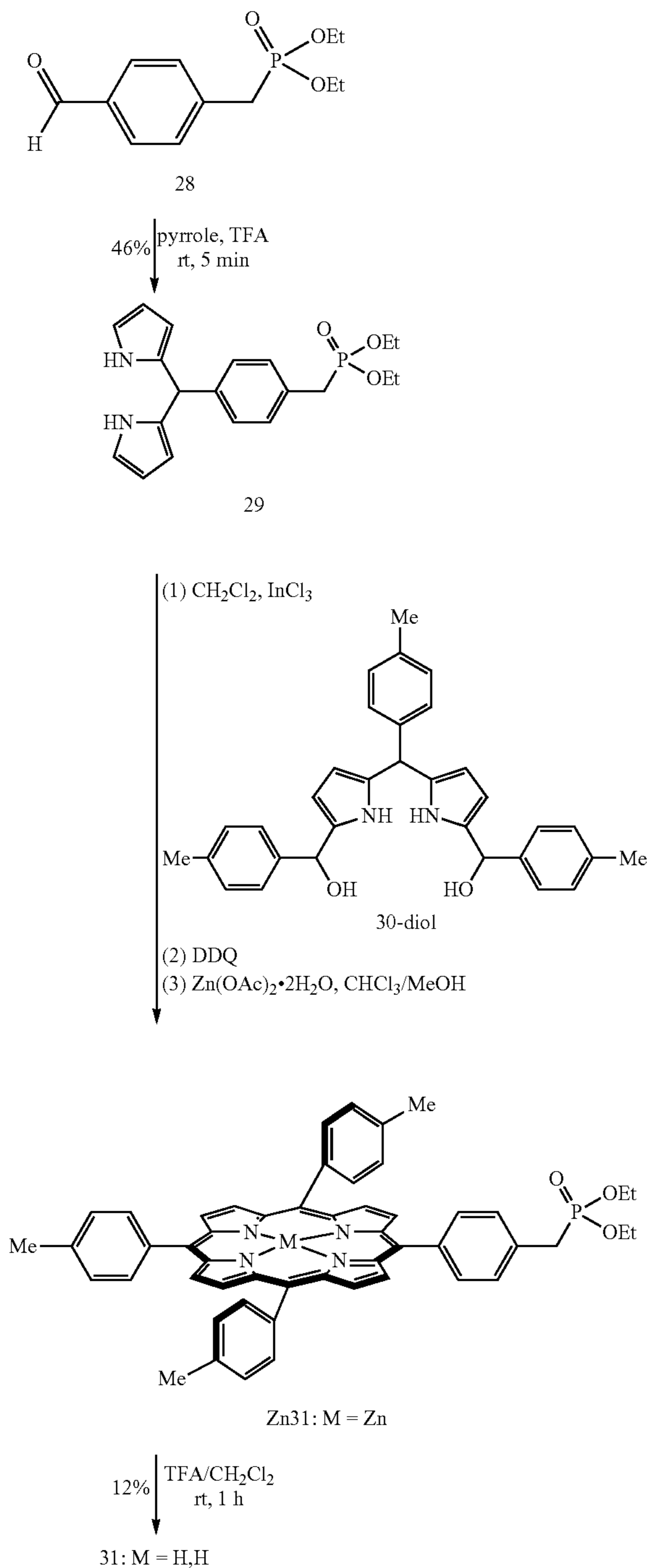
Scheme 12
