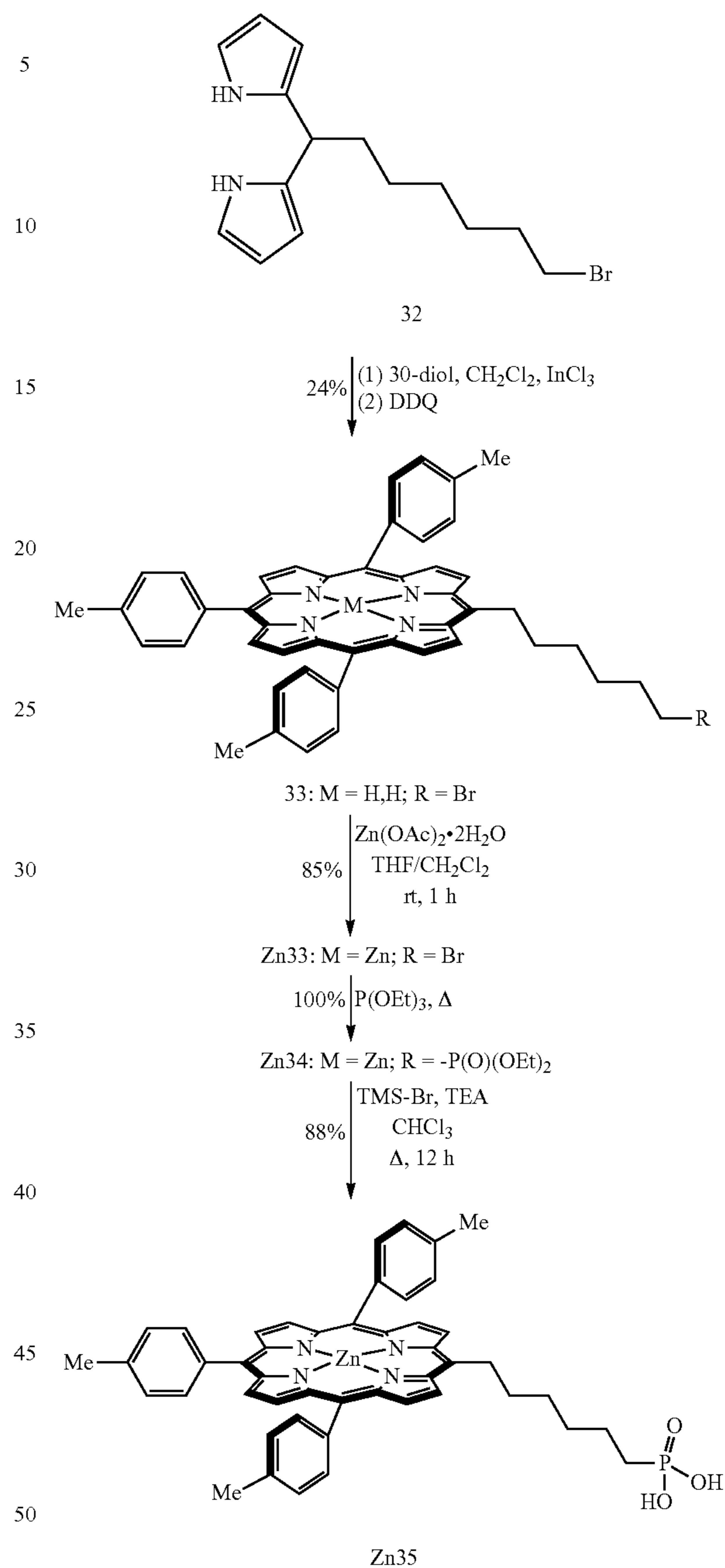
Scheme 13
