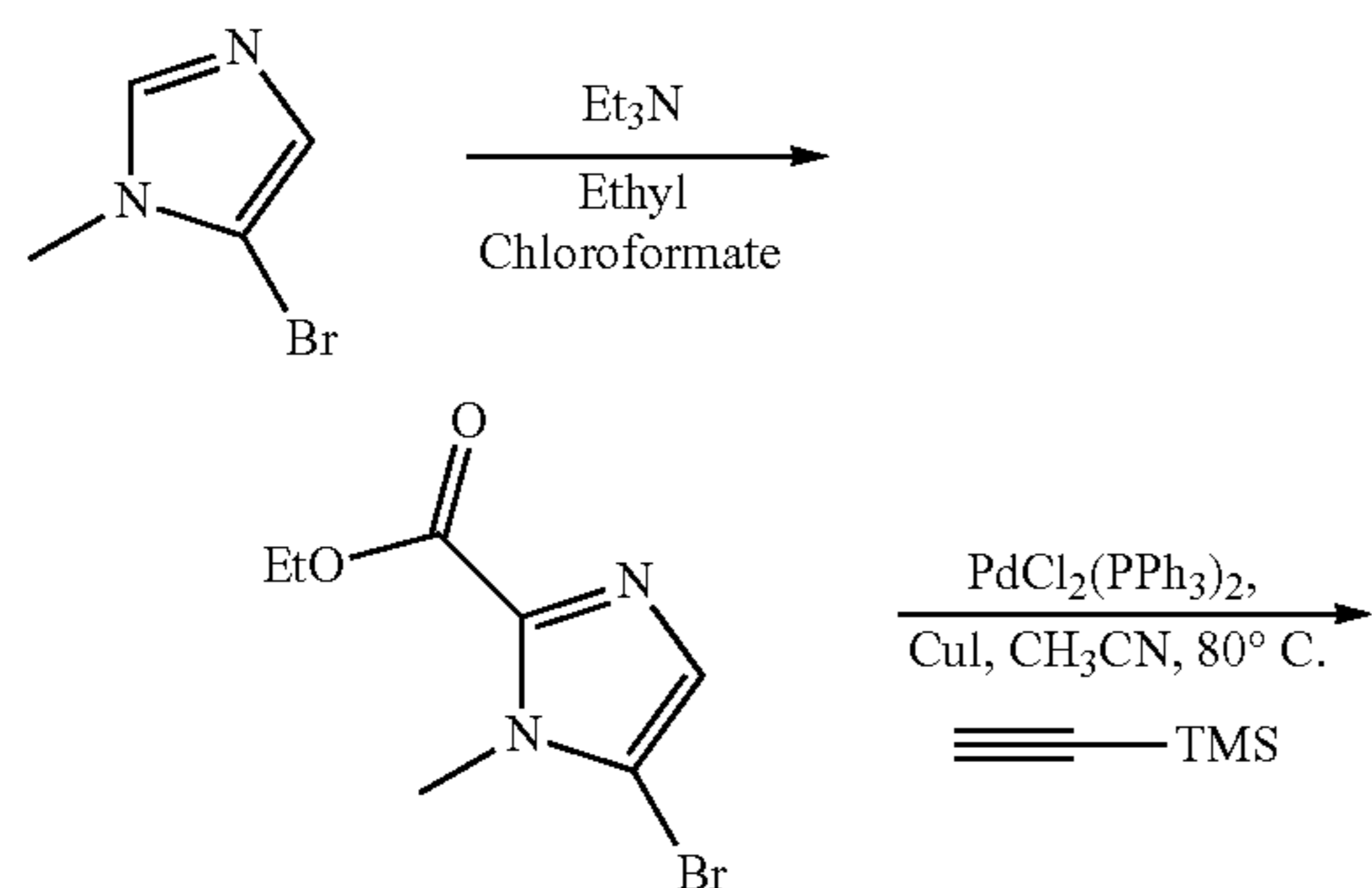
Alternative Synthesis
