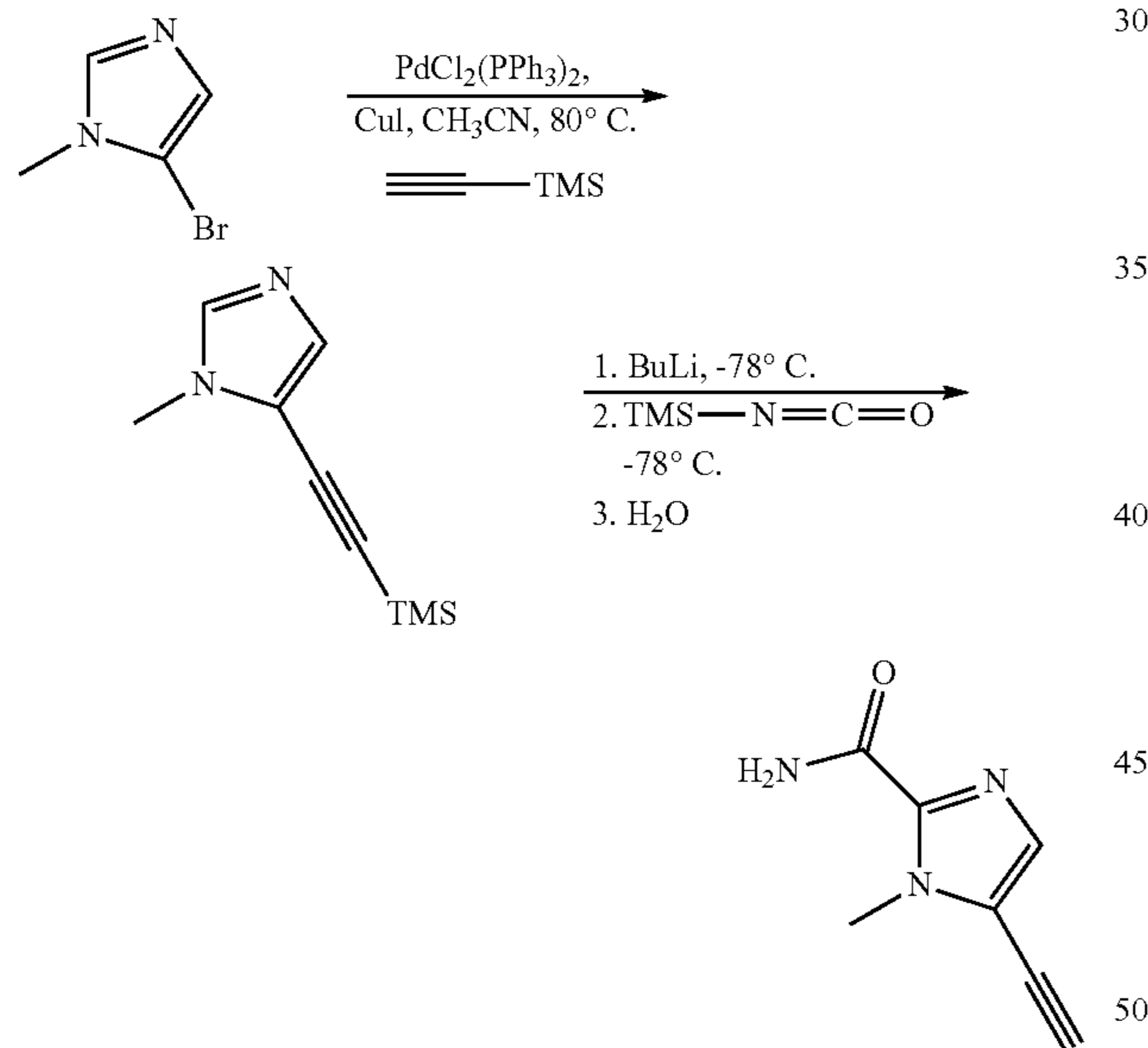
Alternative Synthesis
