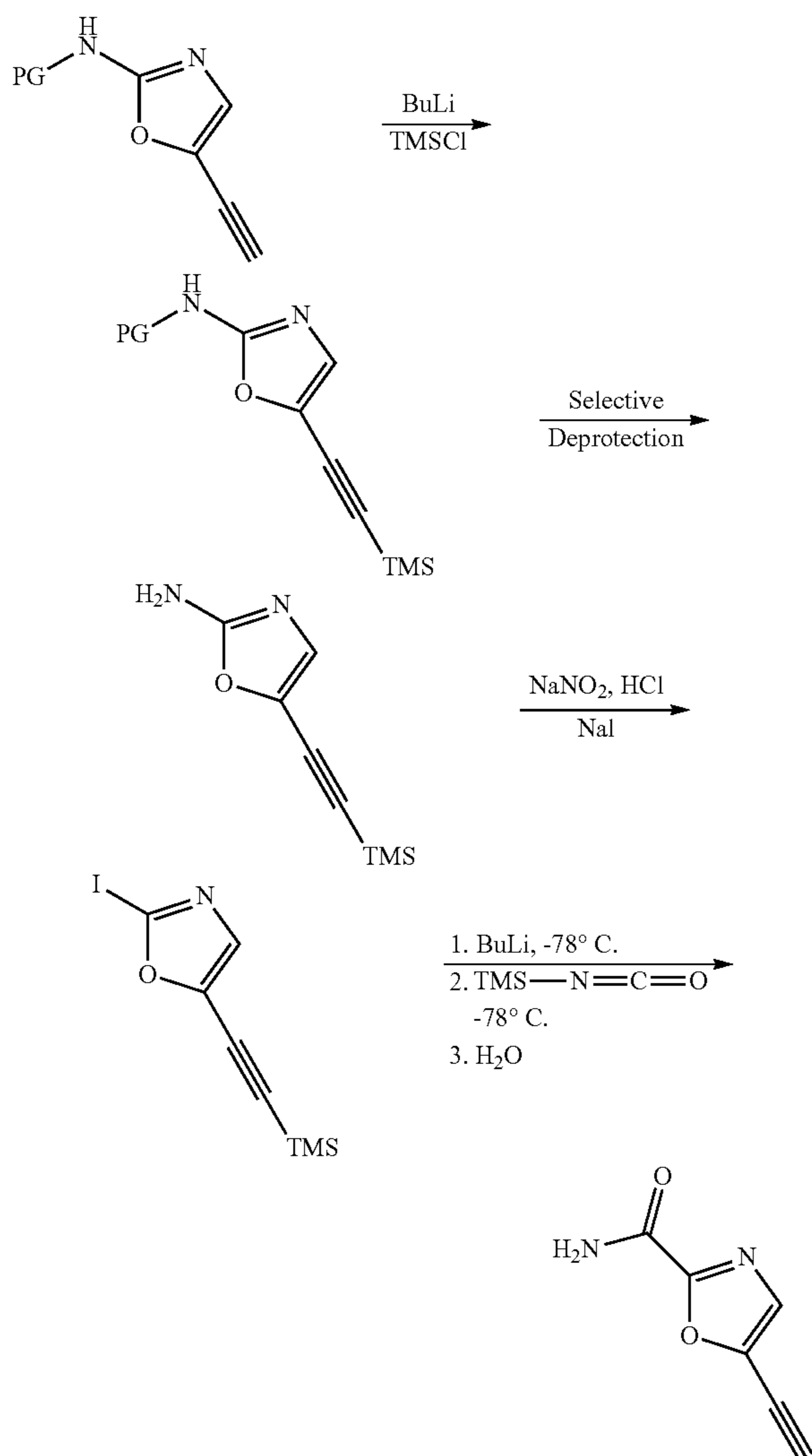
Scheme VI: Preparation of 2-aminocarbonyl substituted ethynyl oxazole
