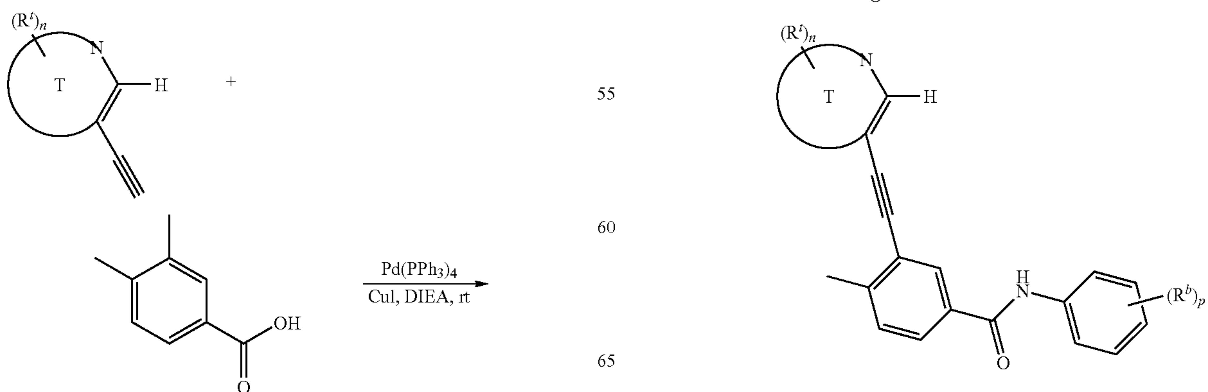
Scheme XV
