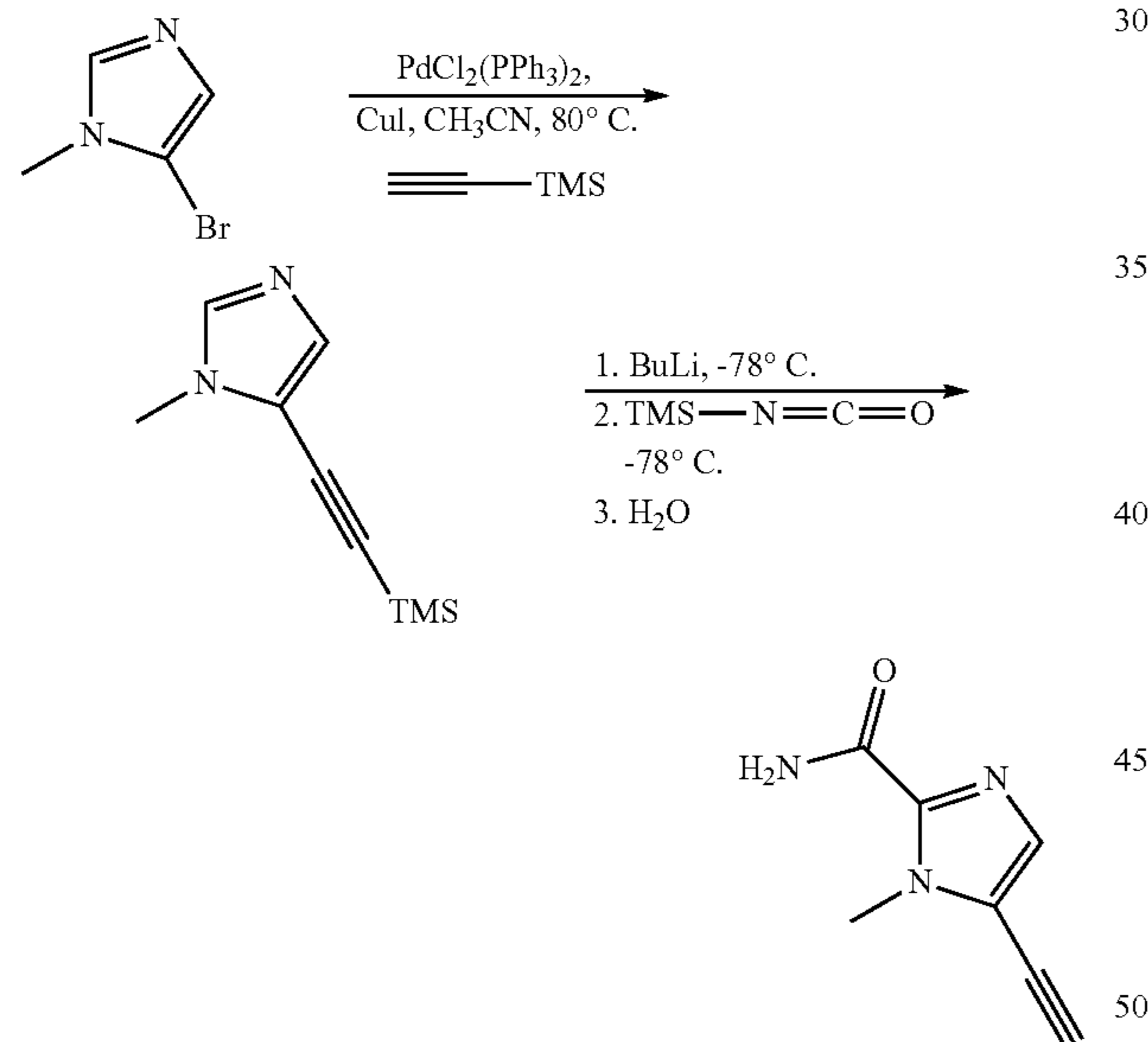
Alternative Synthesis
