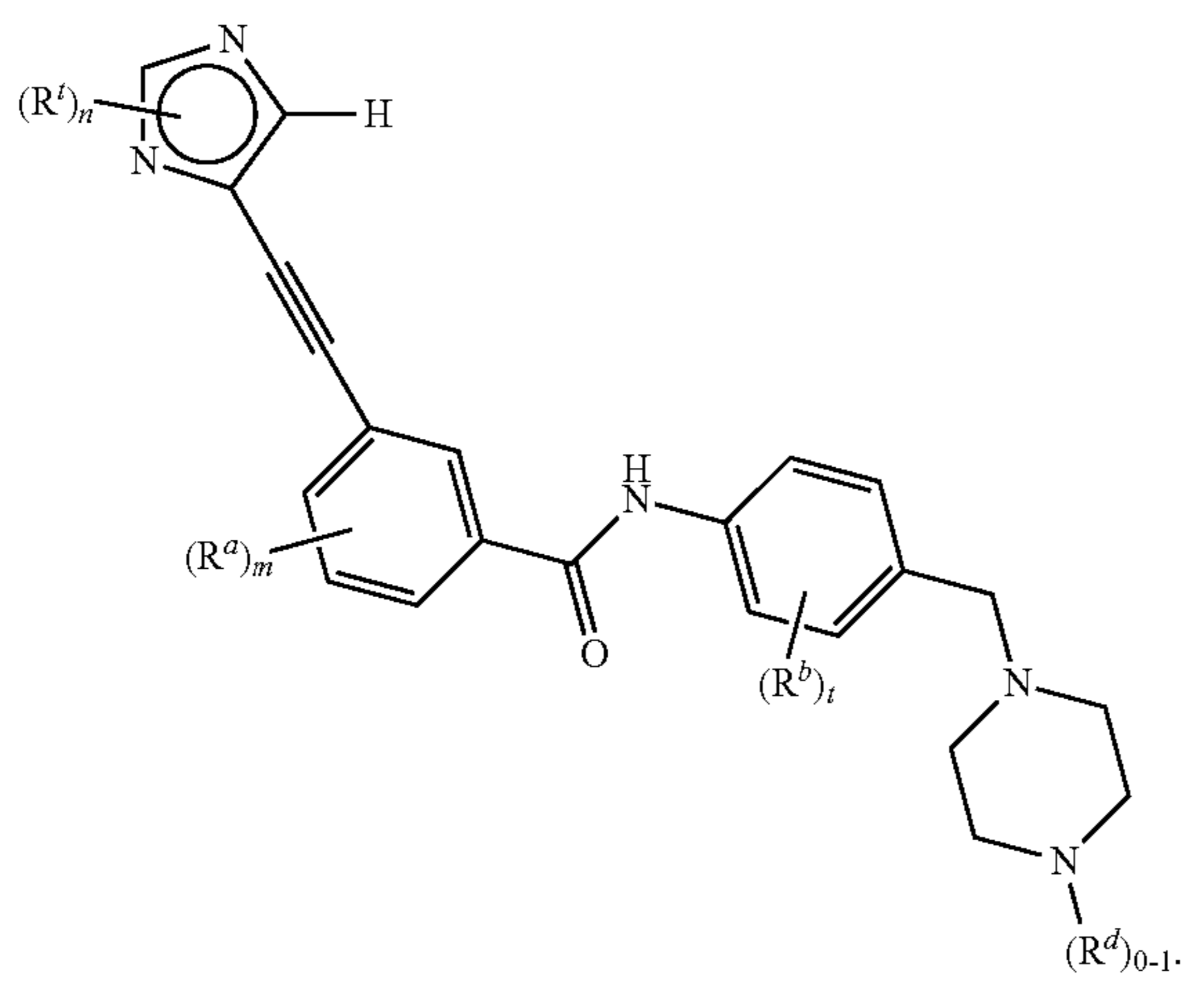
Formula IIIa
