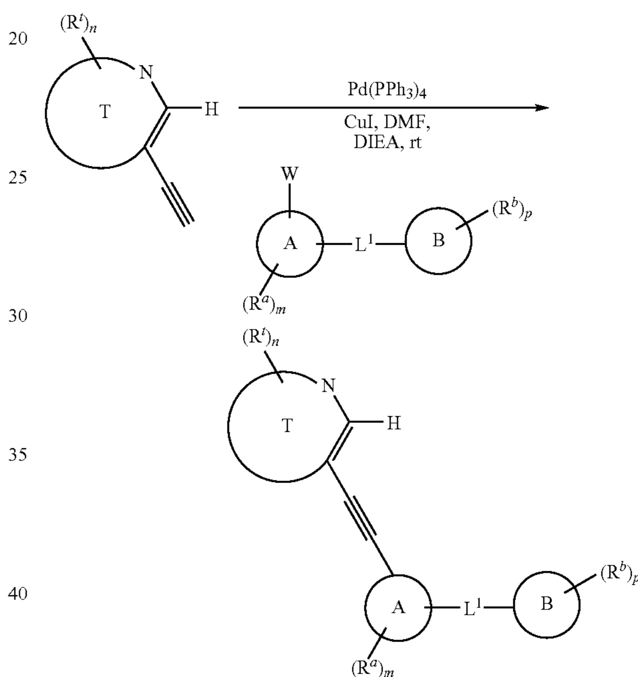
Scheme I: Sonogashira Coupling Reaction
