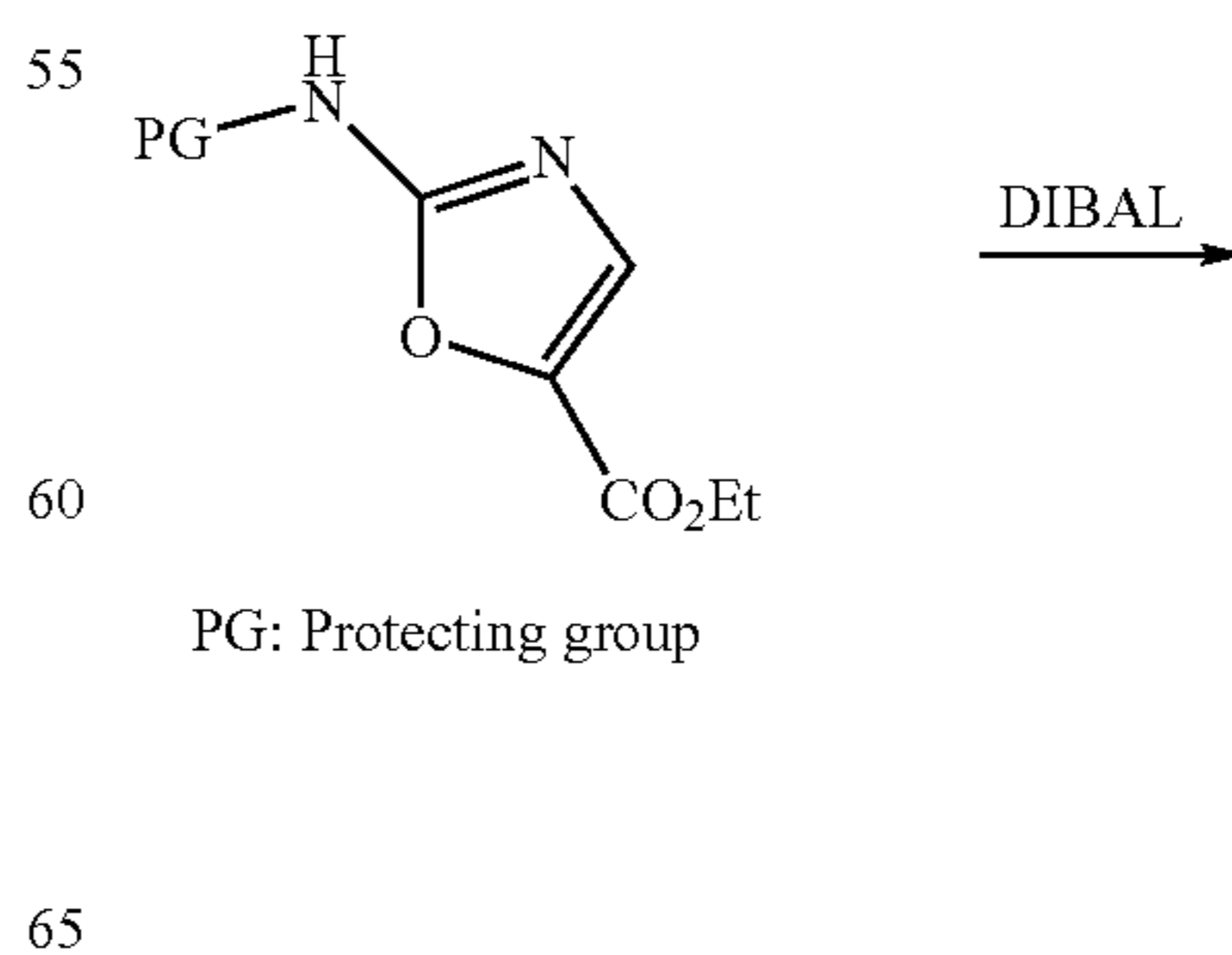
Scheme V: Preparation of 2-amino substituted ethynyl oxazole
