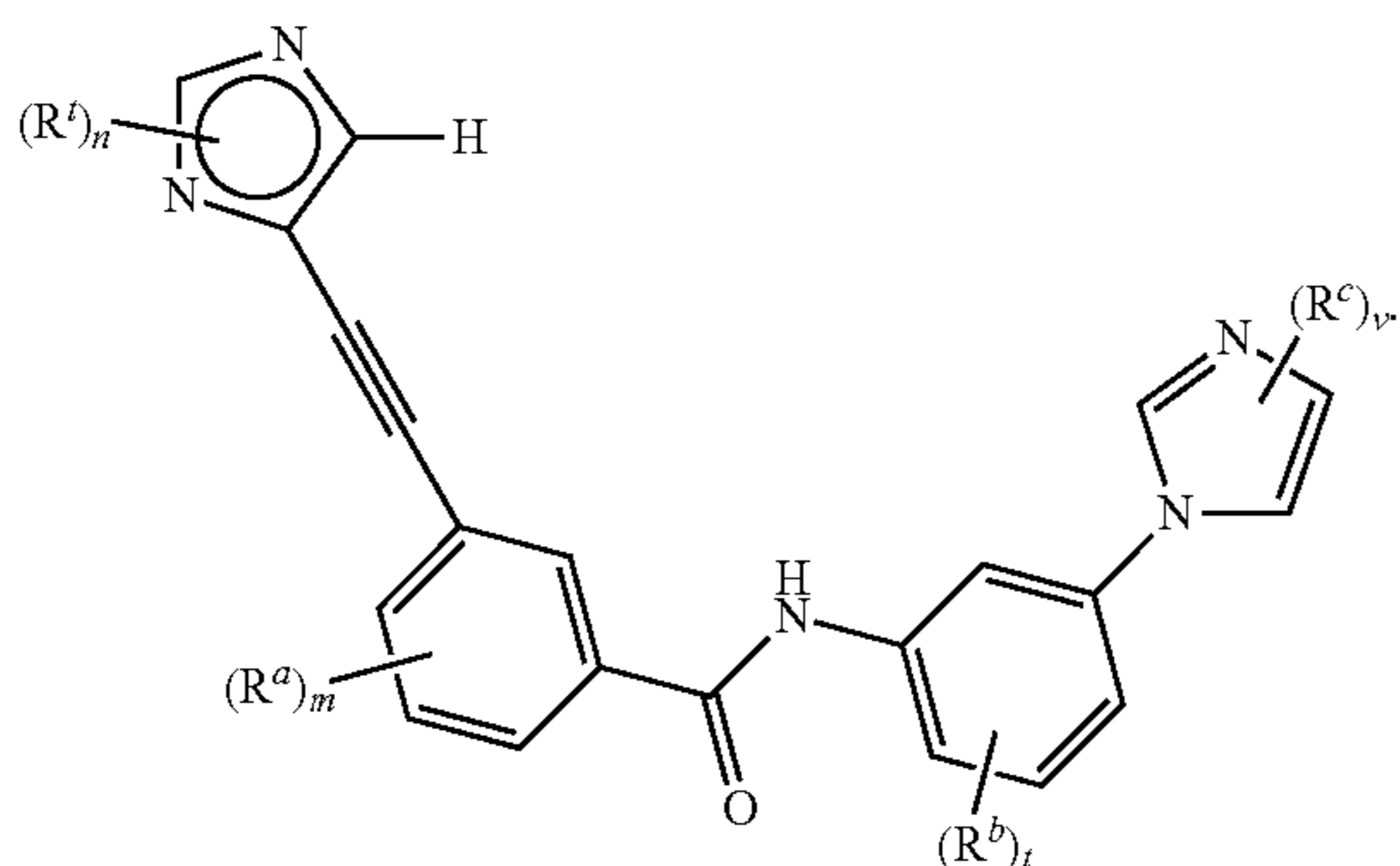
Formula IIa
