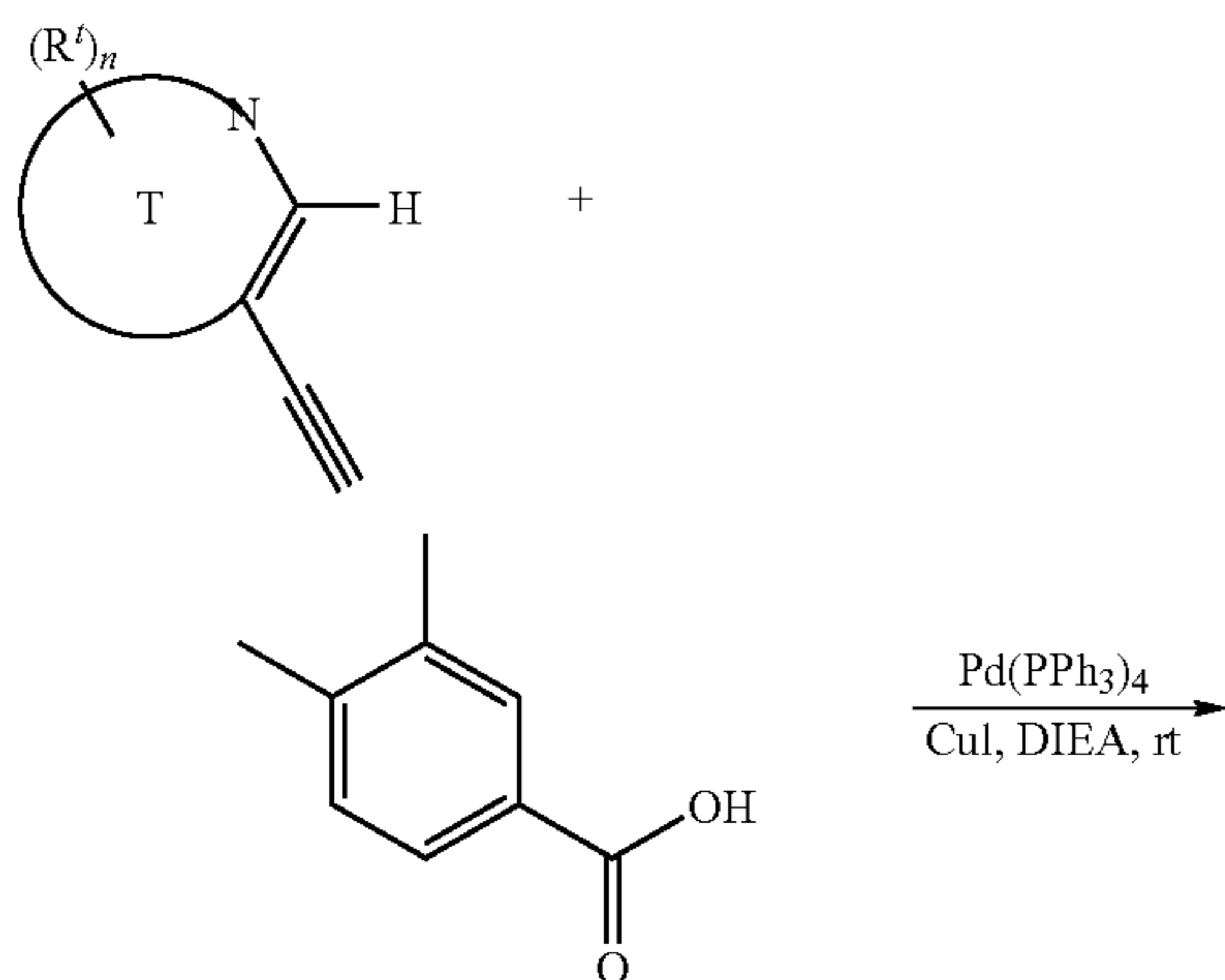
Scheme XV
