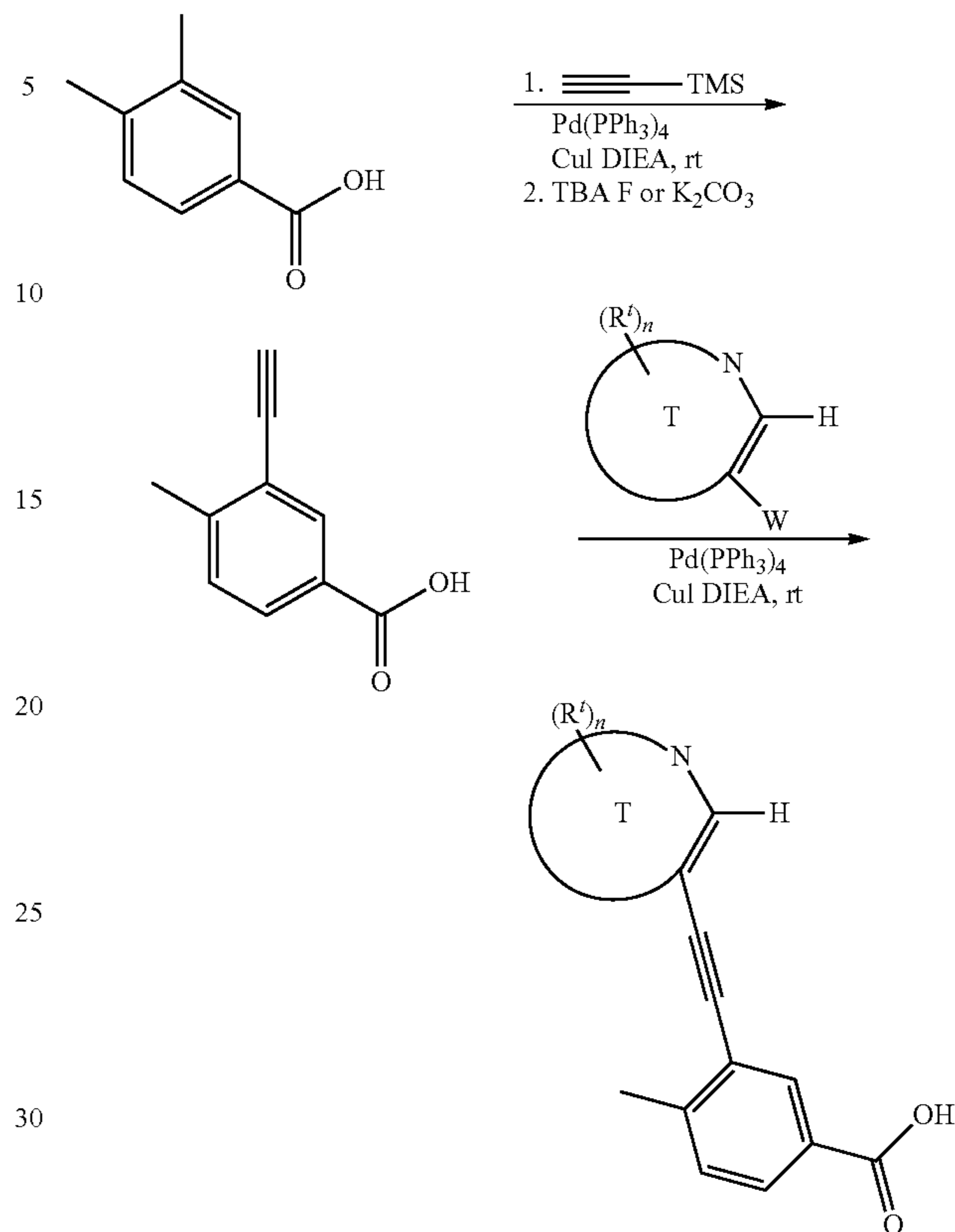
Scheme XVII
