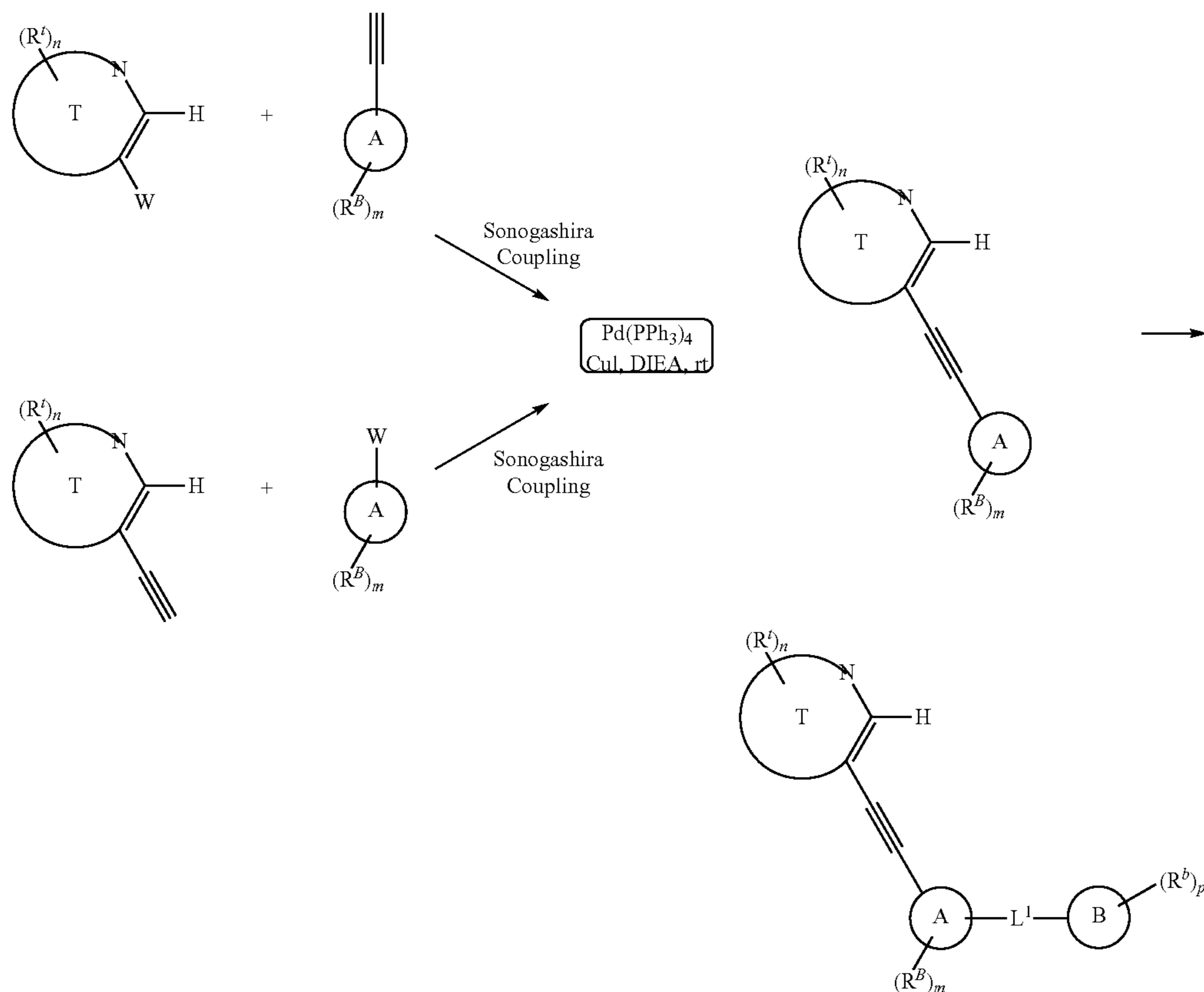
Scheme XIV
