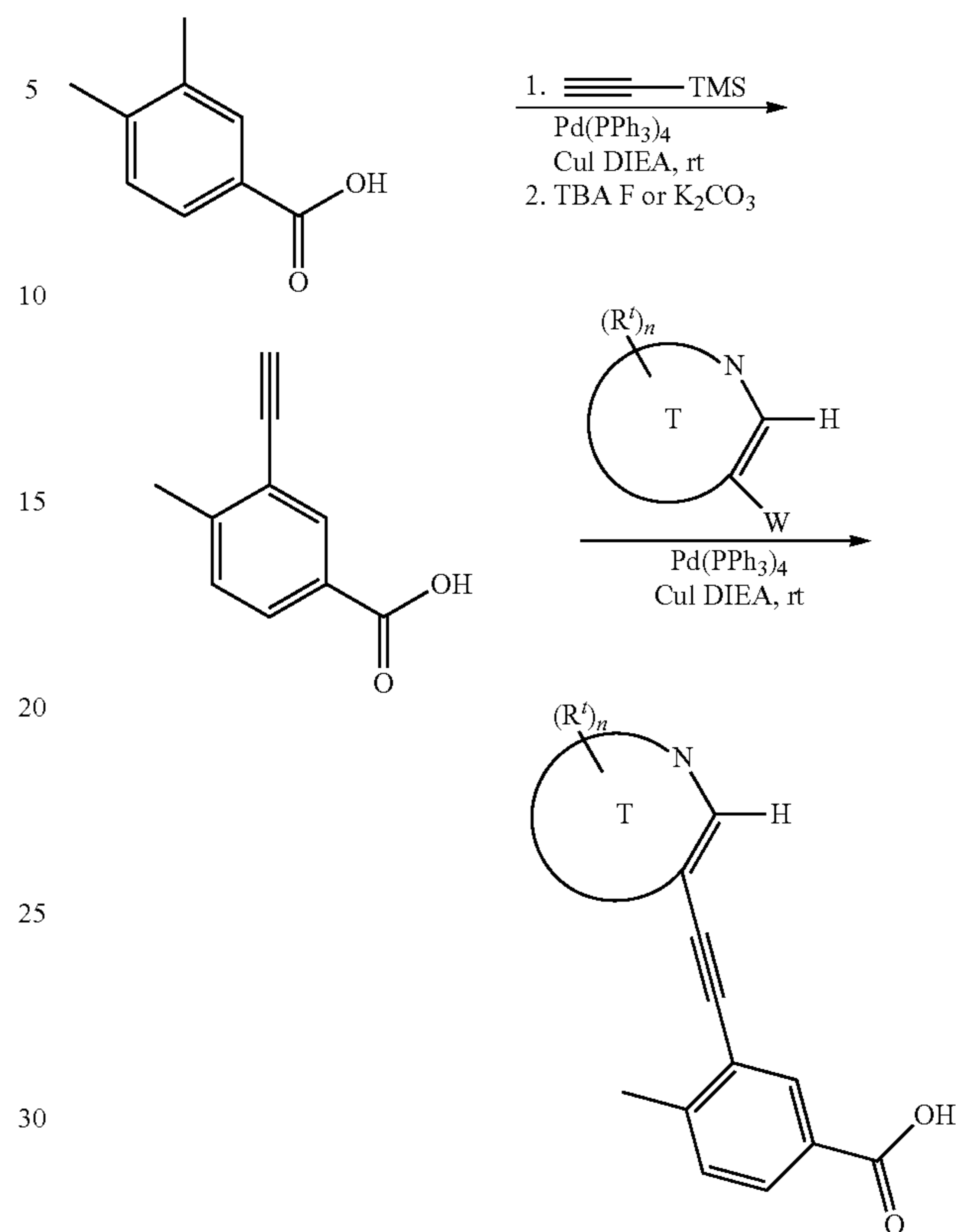
Scheme XVII
