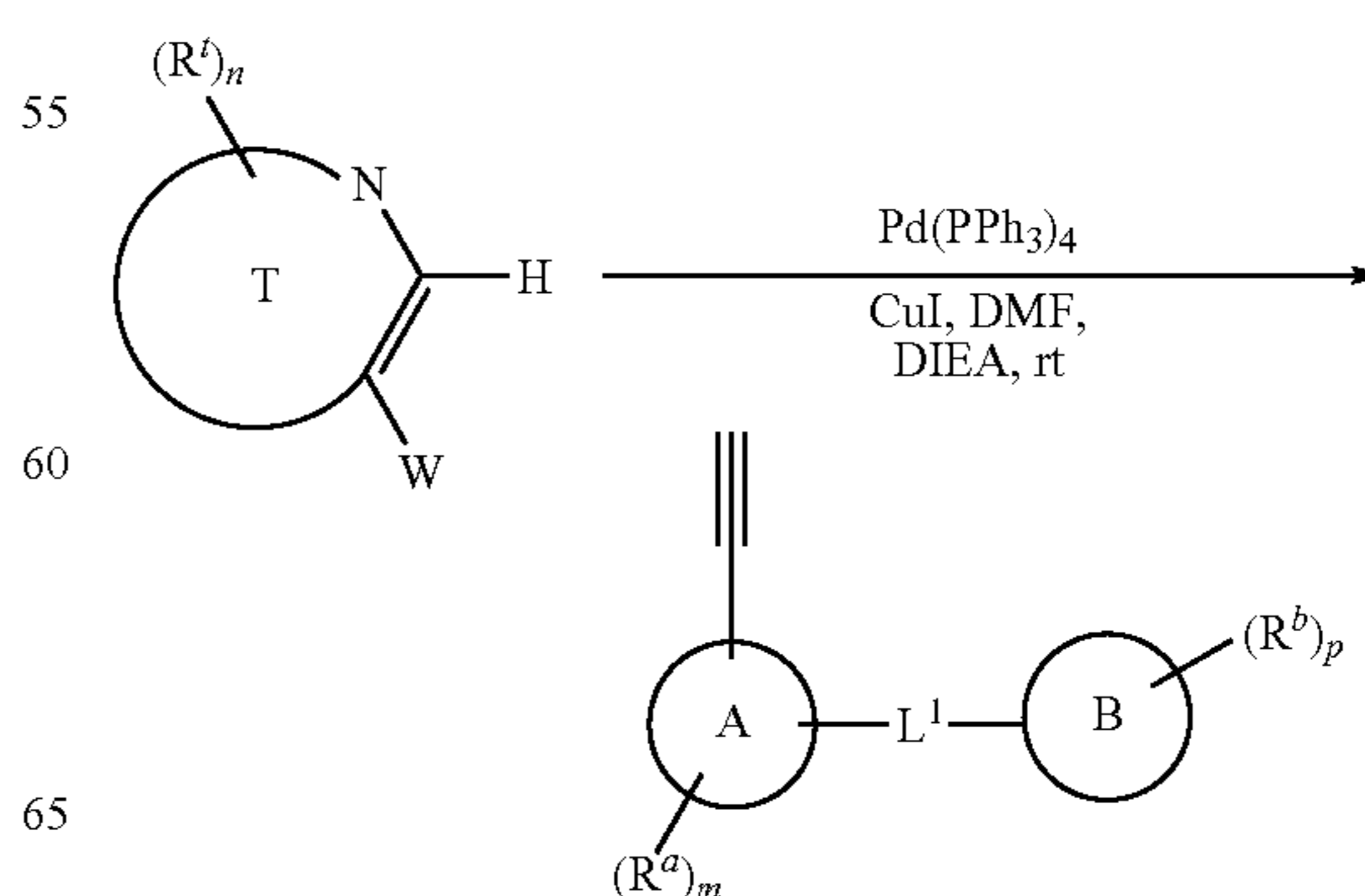
Scheme II: Alternative Sonogashira Coupling Reaction
