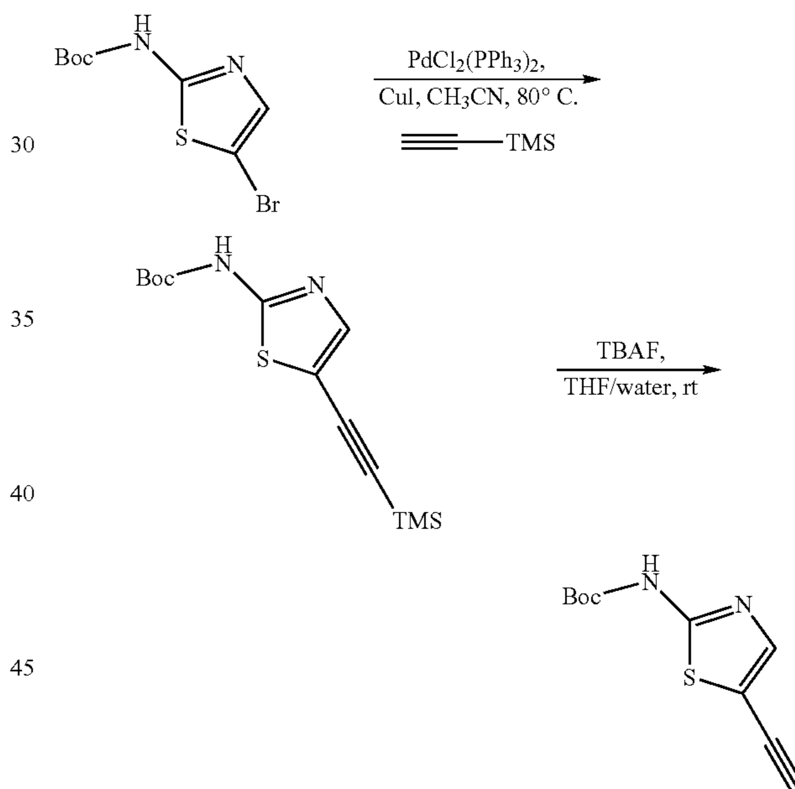
Scheme IV: Preparation of 2-substituted ethynyl thiazole
