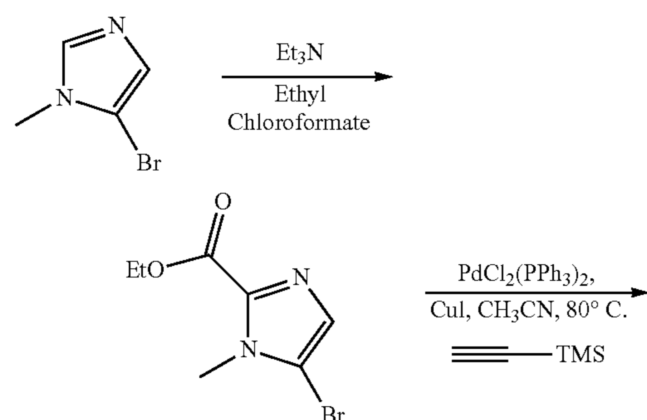
Alternative Synthesis
