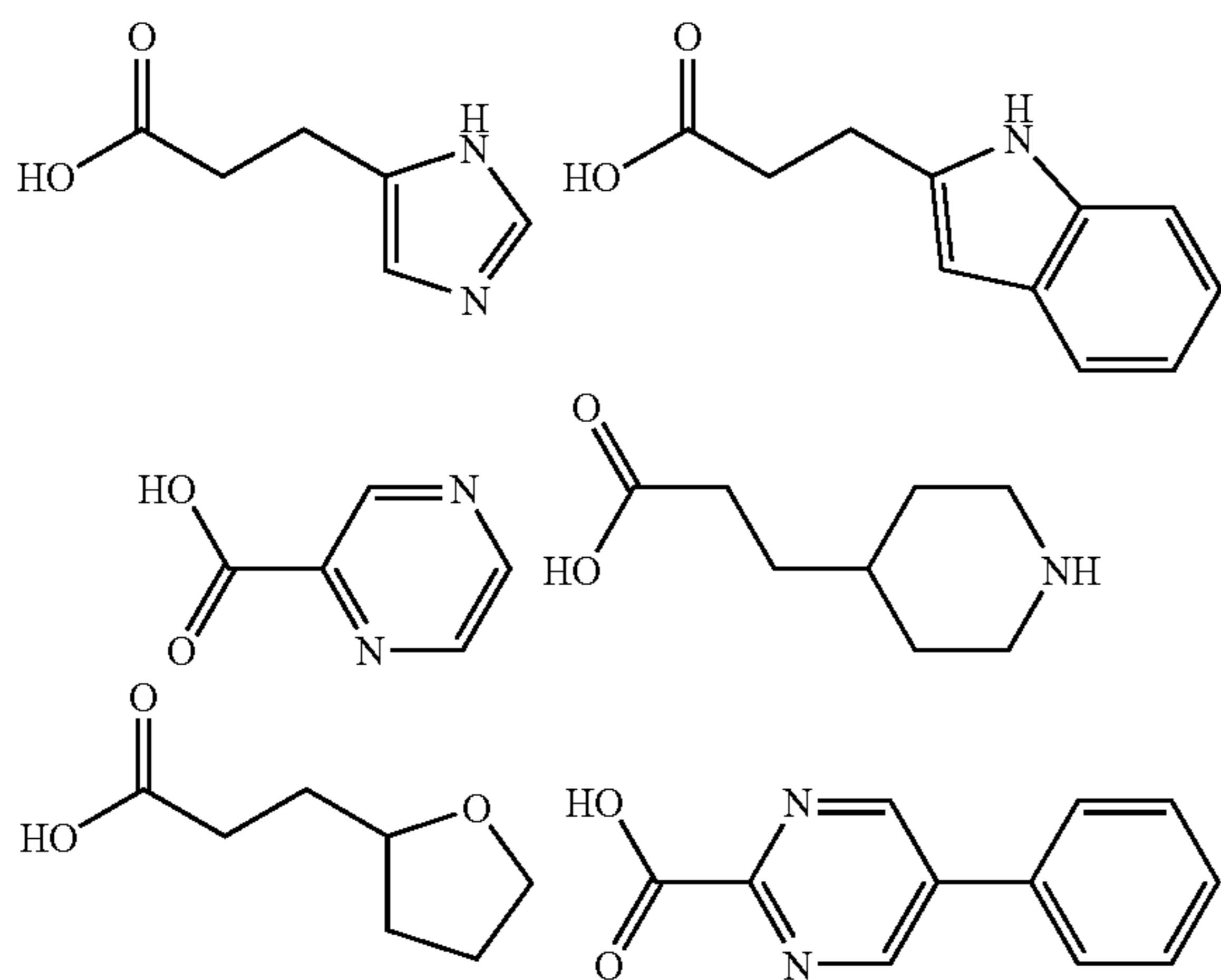
Chart 1: Representative Acids for Amination Reactions.
