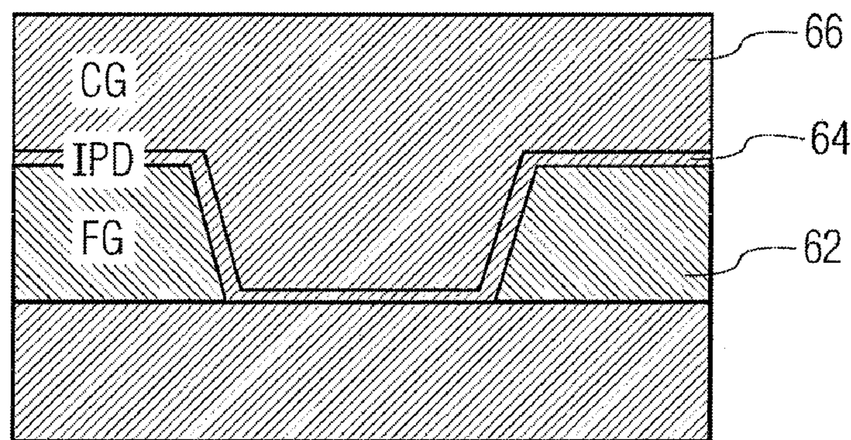
FIG. 16 PRIOR ART
