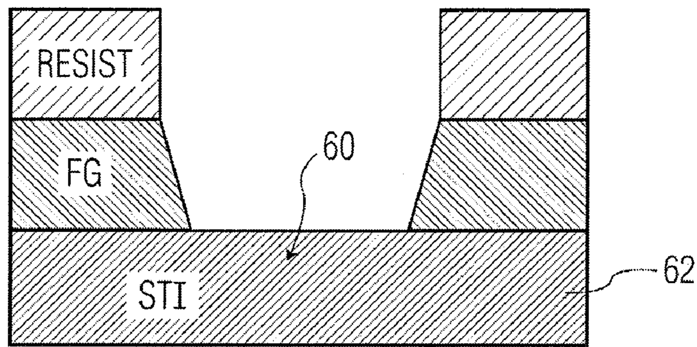
FIG. 15 PRIOR ART
