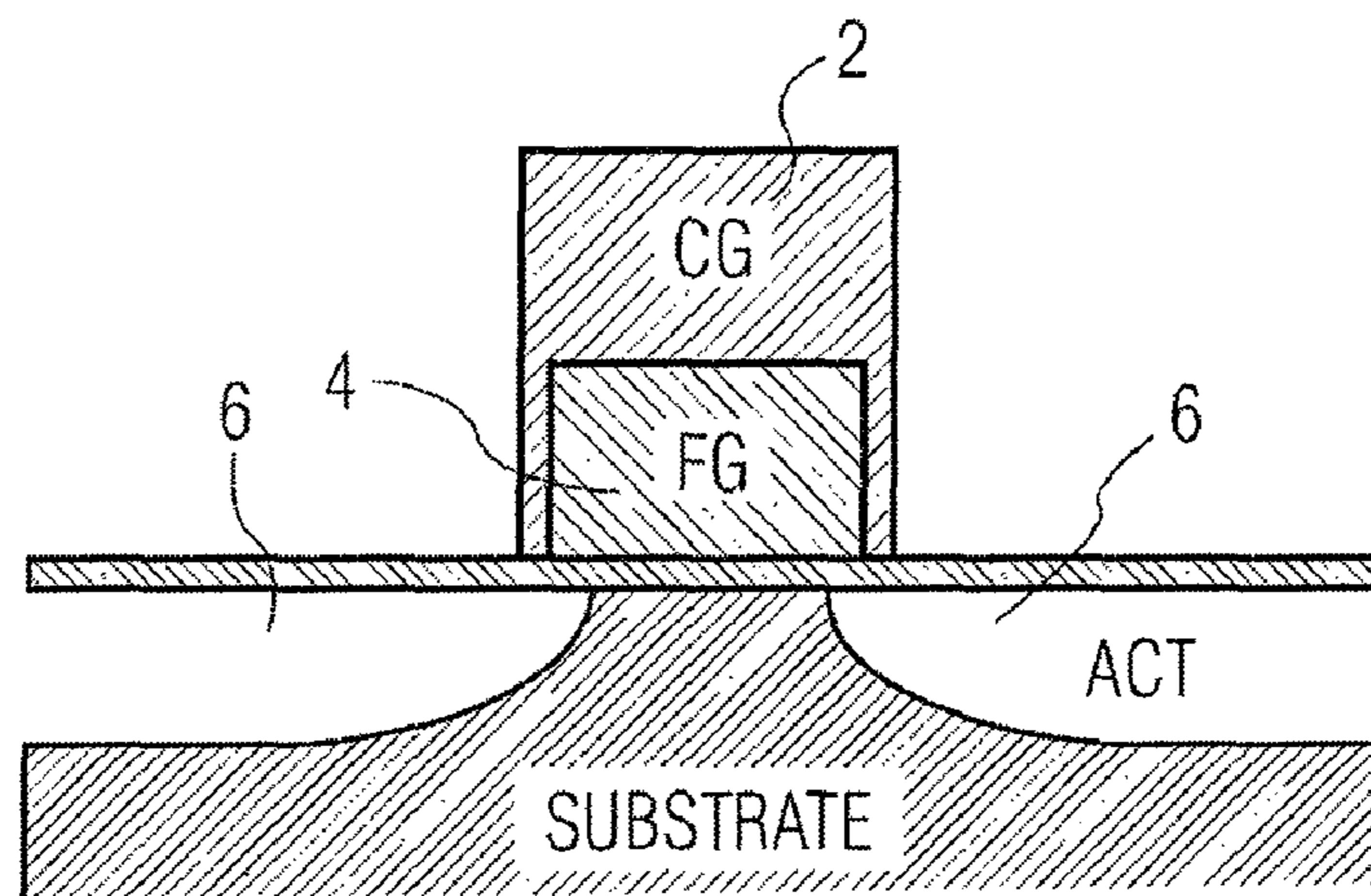
FIG. 2 PRIOR ART
