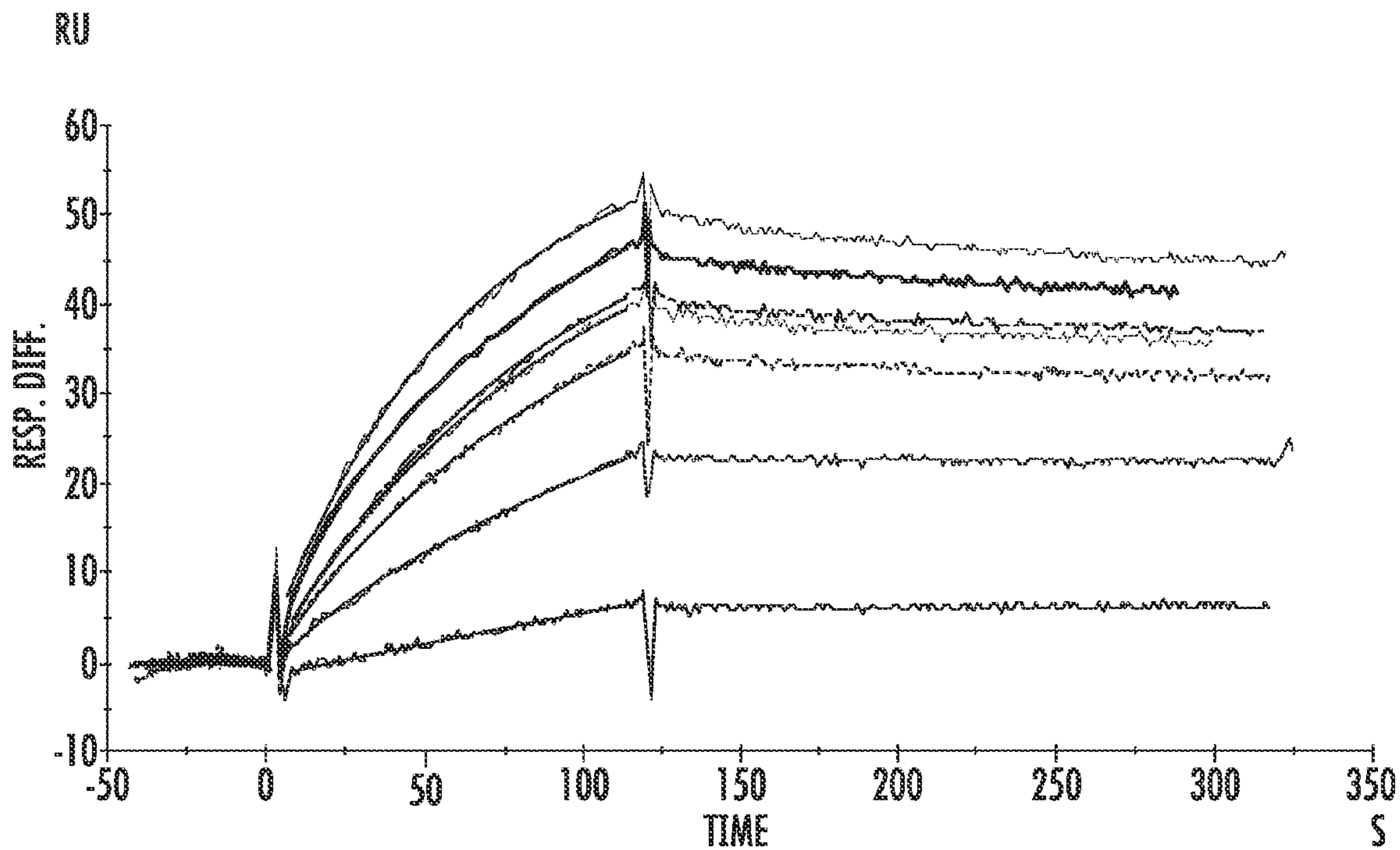
SENSORGRAM FOR RECOMBINANT hCG
