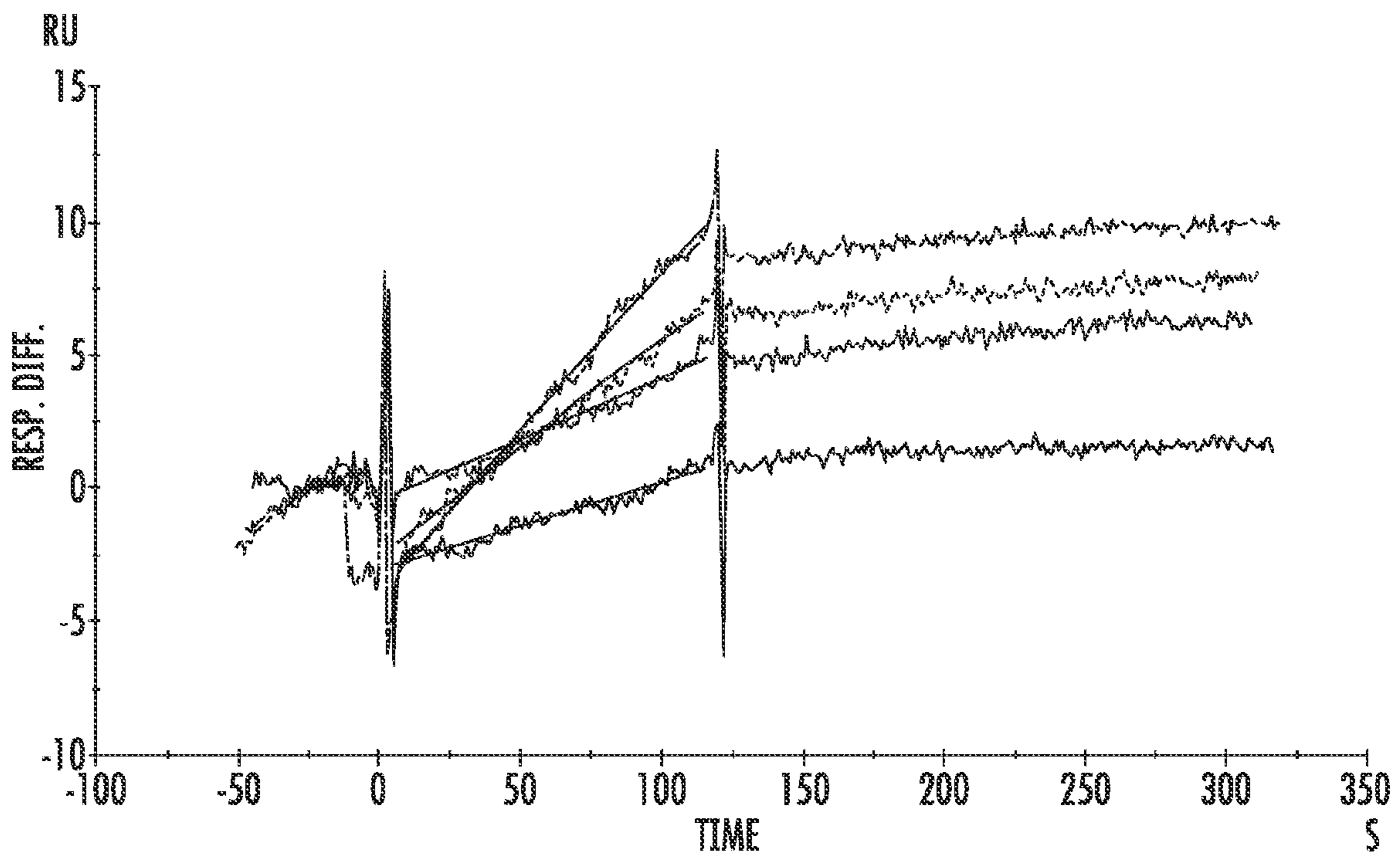
SENSORGRAM FOR B152 ON NORMALLY GLYCOSYLATED hCG
