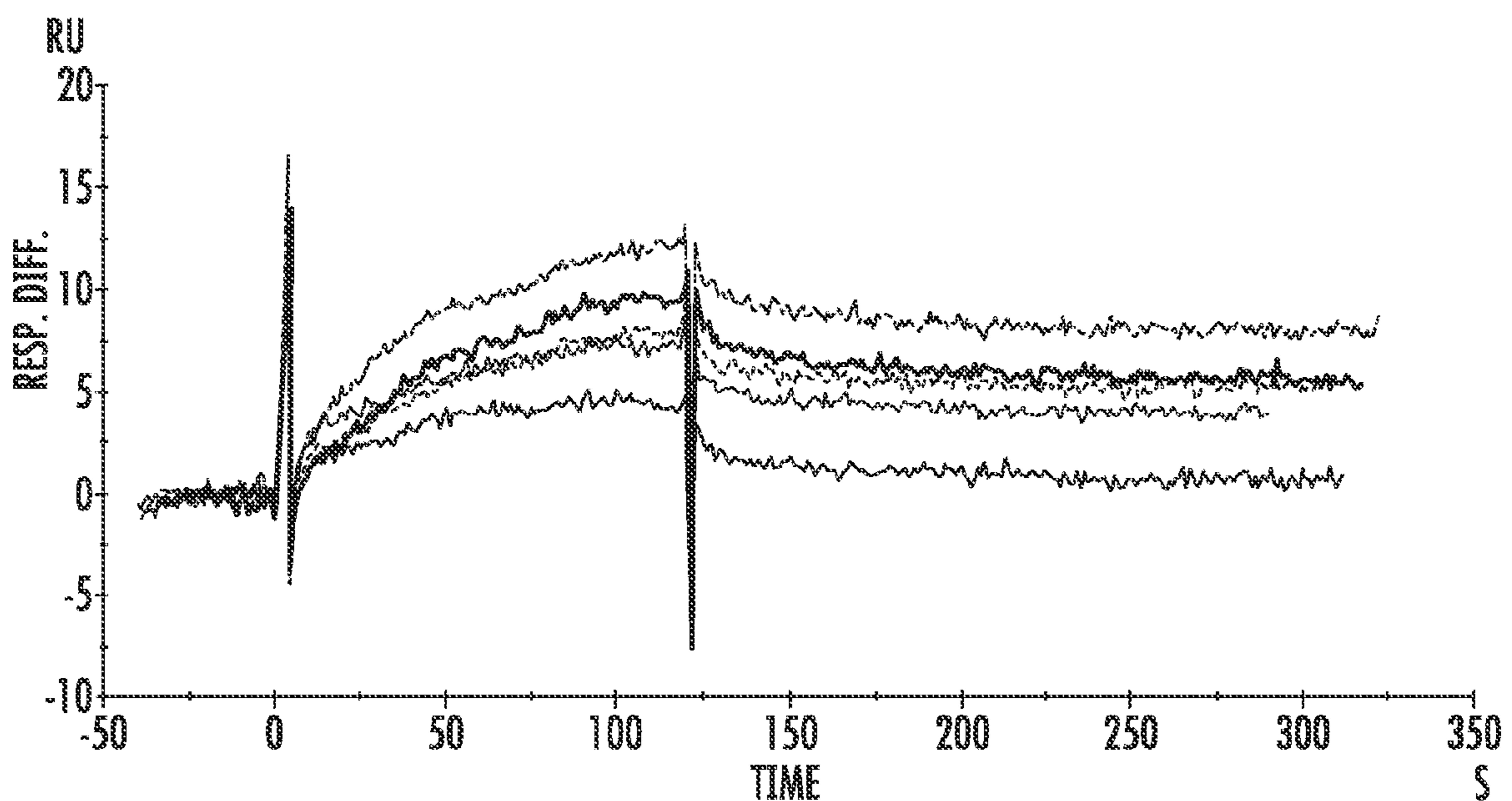
SENSORGRAM FOR B152 ON FREE \beta hCG
