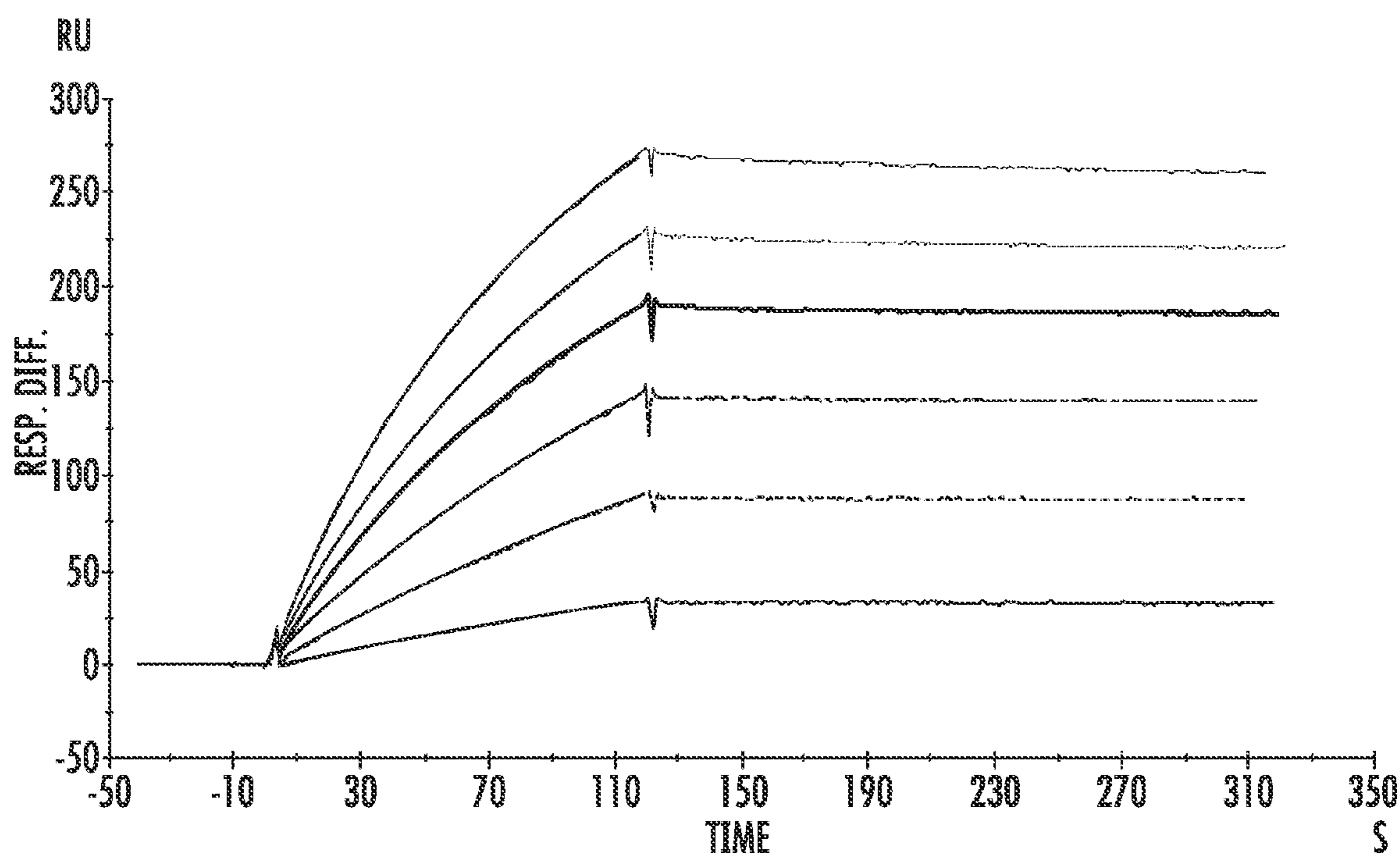
SENSORGRAM FOR JEG-3 hCG-H
