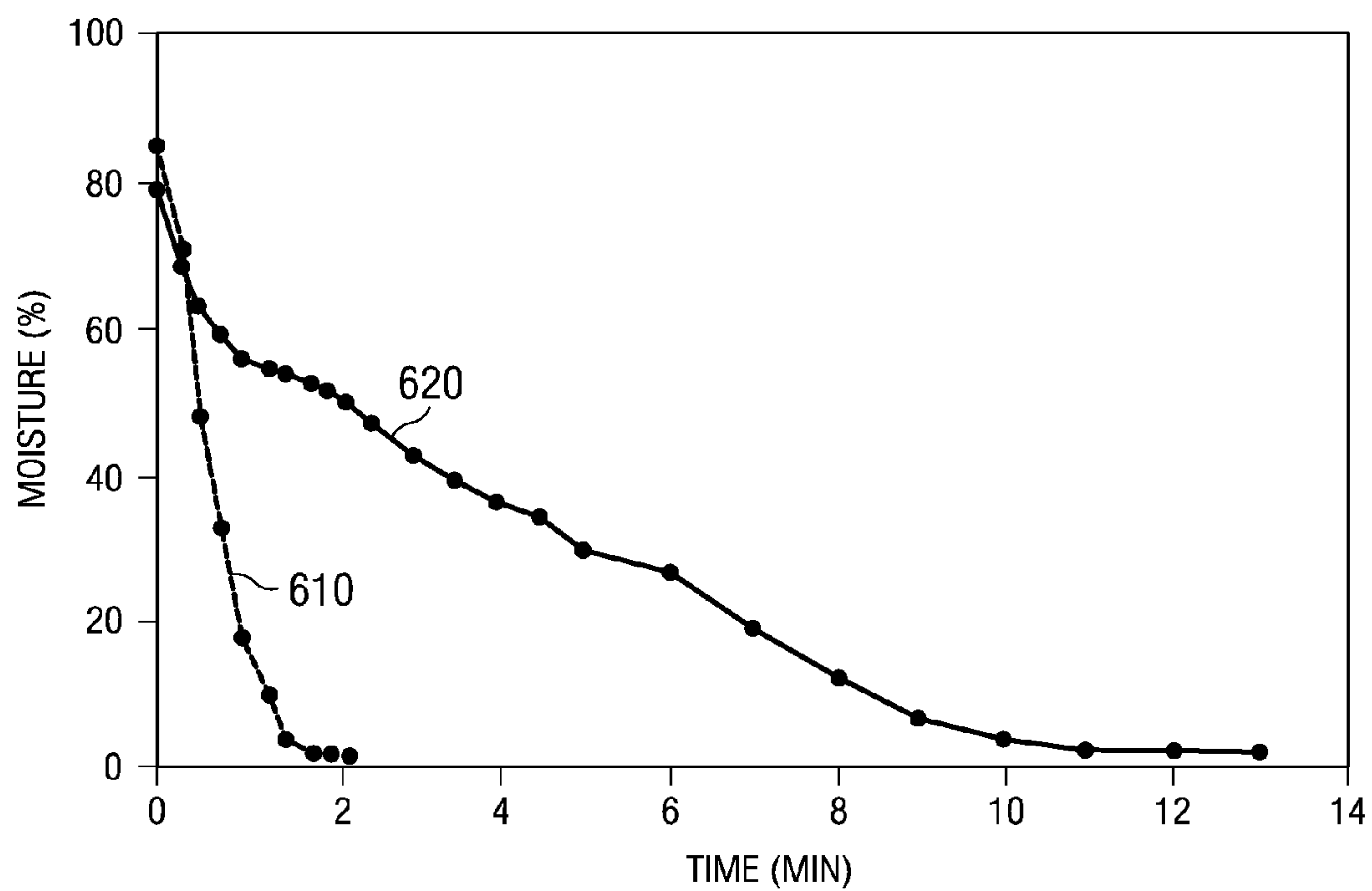
FIG. 6 (PRIOR ART)
