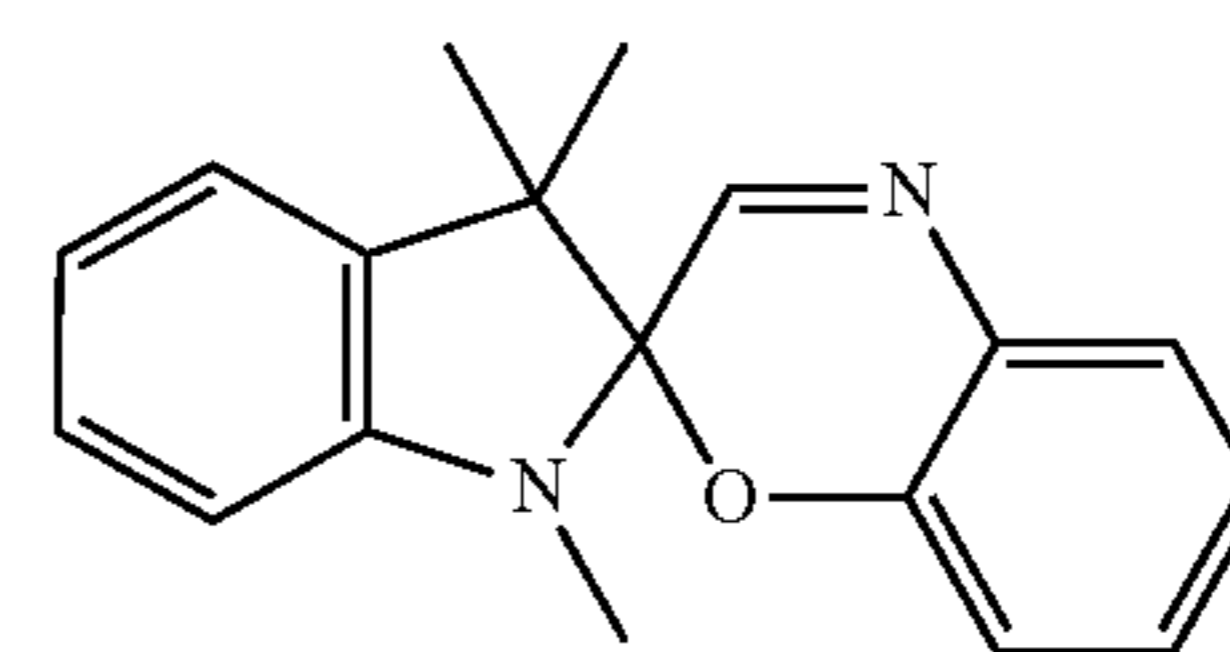
spirooxazine (16)
