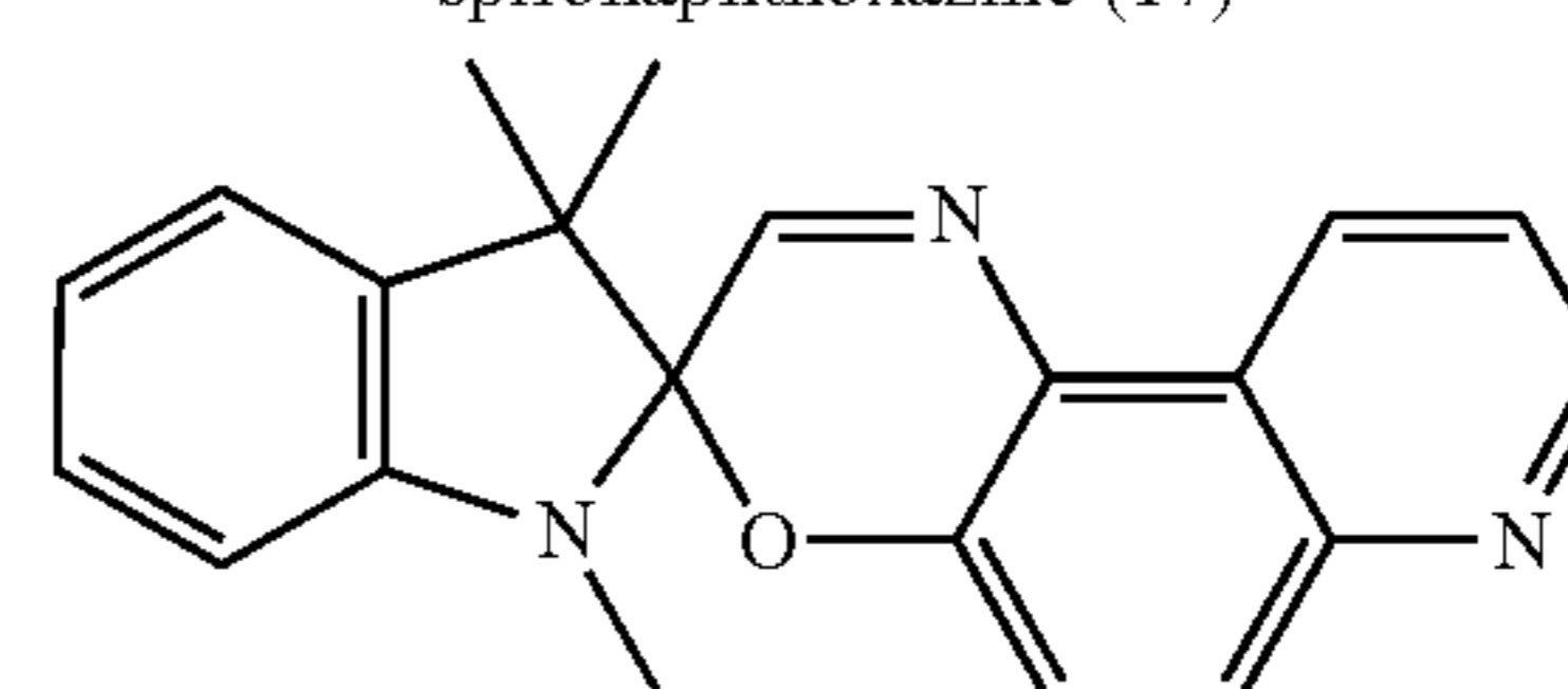
spiroindolinopyridobenzoxazine (18)
