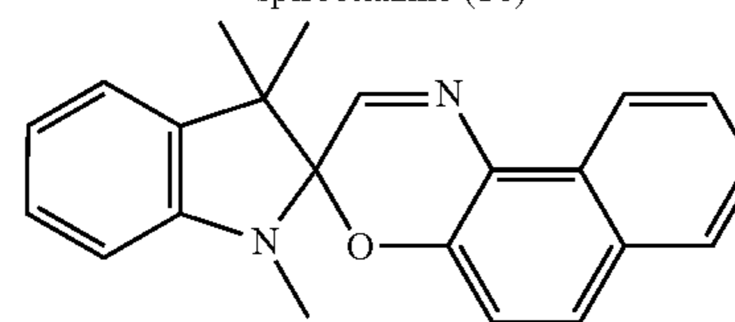
spironaphthoxazine (17)
