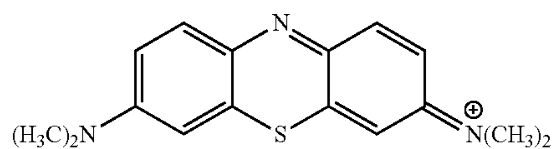
CI Basic Blue 9
