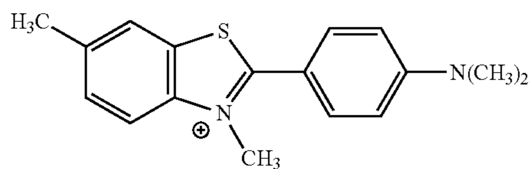
CI Basic Yellow 1
