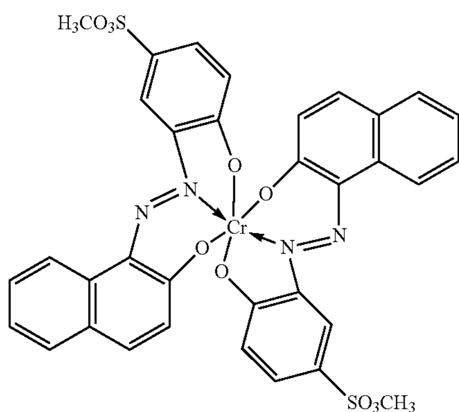
C.I. Acid Violet 78
