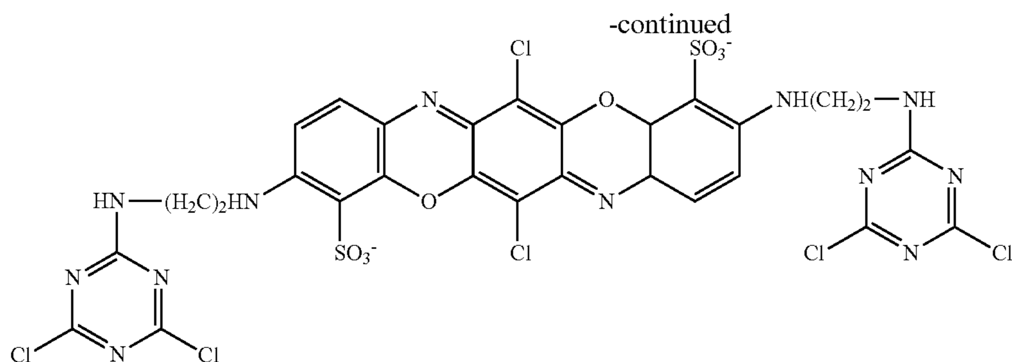
CI Reactive Blue 163
