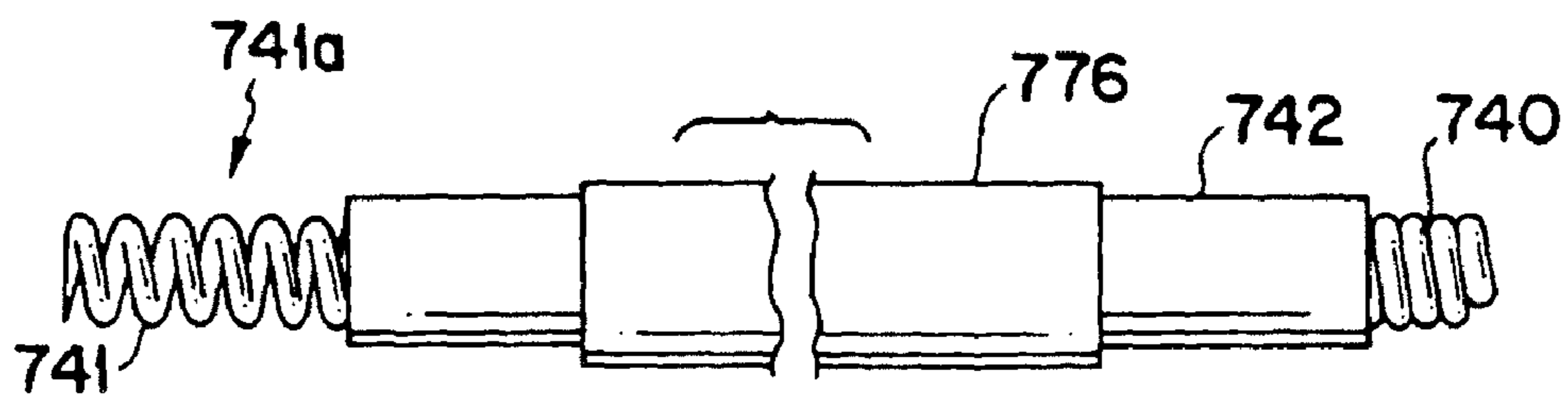
FIG. 3D
