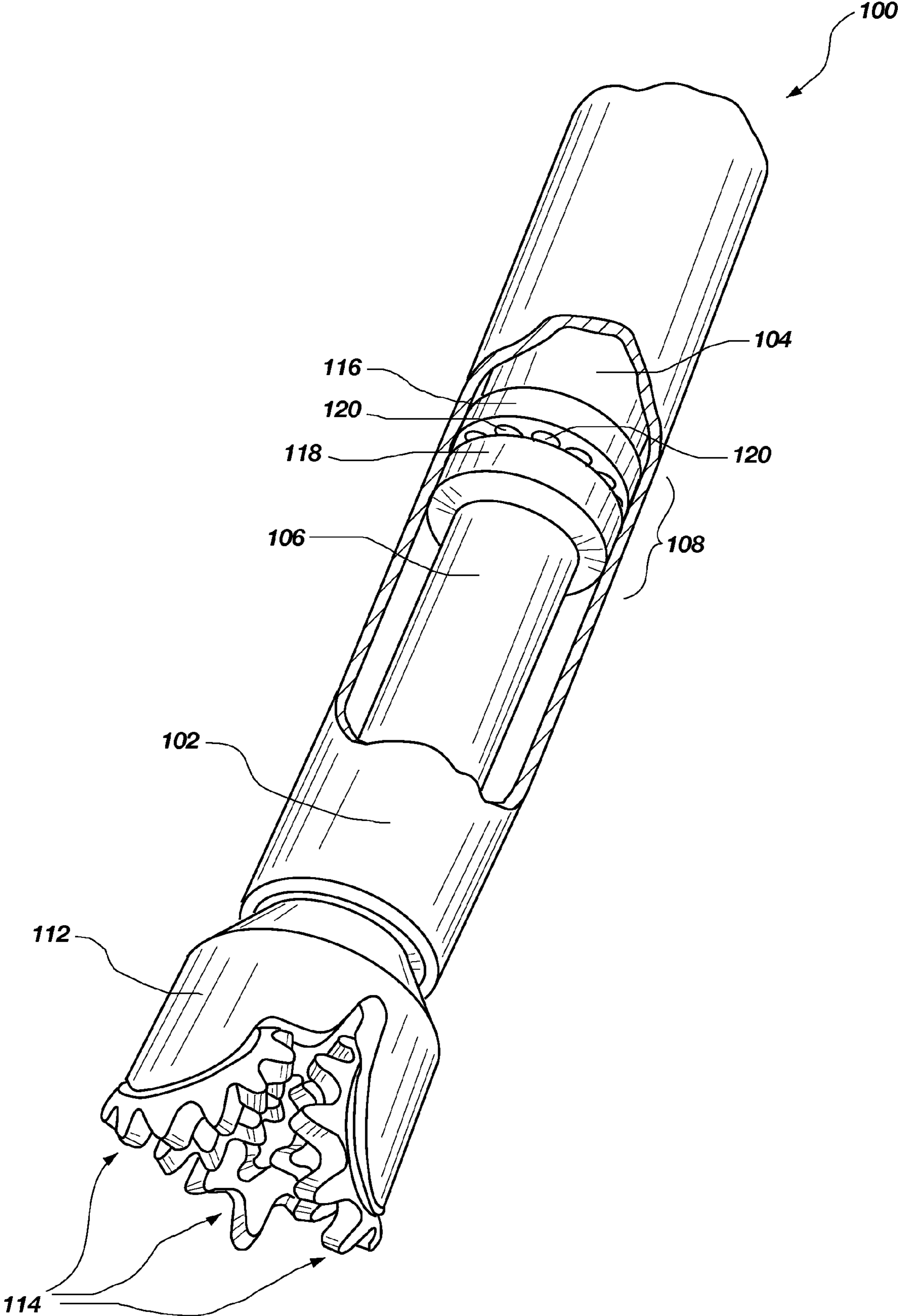
FIG. 1 (PRIOR ART)
