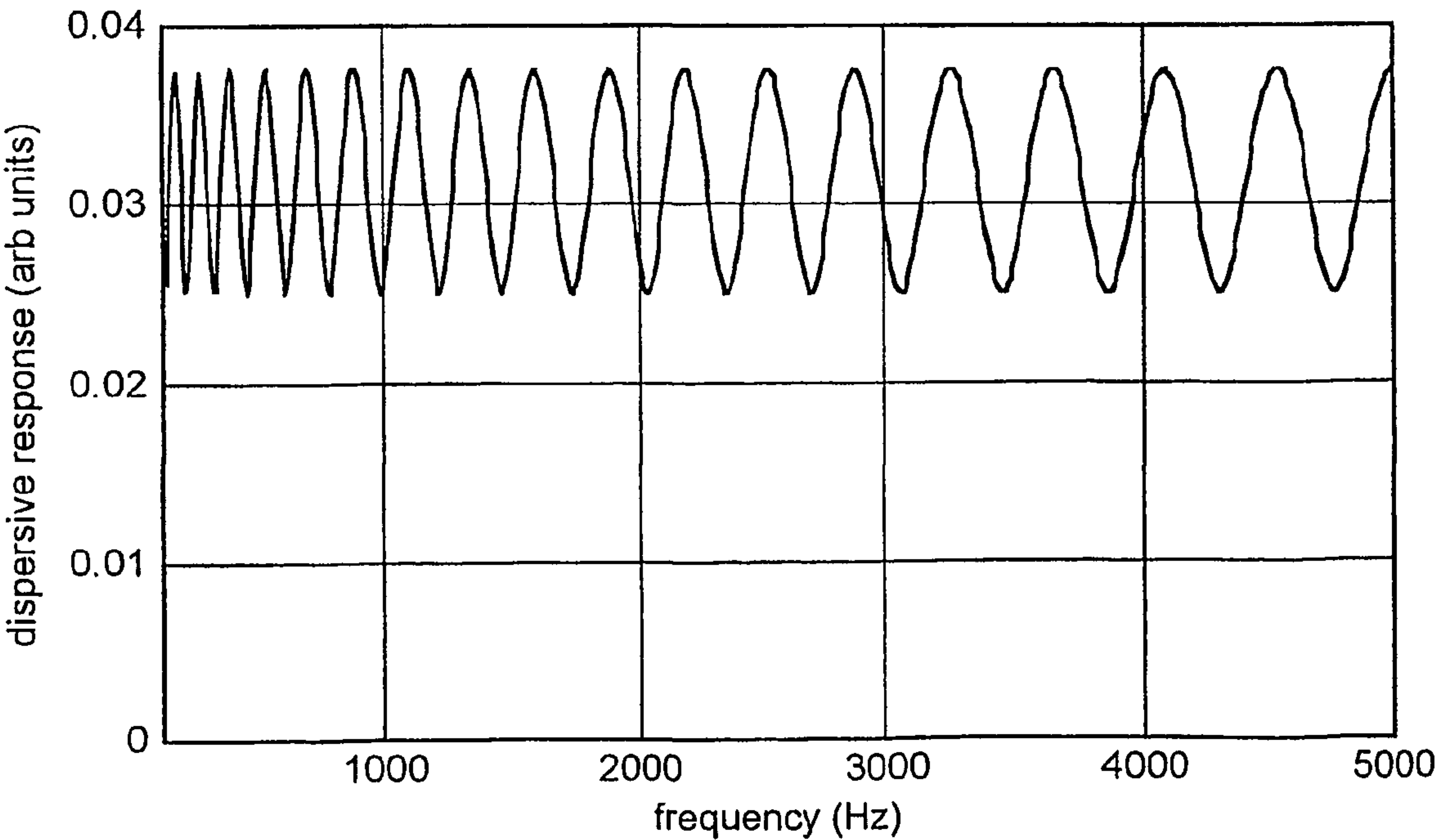
Graph of a dispersive frequency response
