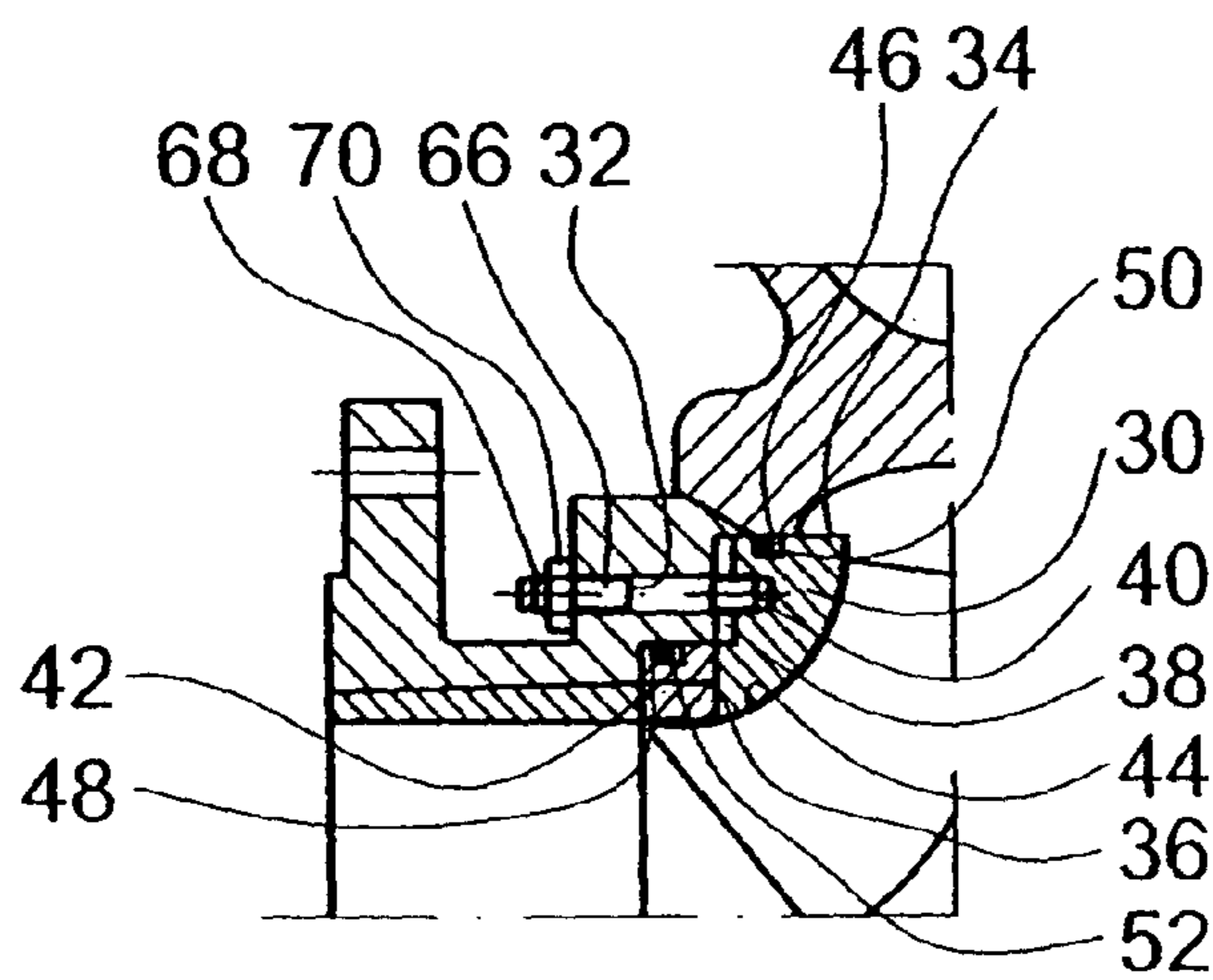
Fig. 2 (PRIOR ART)
