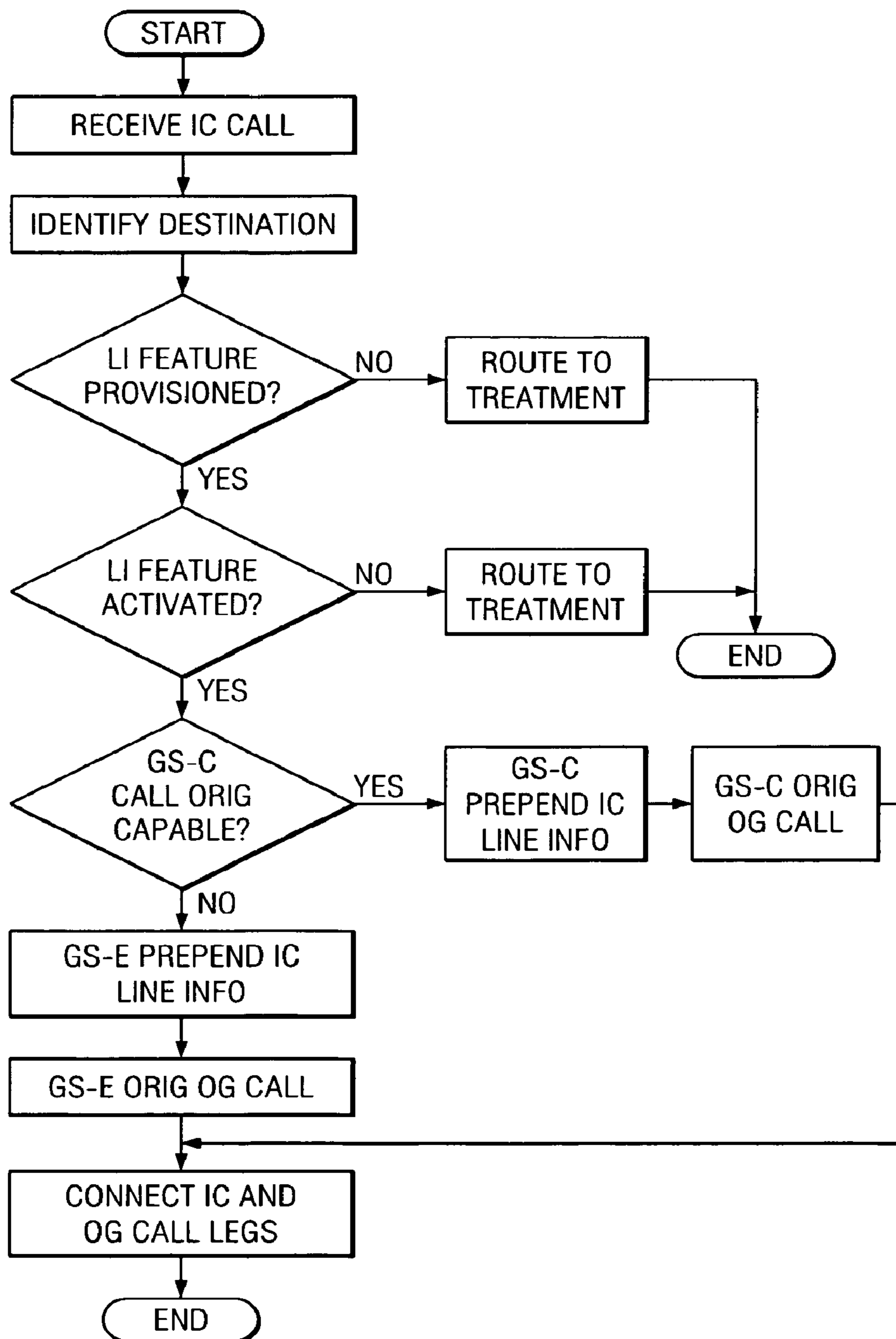
INCOMING CALL HANDLING FLOW CHART
