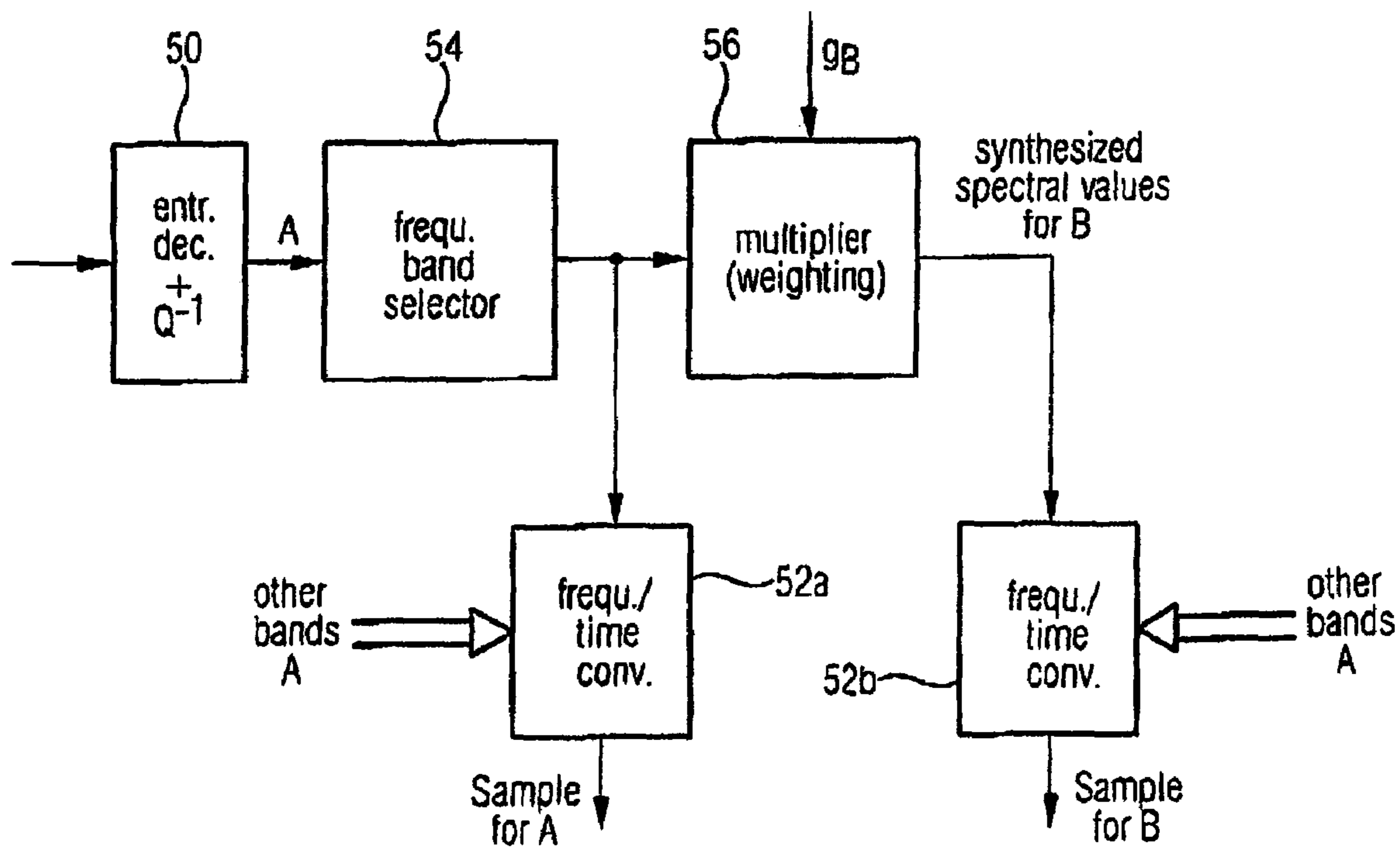
FIG 5 (decoder side)
