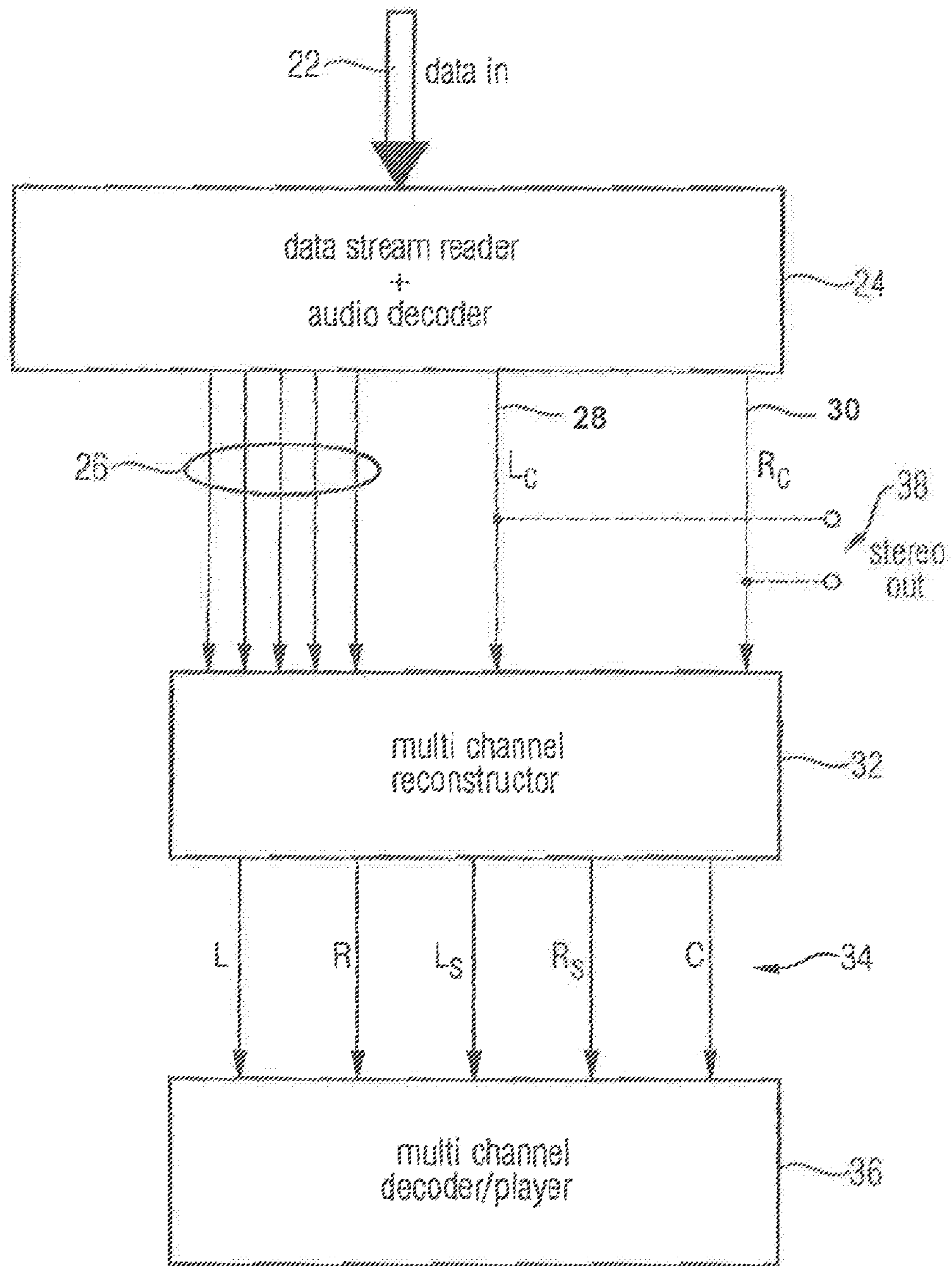
FIG 2 (Decoder)
