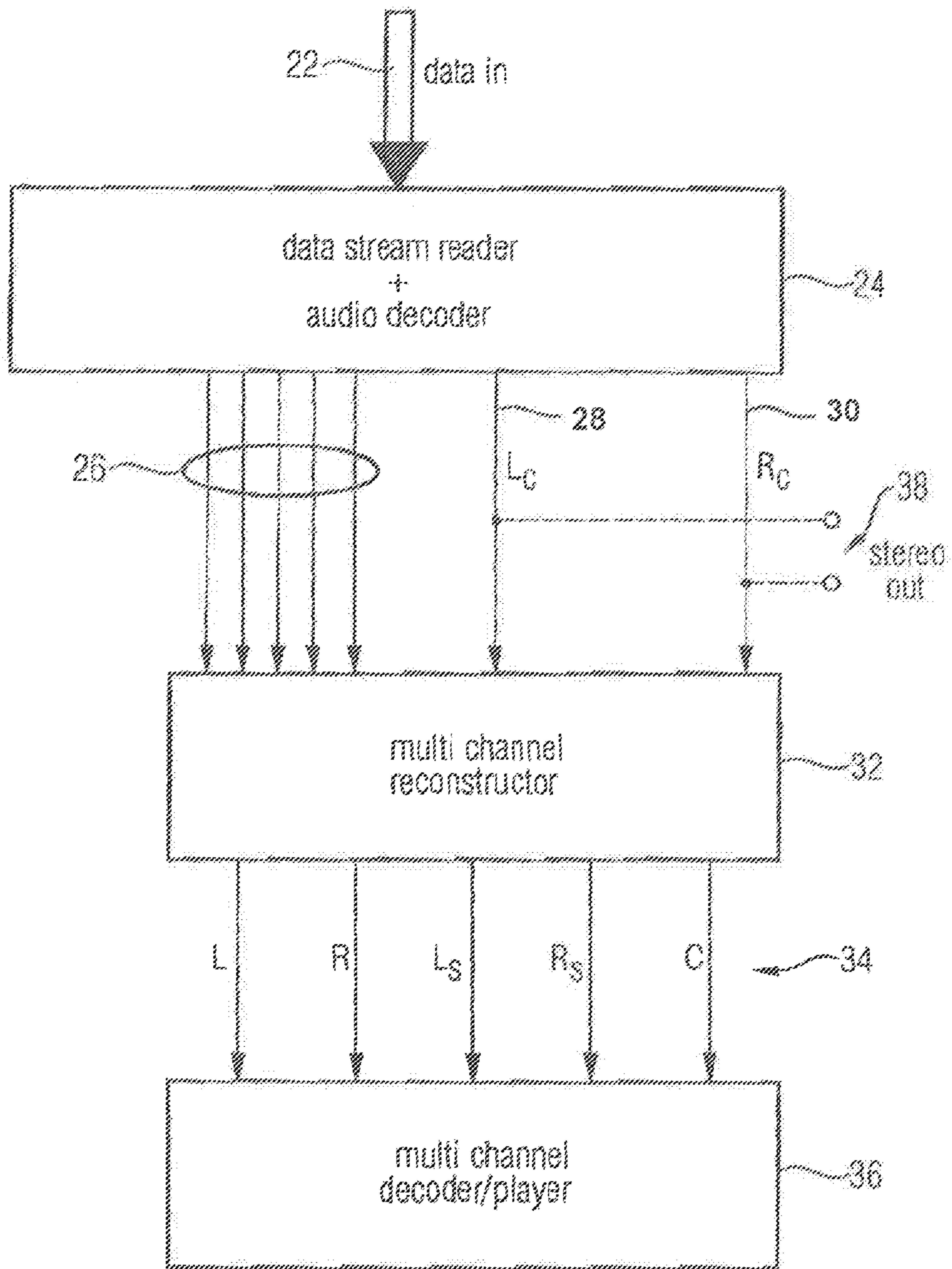
FIG 2 (Decoder)
