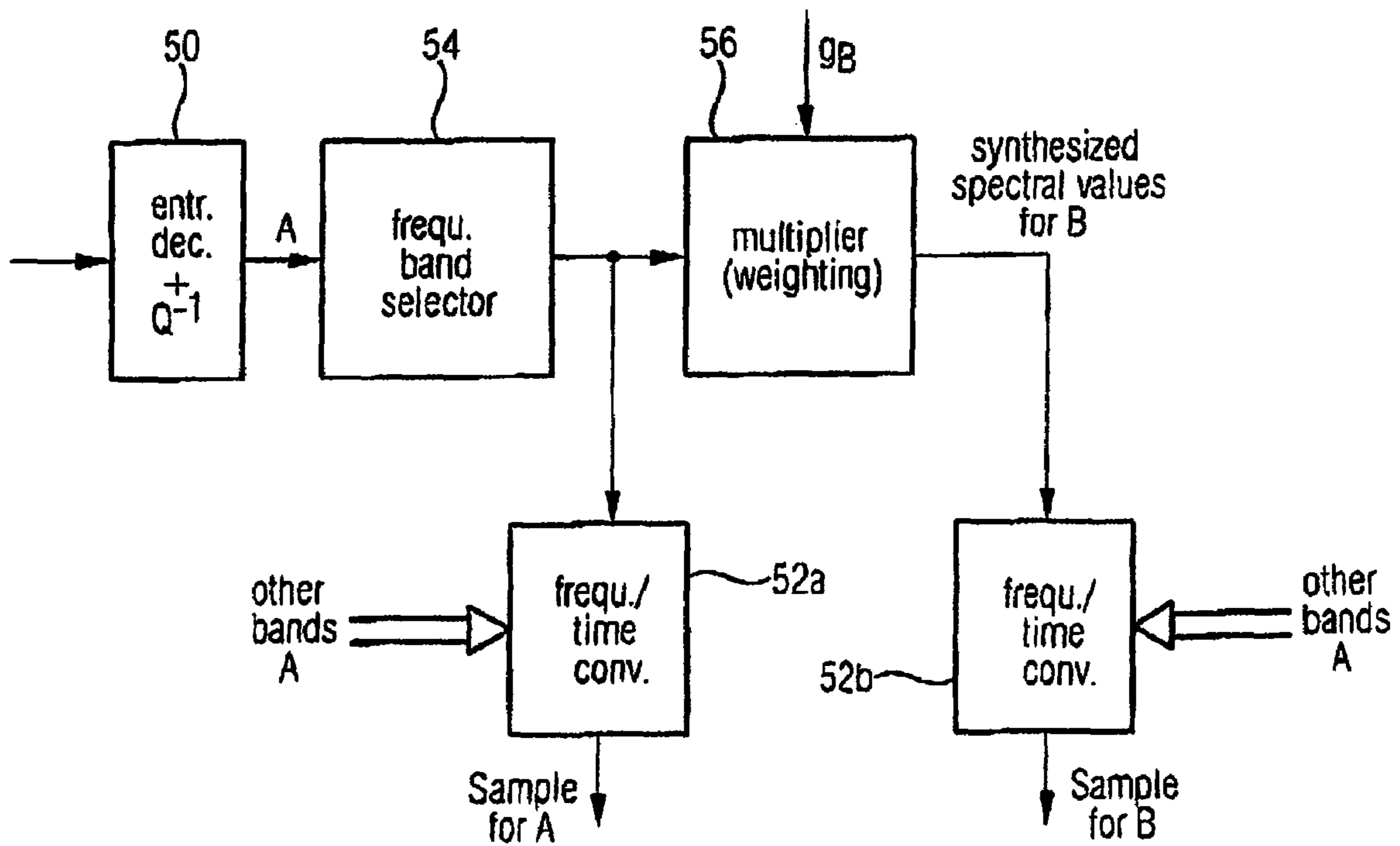
FIG 5 (decoder side)
