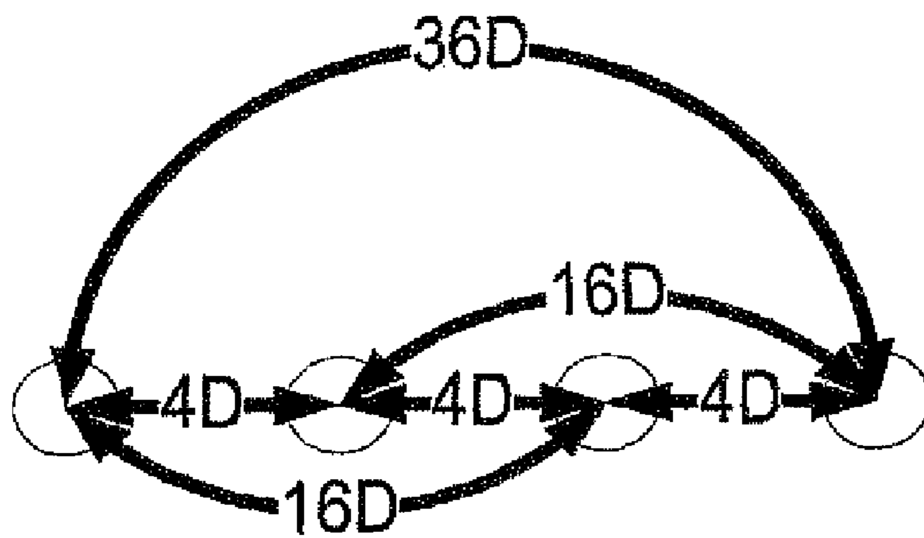
Squared Euclidean distance
