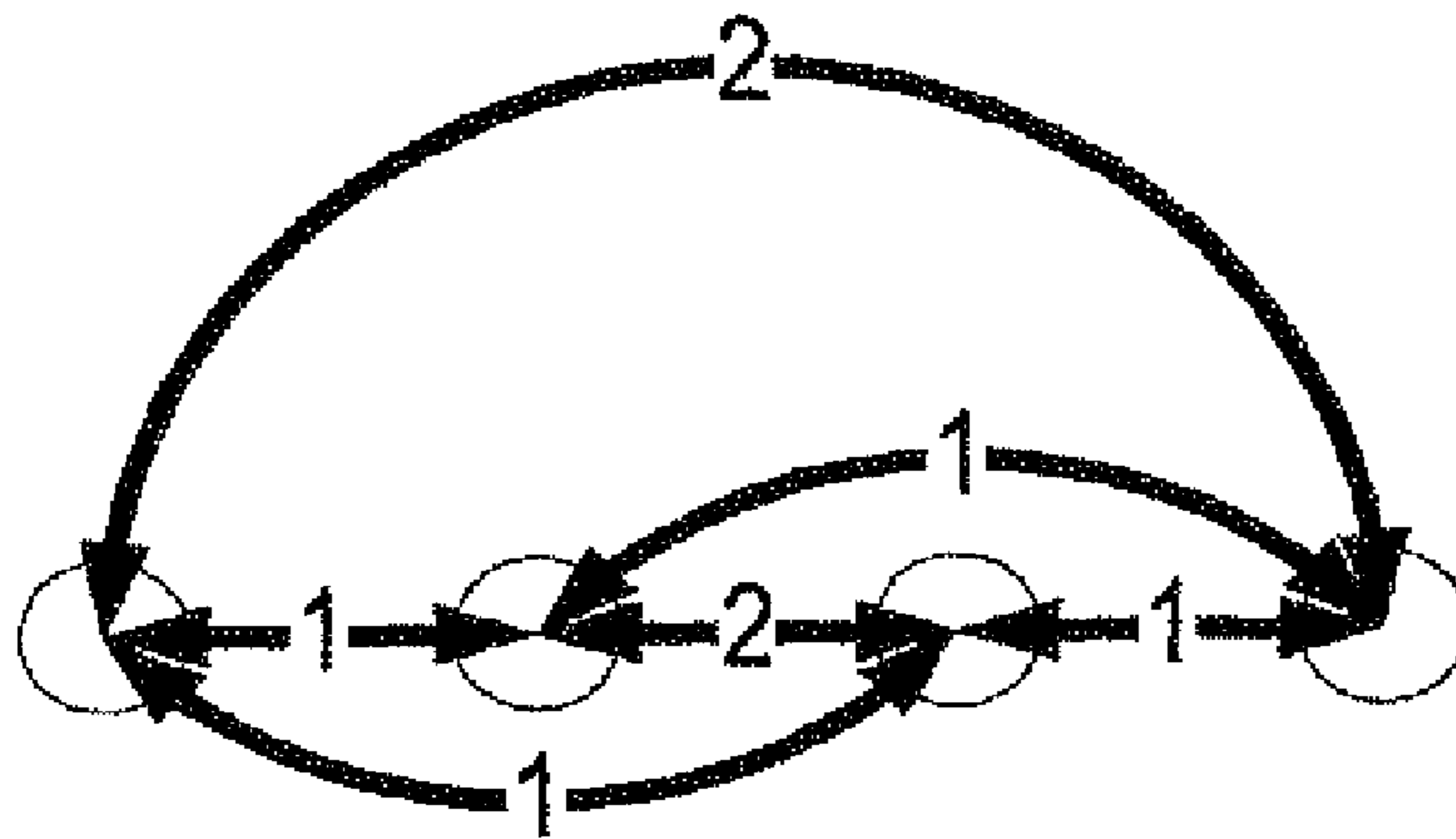
Hamming distance
