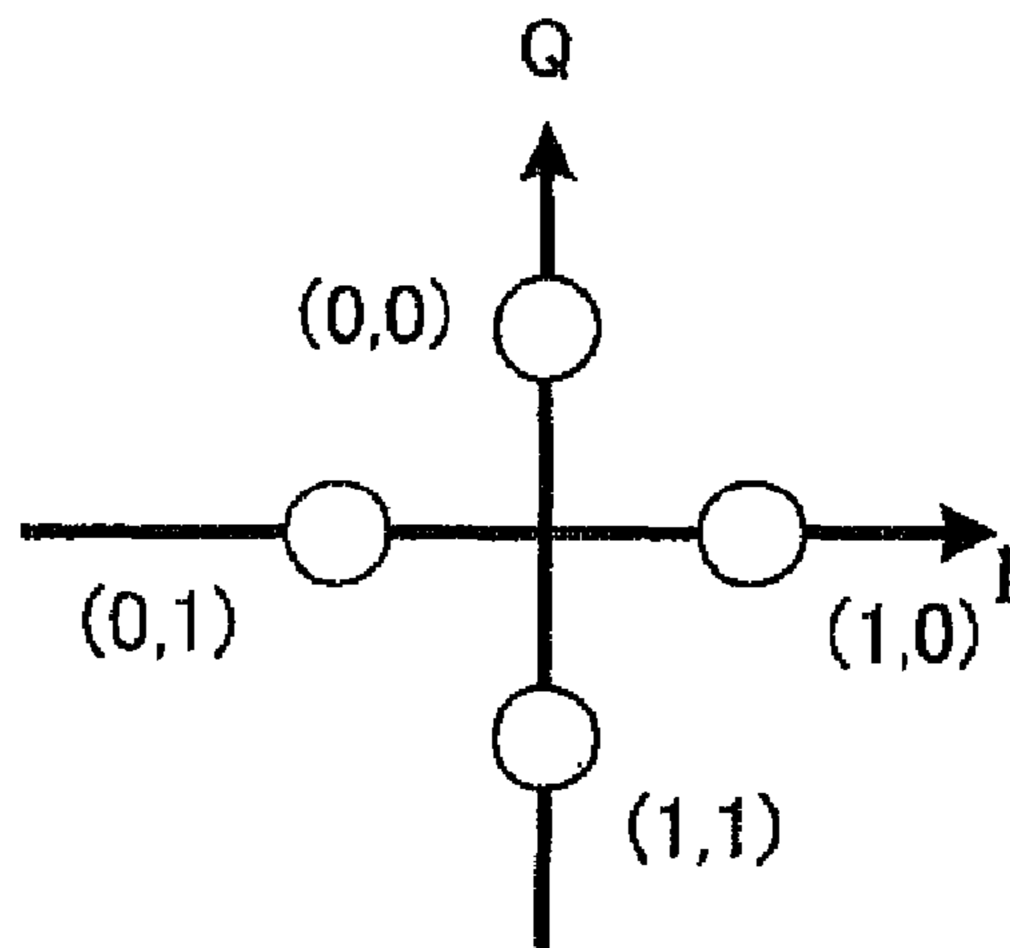
S1(i)'' SIGNAL POINT ARRANGEMENT
