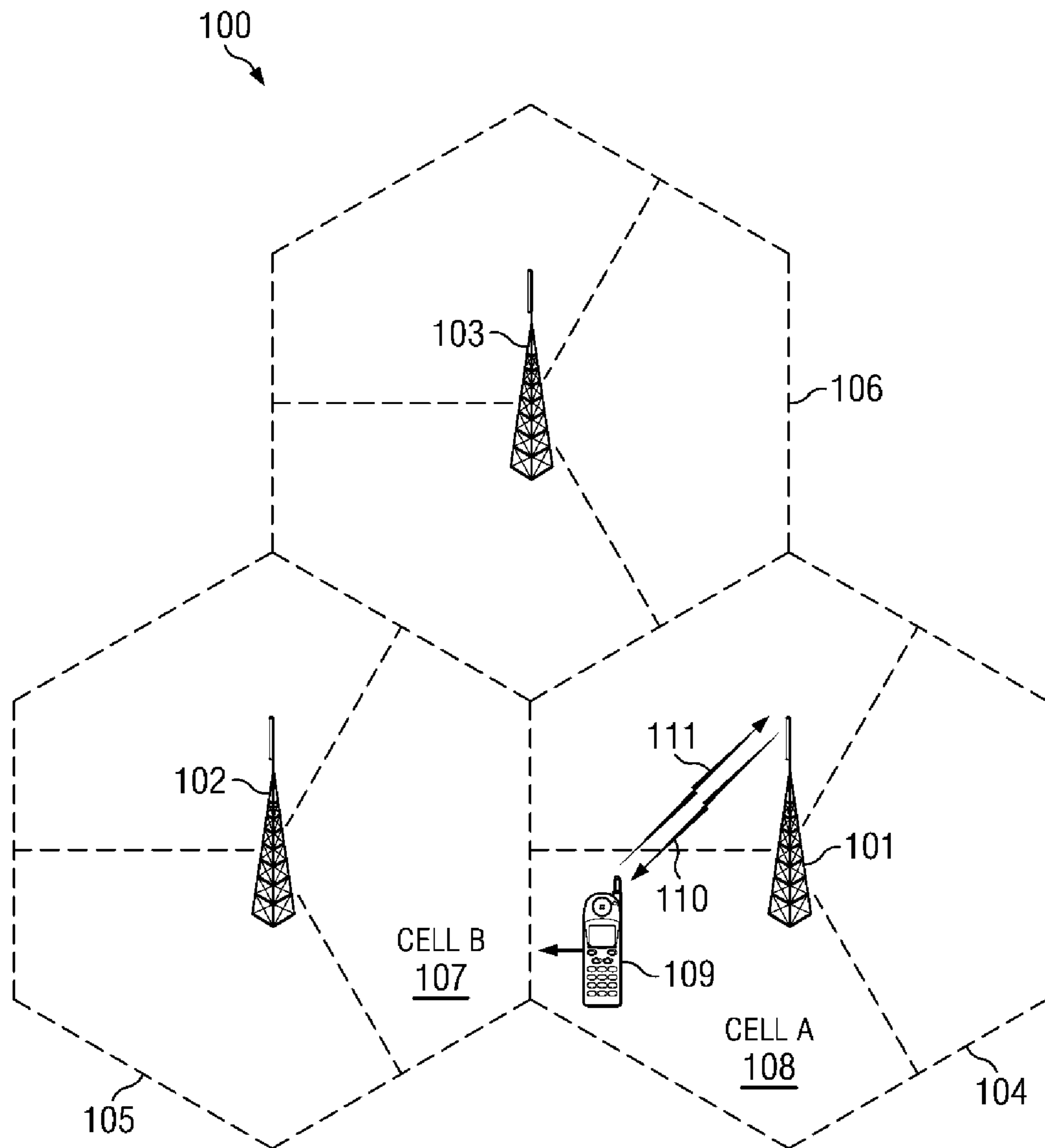
FIG. 1 (PRIOR ART)
