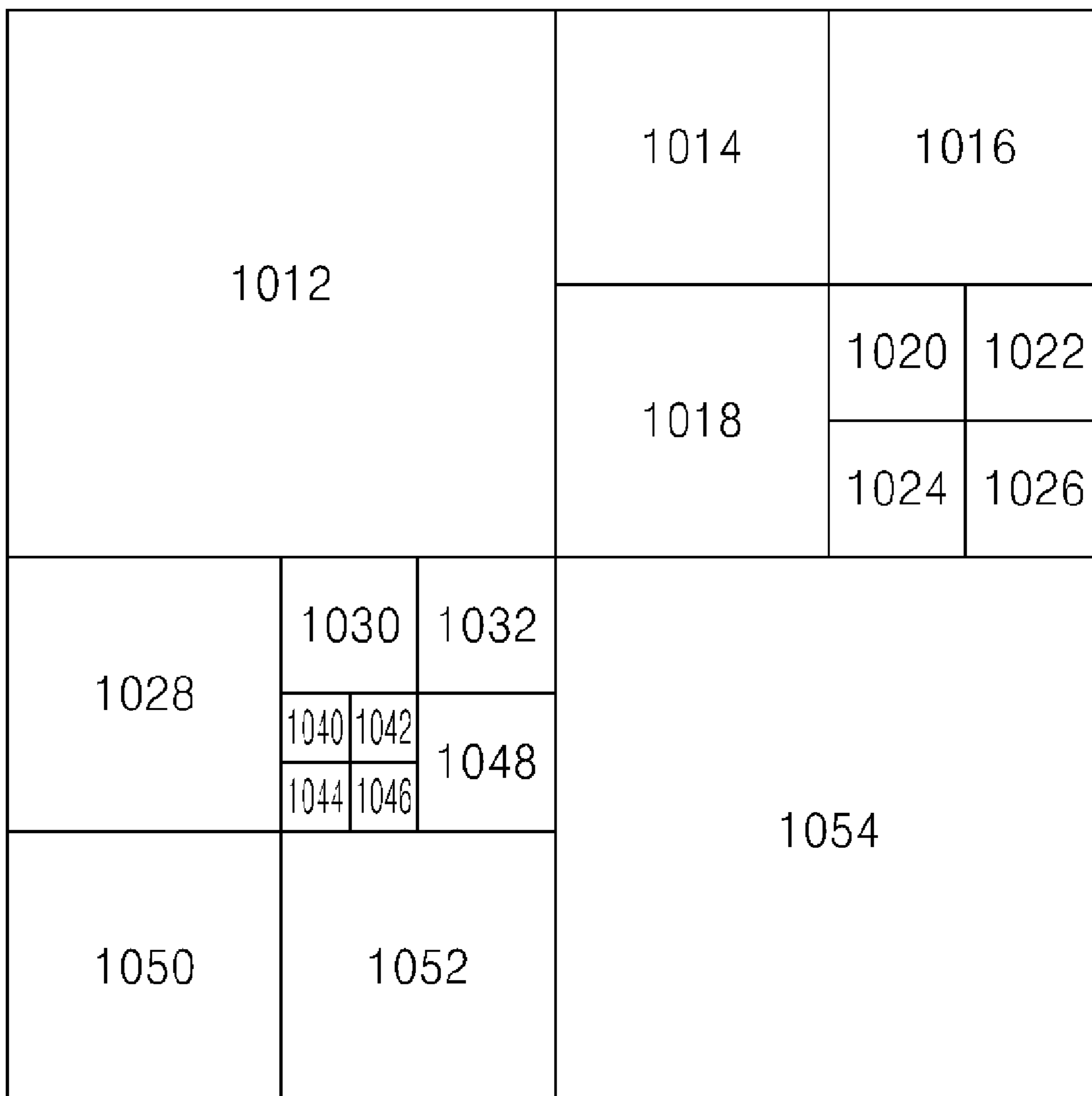
CODING UNITS (1010)
