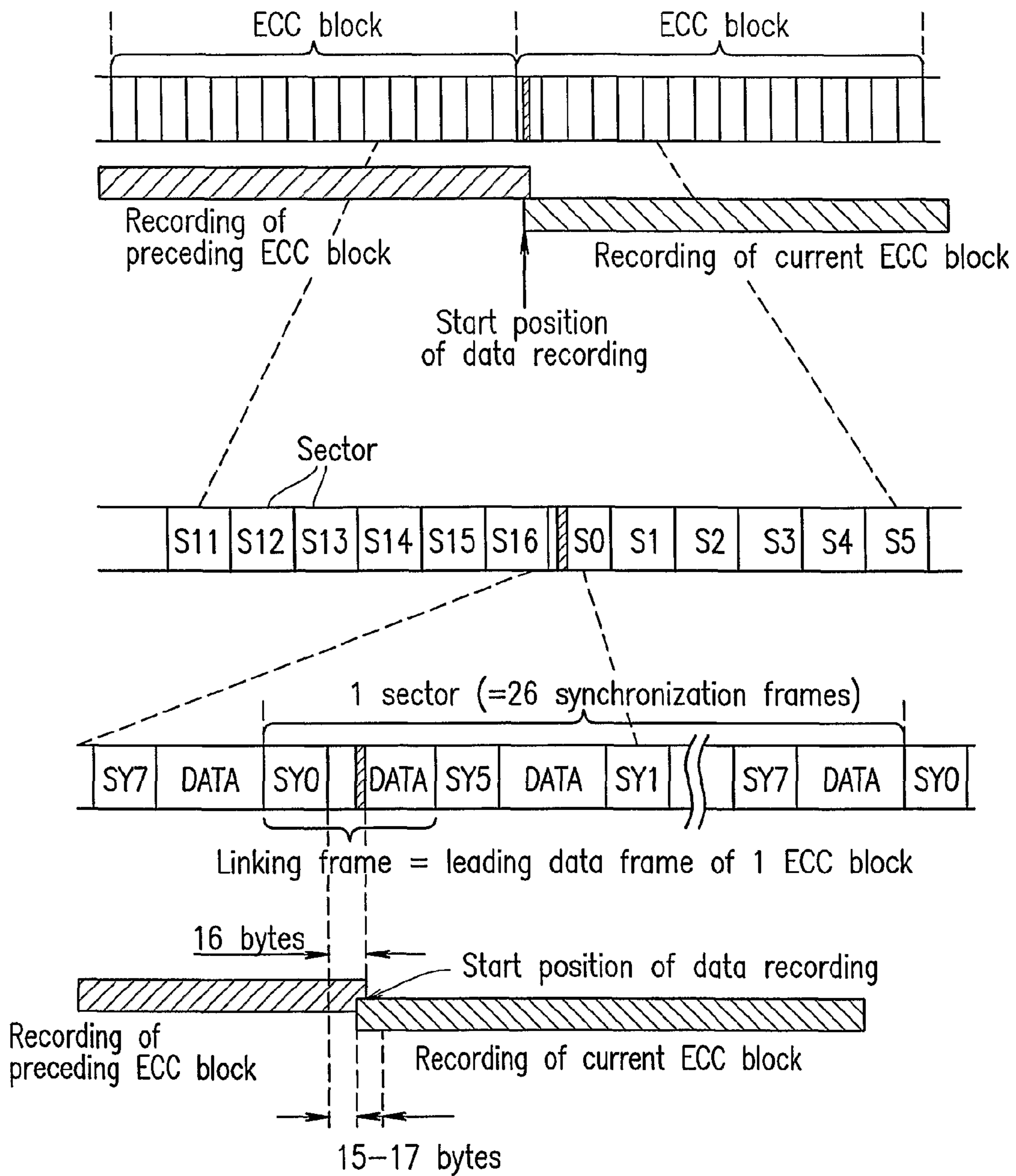
FIG. 44 CONVENTIONAL ART
