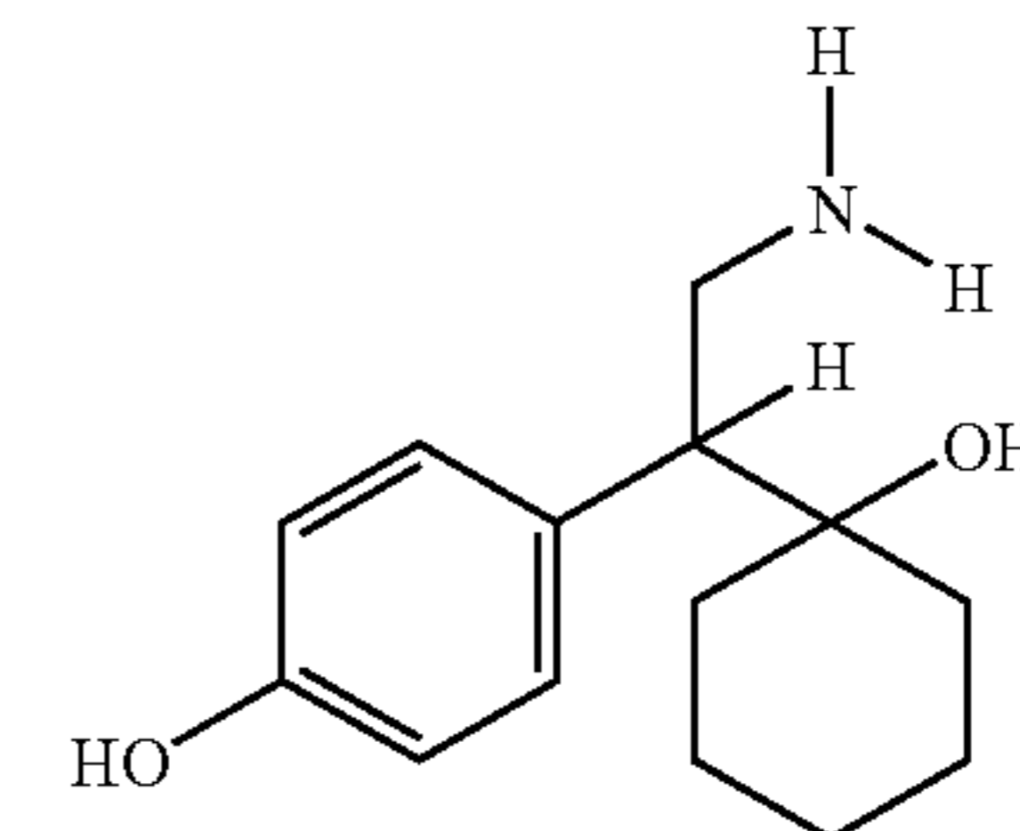
O-desmethyl-N,N-didesmethylvenlafaxine
