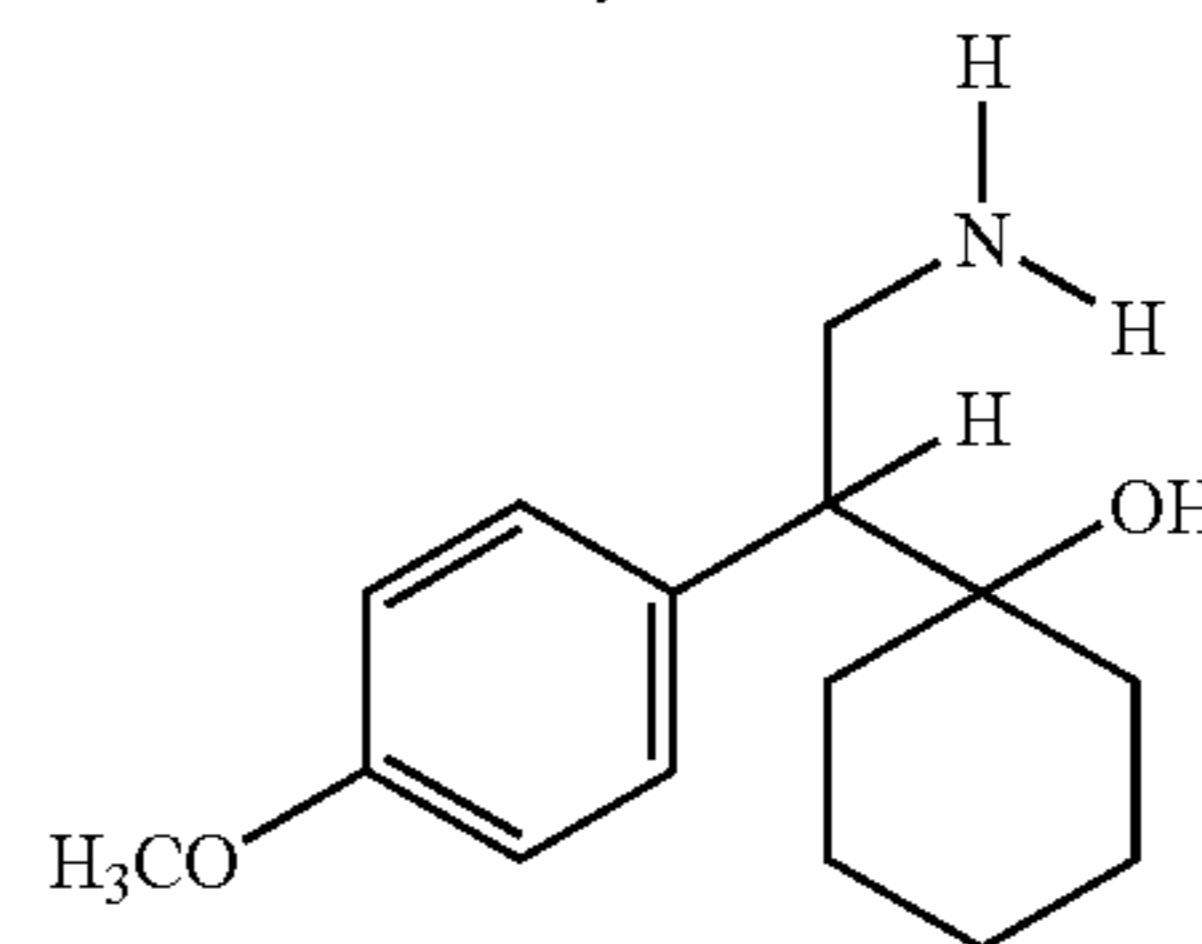
N,N-didesmethylvenlafaxine
