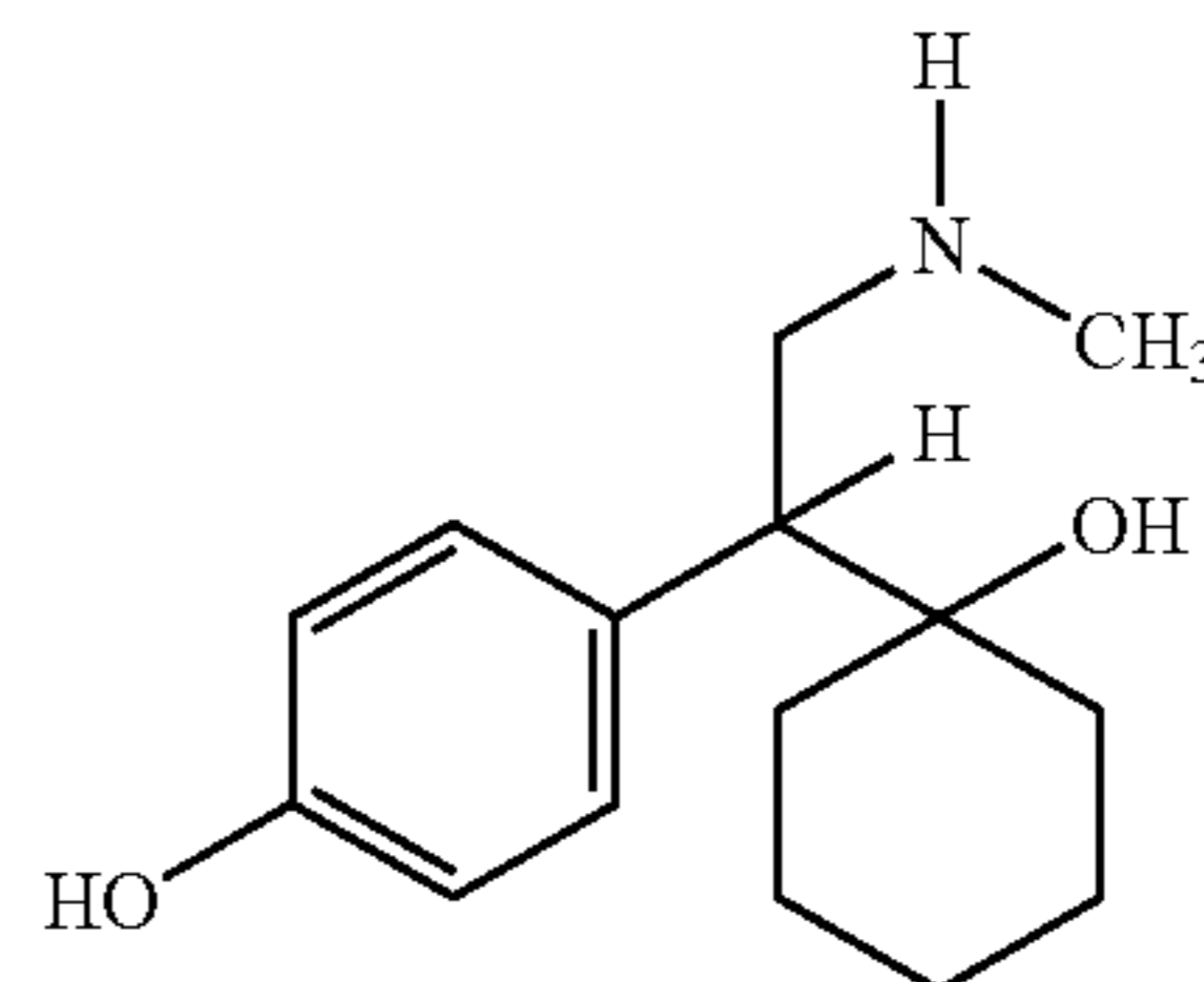
N,O-didesmethylvenlafaxine
