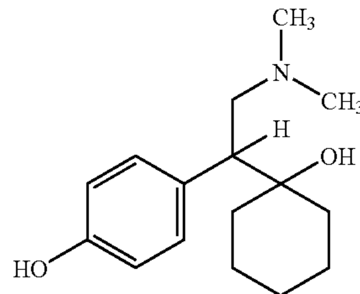
O-desmethylvenlafaxine
