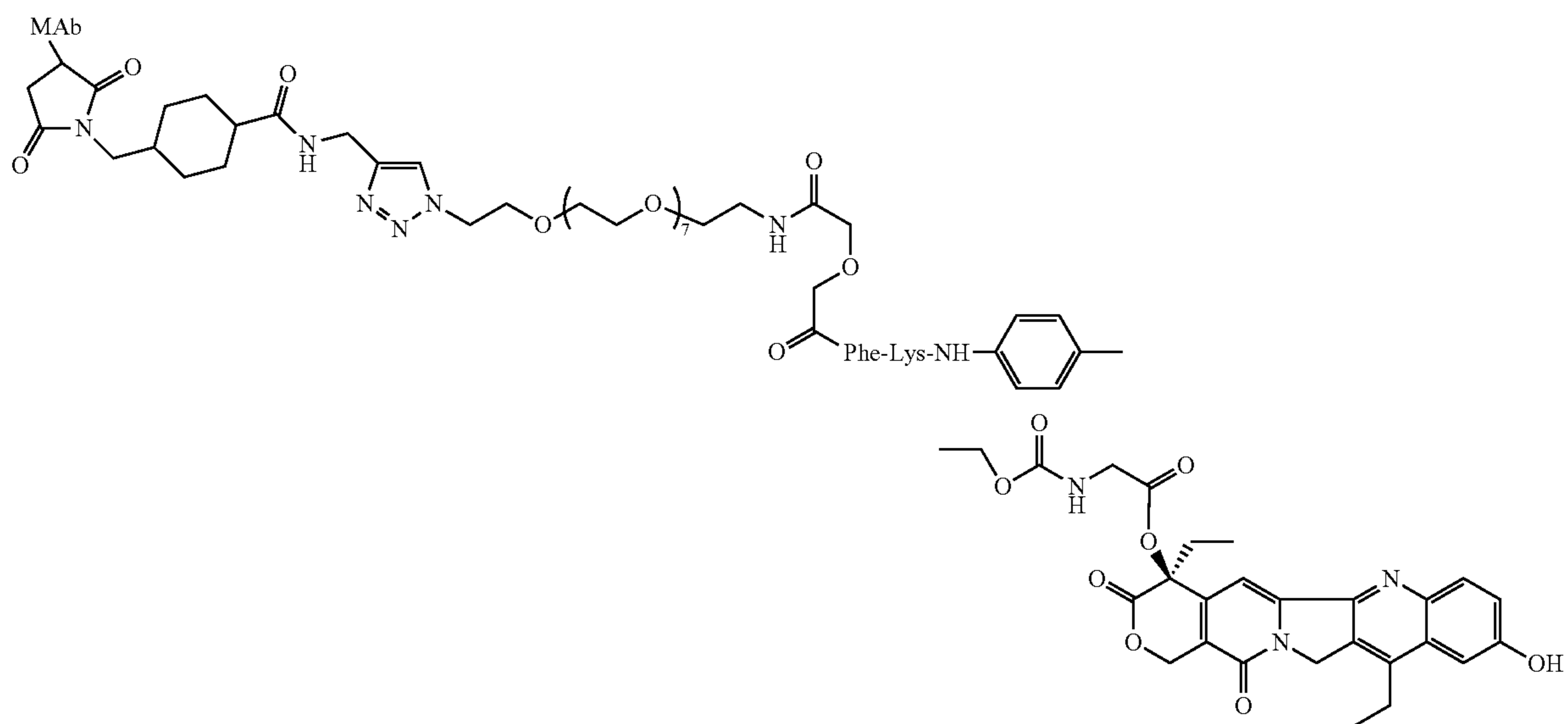
MAb-CL2-SN-38
