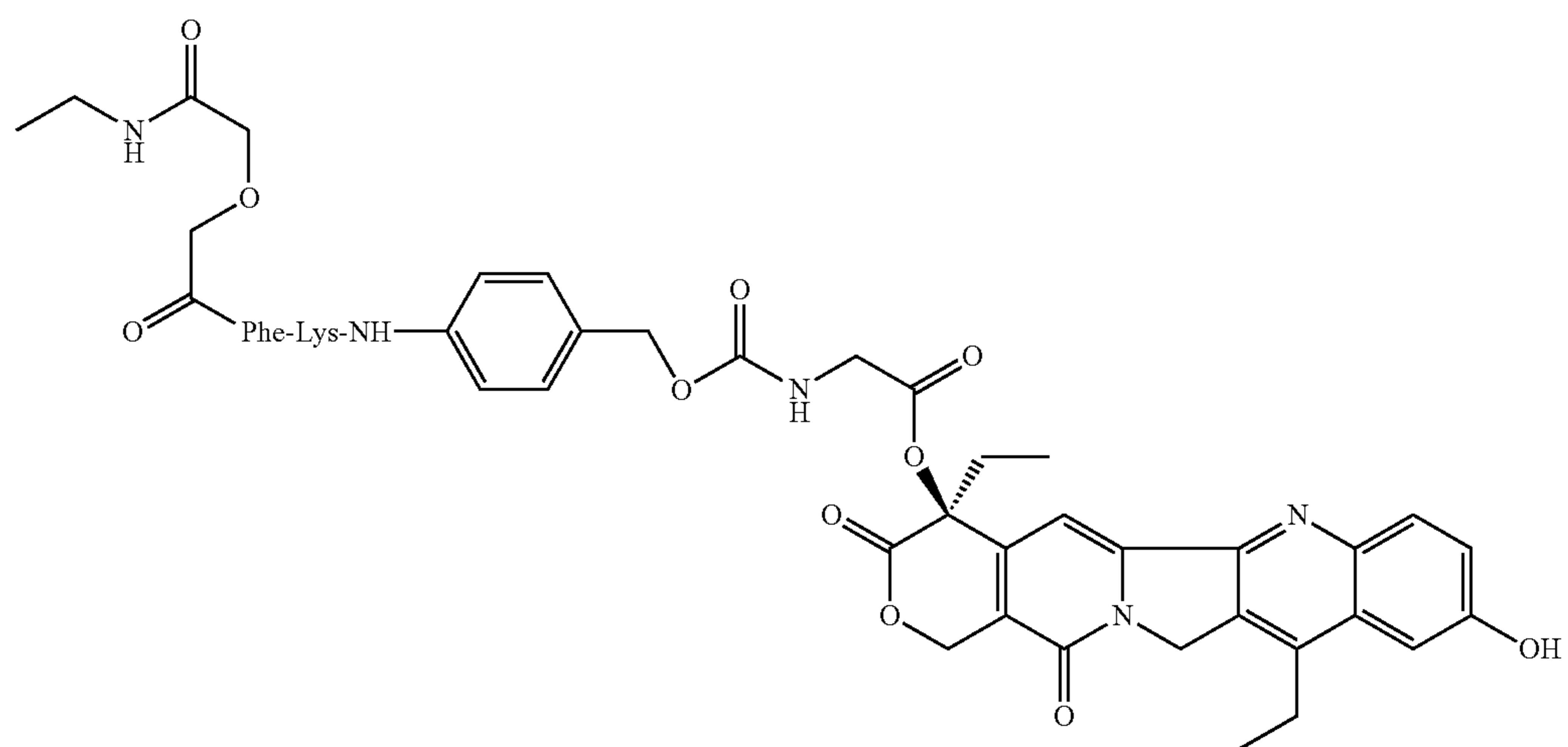
MAb-CL3-SN-38
