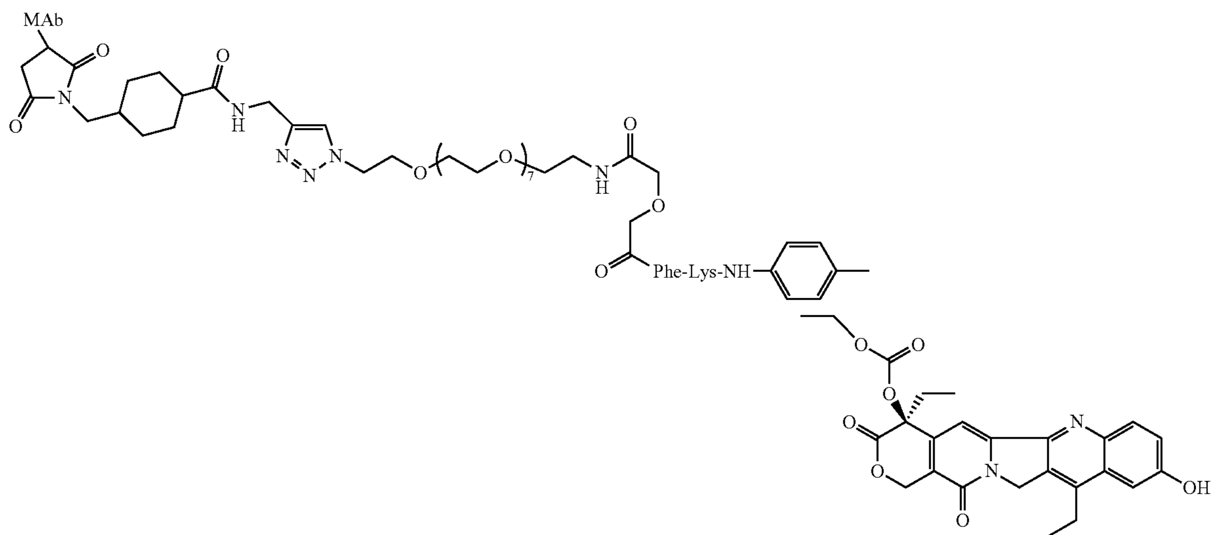
MAb-CL2-SN-38
