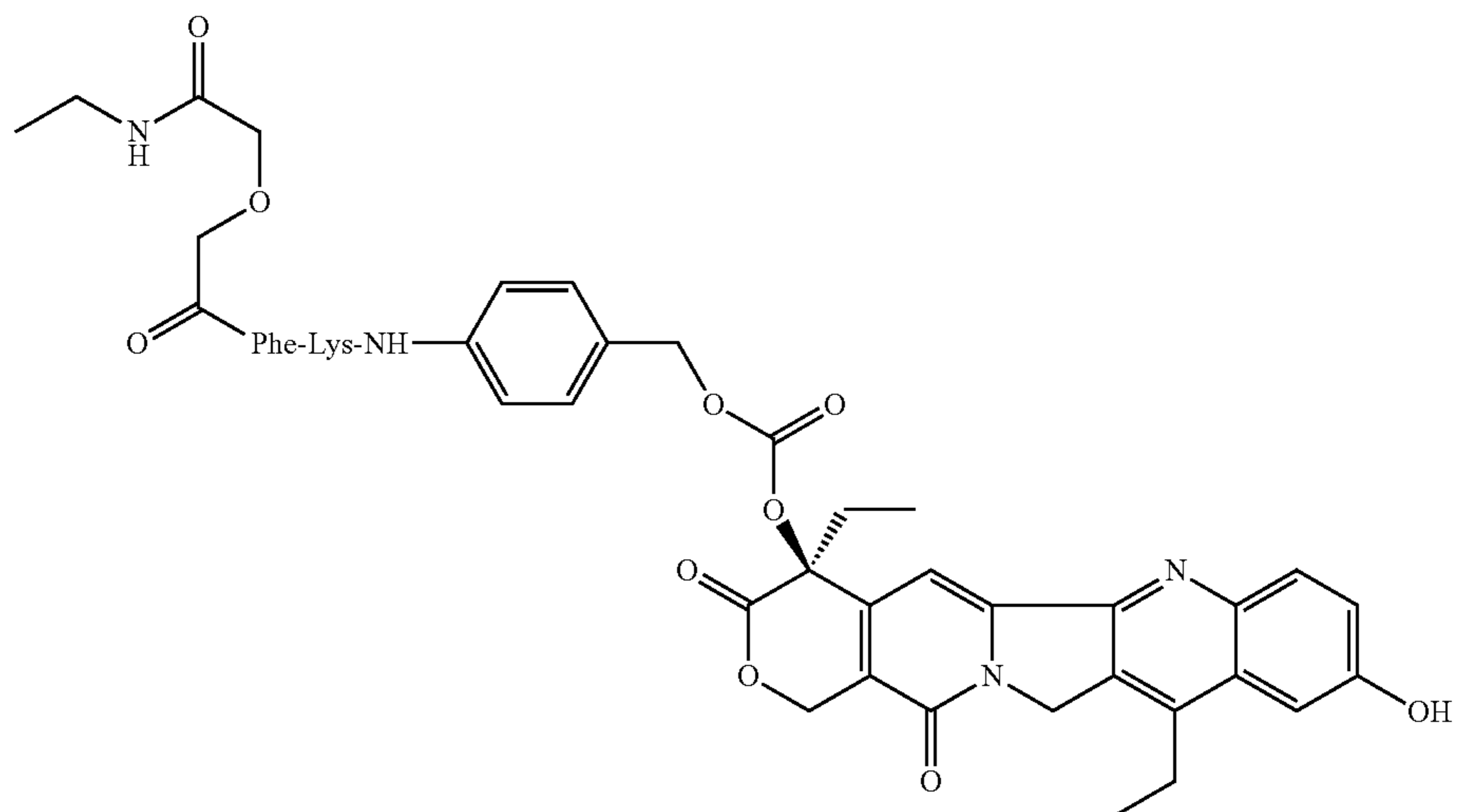
MAb-CL2-SN-38
