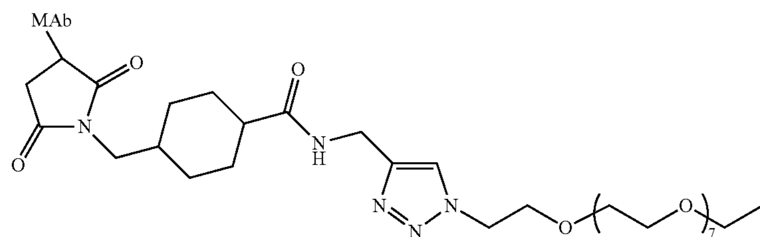
MAb-CL2-SN-38
