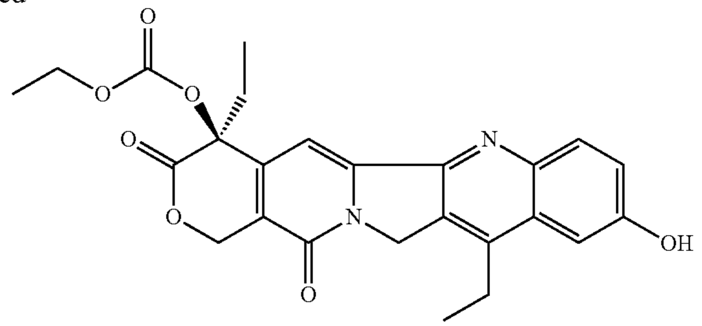
MAb-CL5-SN-38
