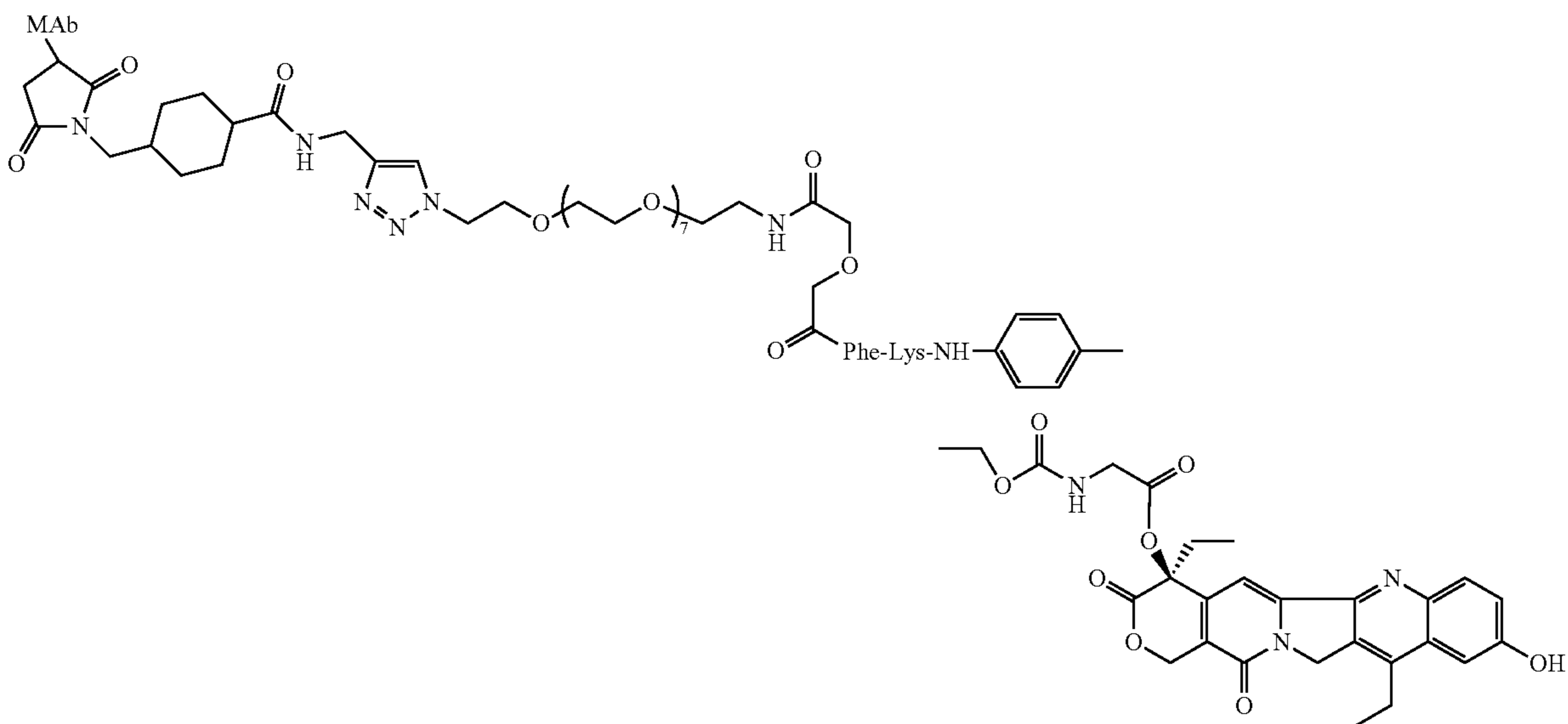
MAb-CL2-SN-38
