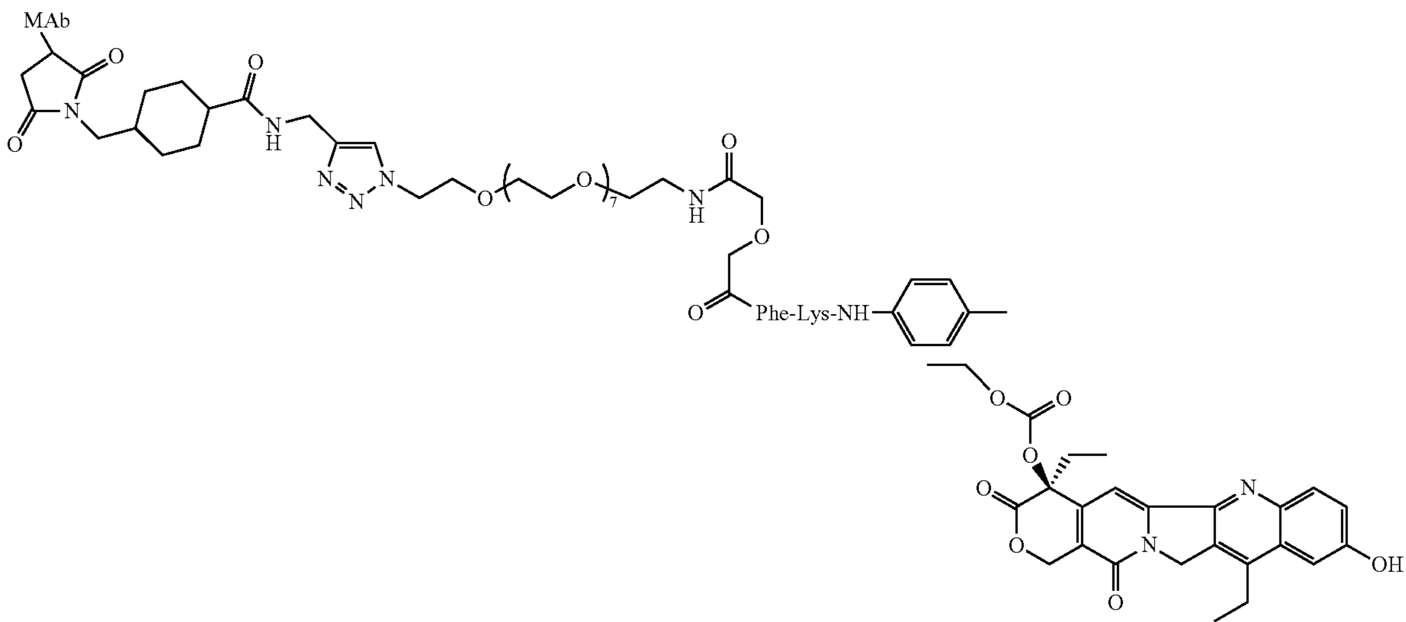
MAb-CL2-SN-38
