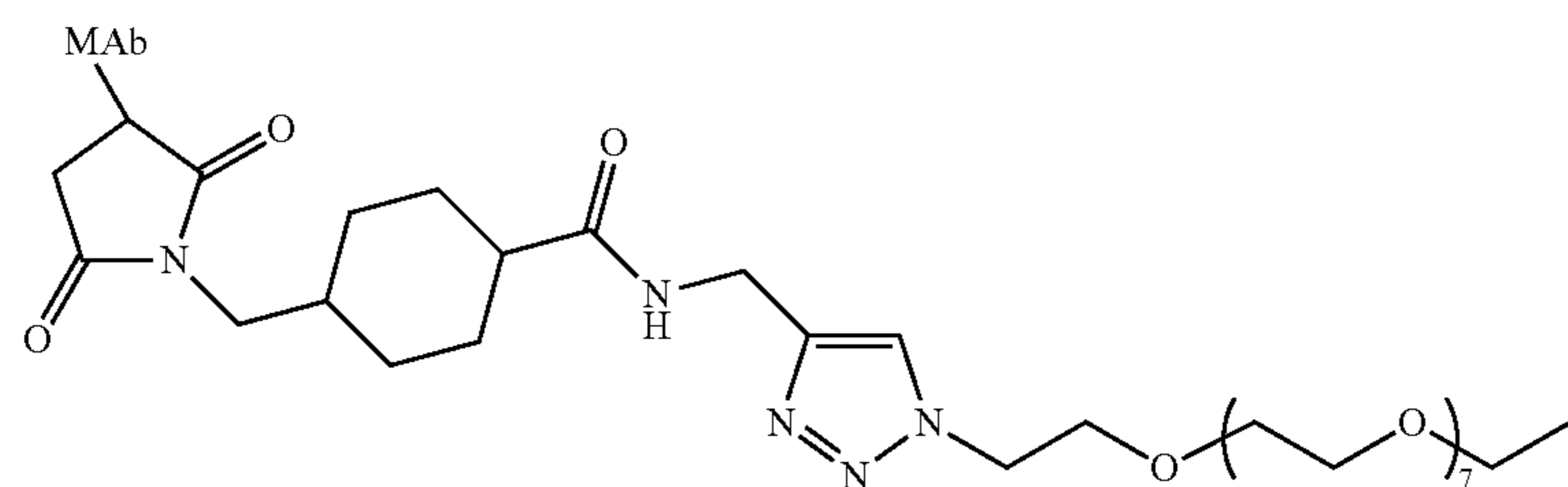
MAb-CL2-SN-38
