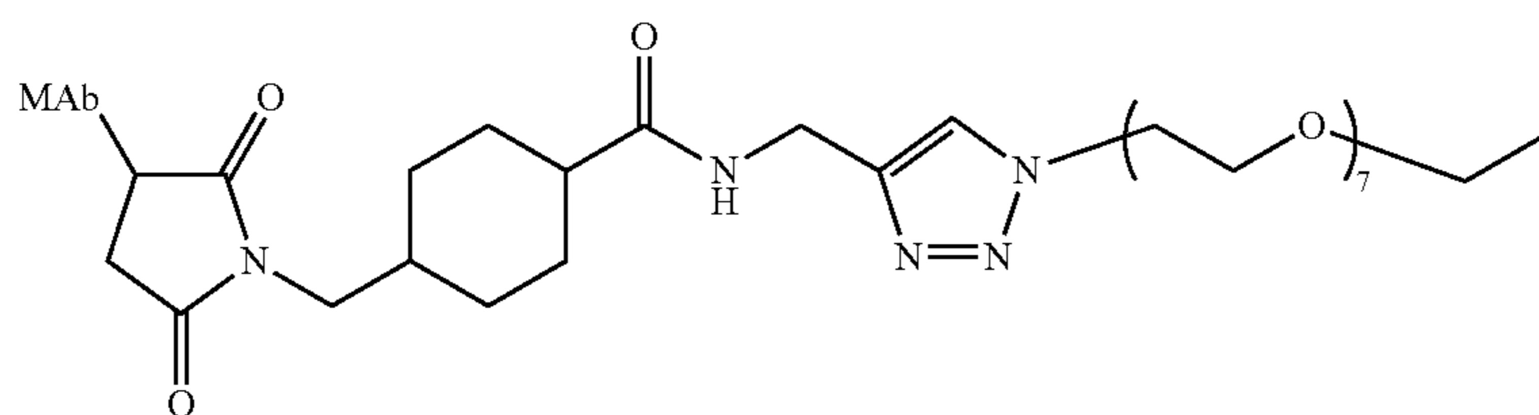
MAb-CL4-SN-38 and
