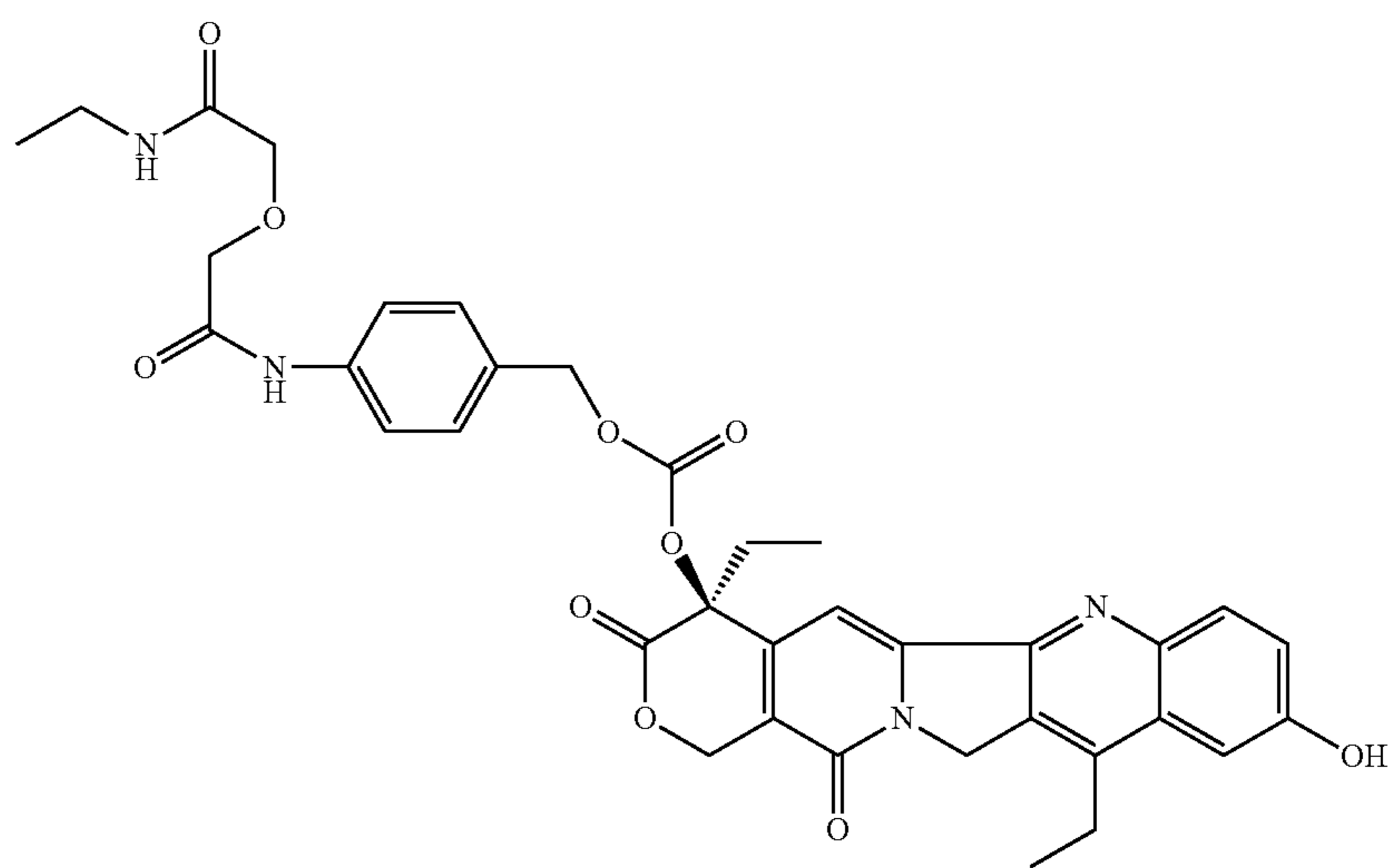
MAb-CL4-SN-38 and
