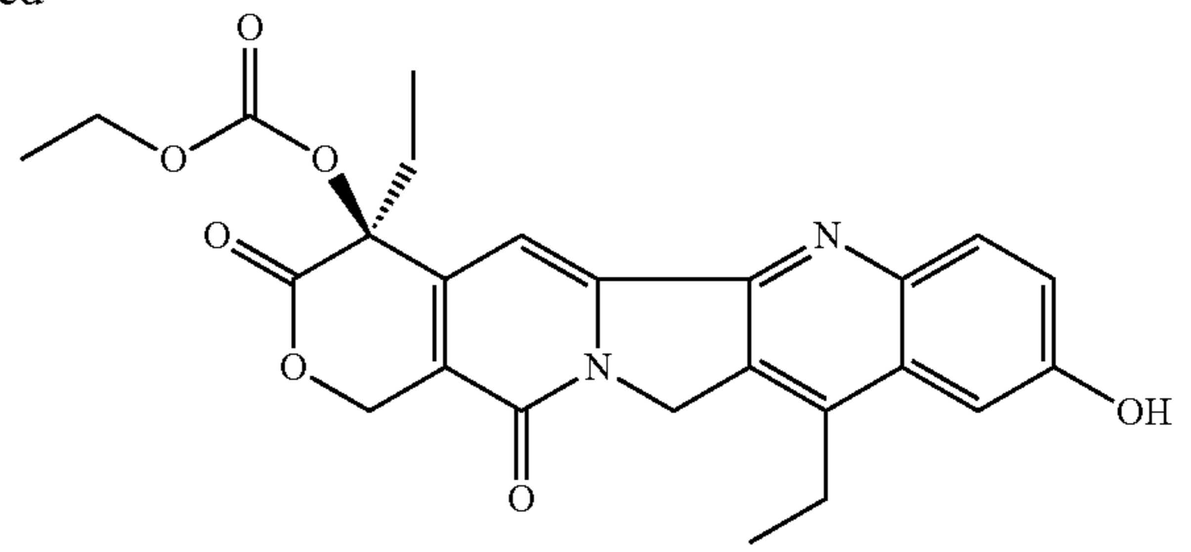
MAb-CL5-SN-38
