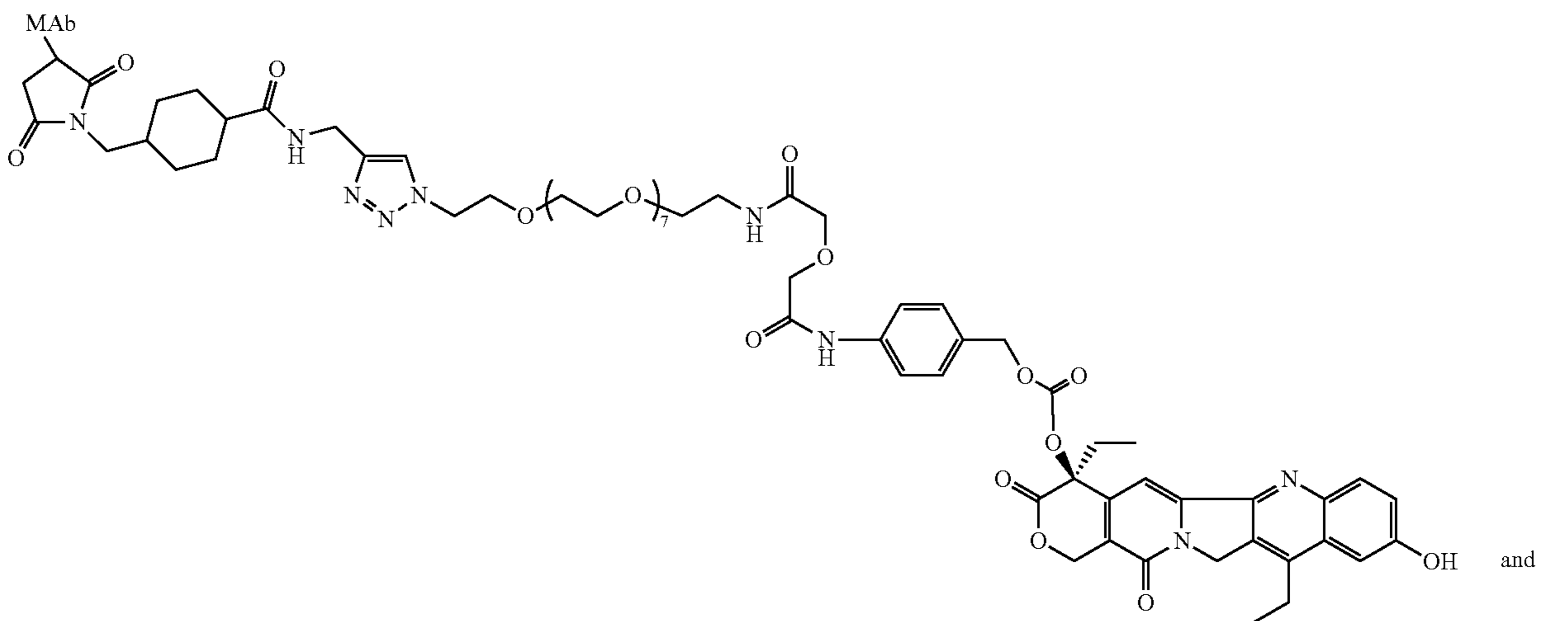
MAb-CL4-SN-38
