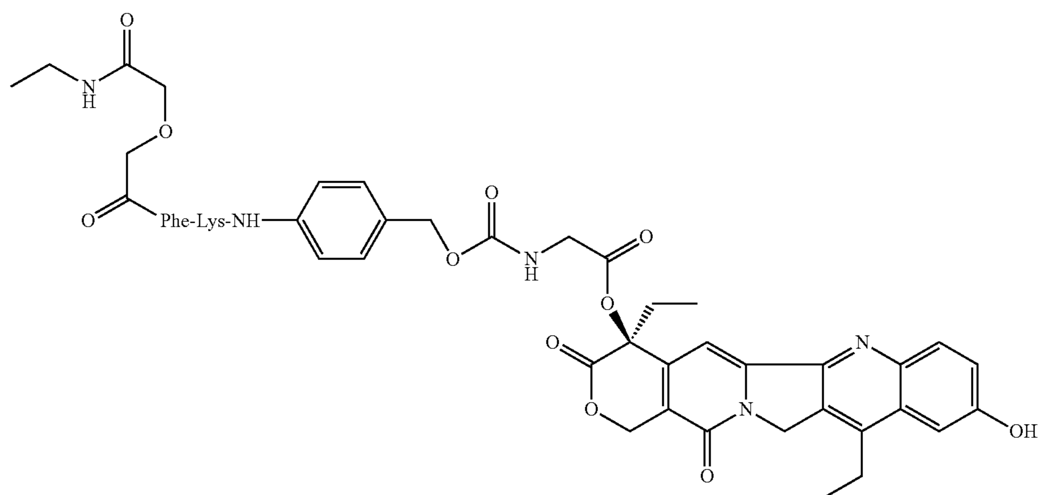
MAb-CL3-SN-38
