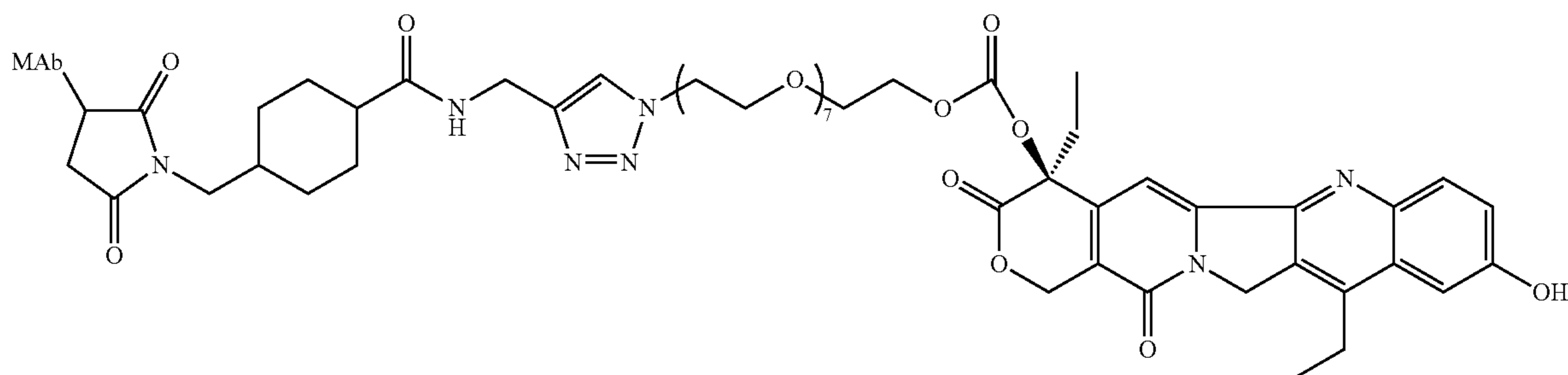
MAb-CL5-SN-38
