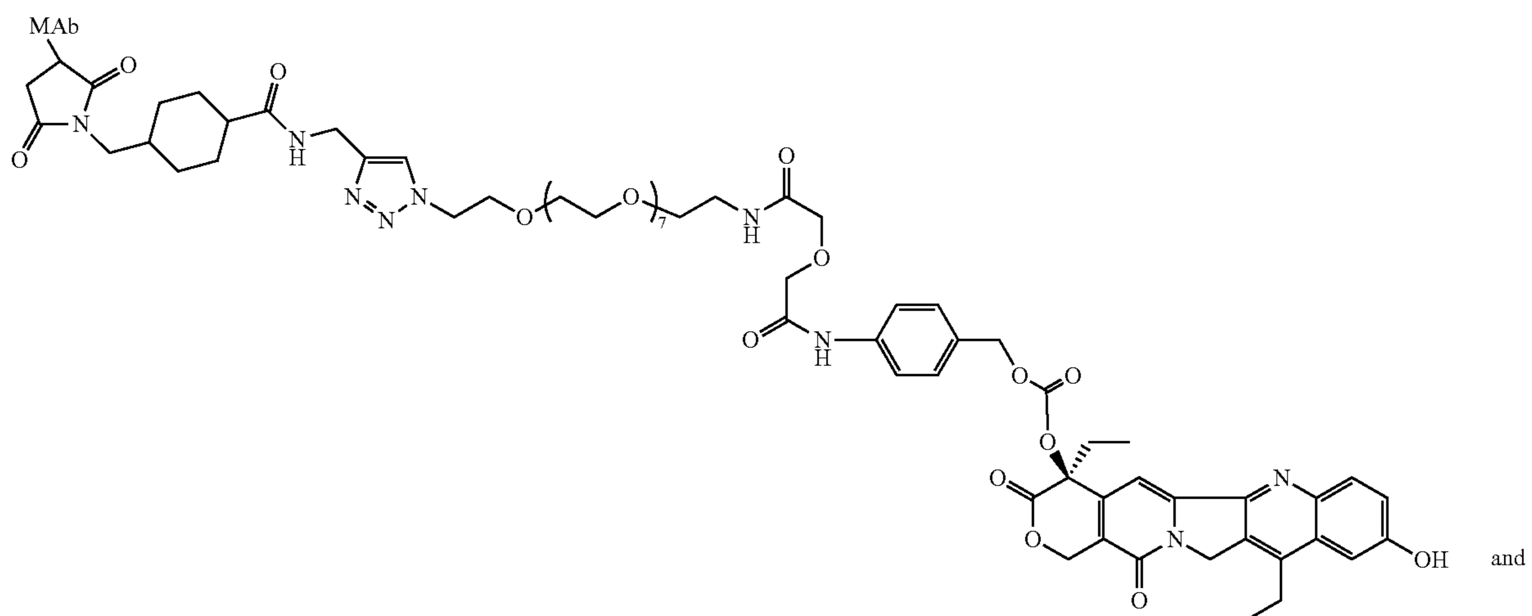
MAb-CL4-SN-38
