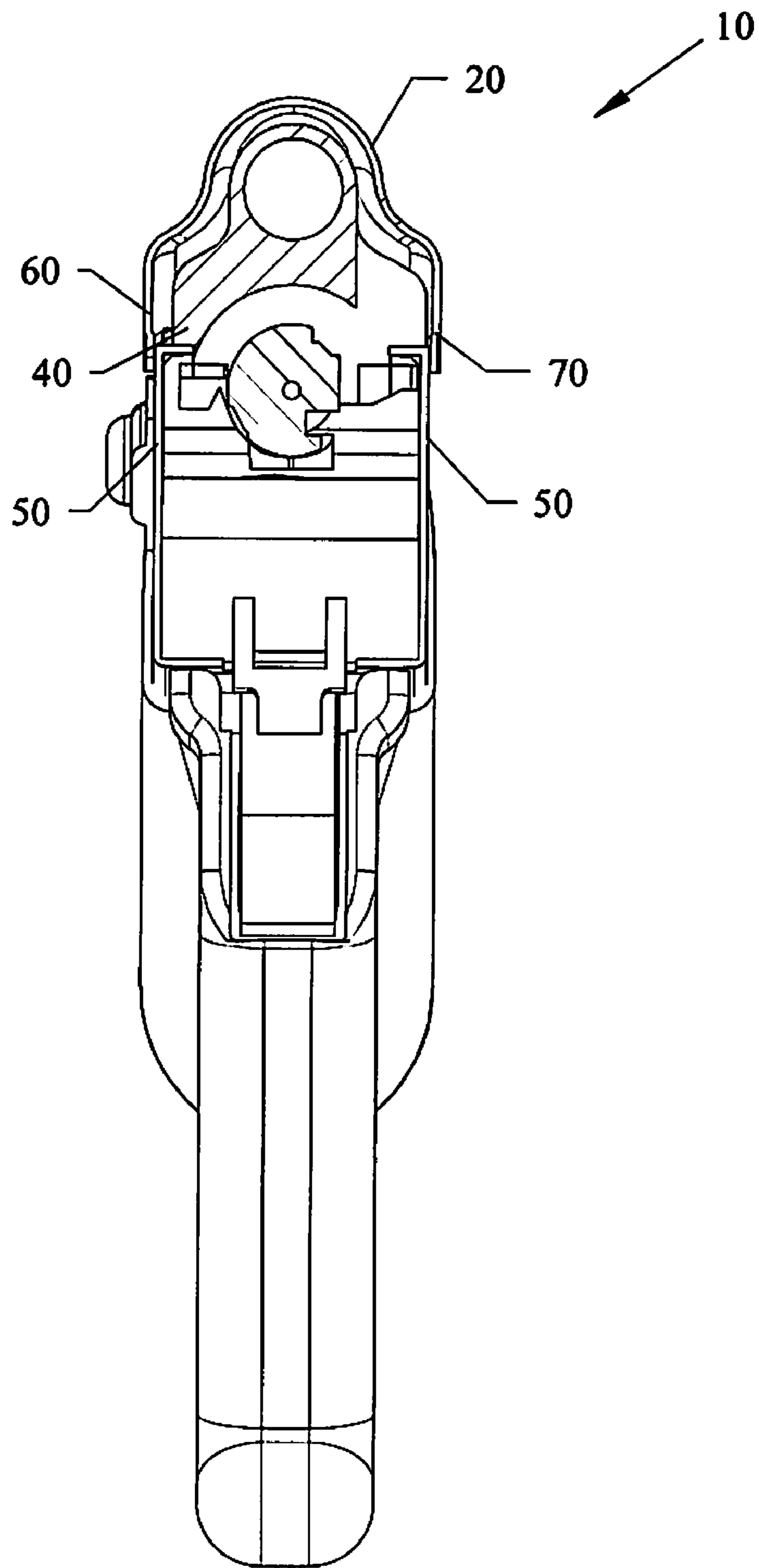
Fig.8 (PRIOR ART)
