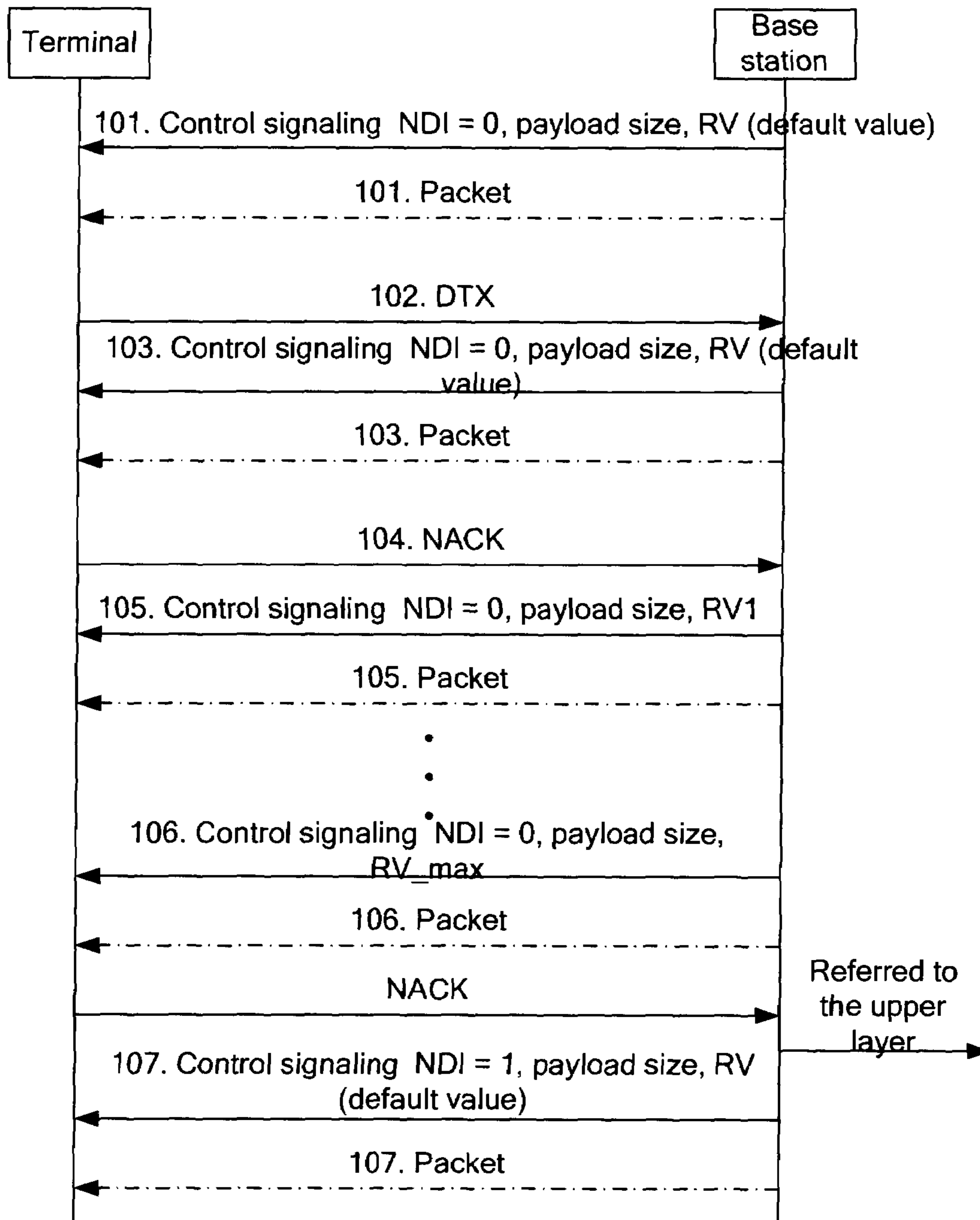
Figure 1 ( Prior Art )
