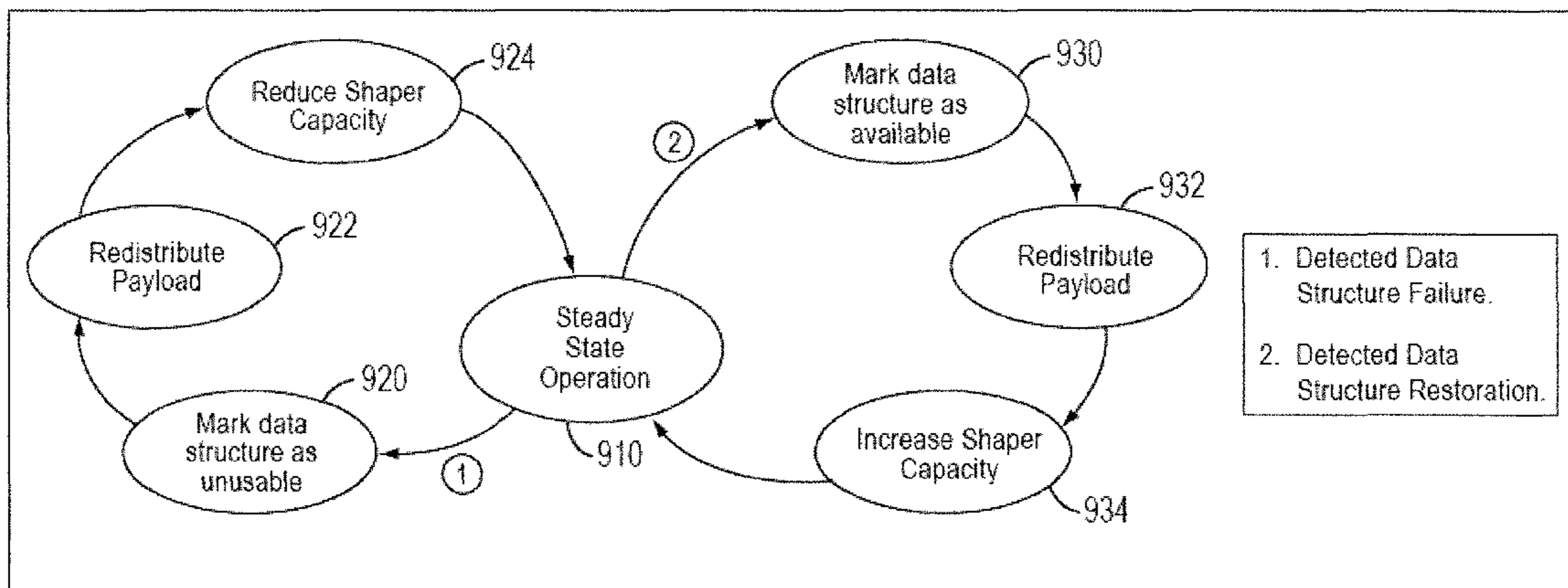
Link Aggregation Payload Redistribution State Diagram
