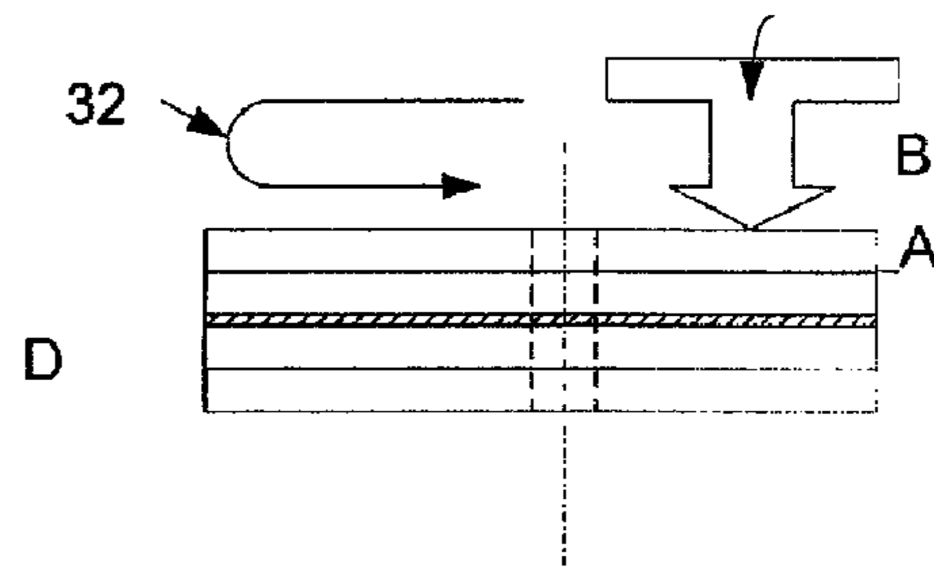
FIG. 1C PRIOR ART
